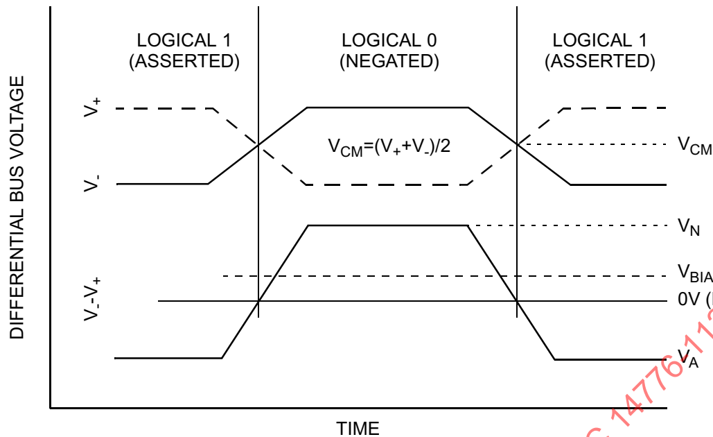
Figure 42 - Signaling sense
