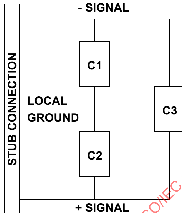
Figure 33 - Capacitive loads
