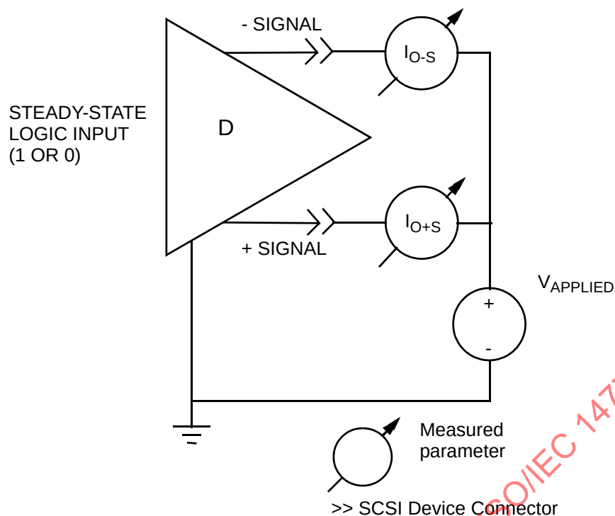
Figure A.6 - Driver short-circuit test circuit
