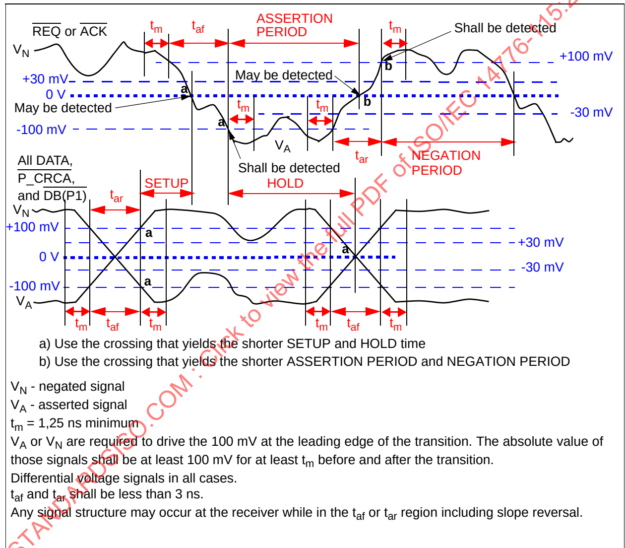
Figure 60 - LVD timing measurement points for ST synchronous transfers
