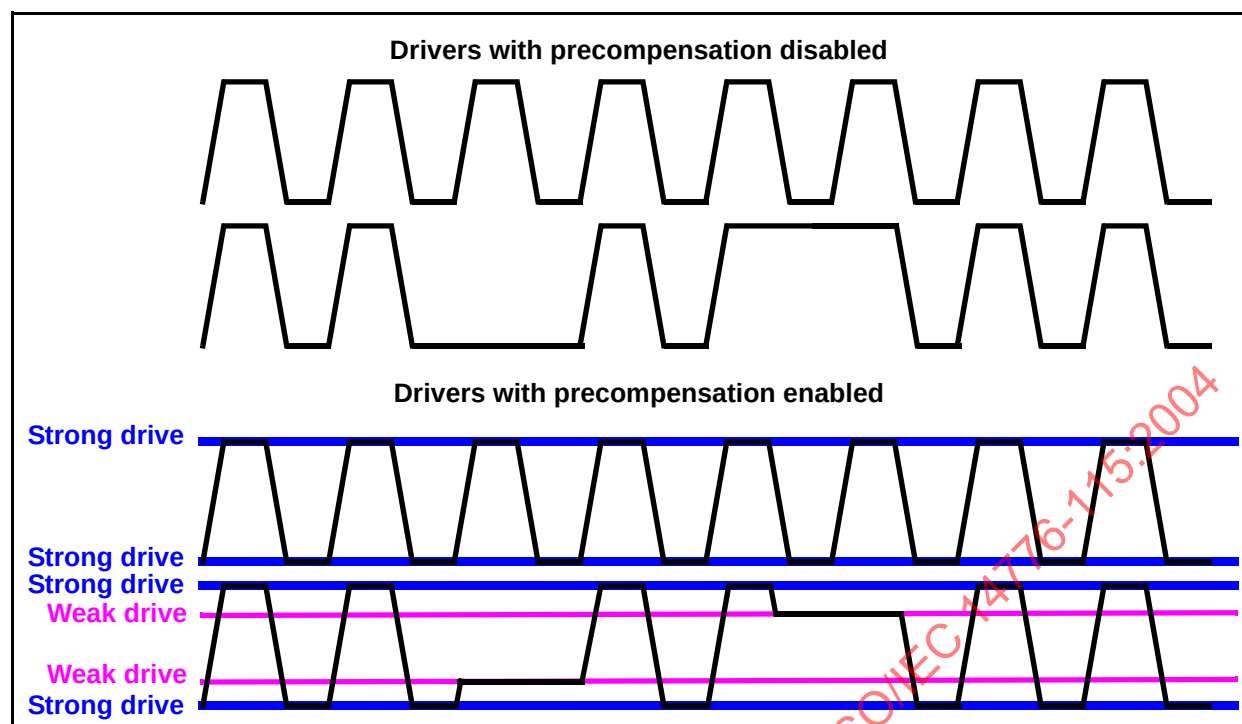
Figure 46 - Examples of fast-160 driver precompensation
