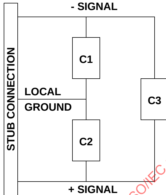
Figure 49 - LVD Capacitive loads
