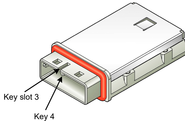
Figure 56 – Mini SAS 4x receptacle connector - end device or enclosure universal port for trained 1.5 Gbit/s, 3 Gbit/s, and 6 Gbit/s and for untrained 1.5 Gbit/s and 3 Gbit/s
