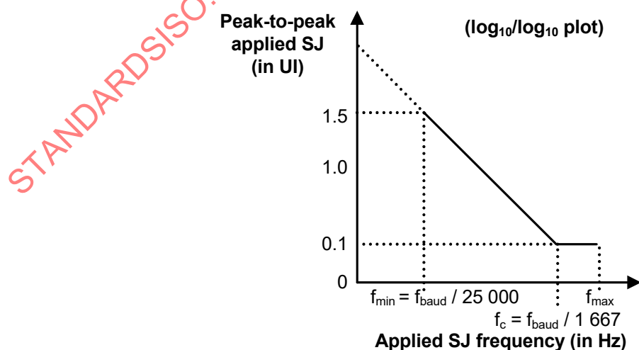
Figure 139 – Applied SJ for untrained 1.5 Gbit/s and 3 Gbit/s
