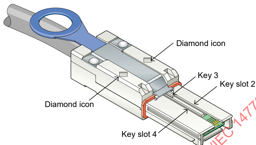
Figure 47 – Mini SAS 4x cable plug connector for trained 1.5 Gbit/s, 3 Gbit/s, and 6 Gbit/s that attaches to an enclosure out port
