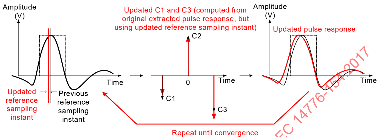
Figure 120 – Convergence of reference transmitter equalization
