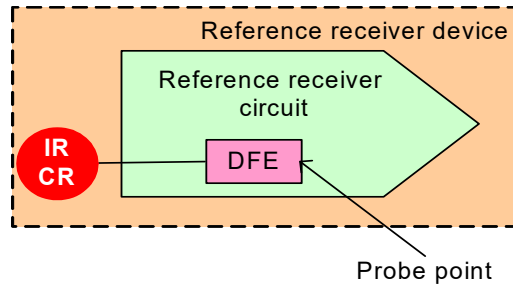
Figure 141 – Reference receiver device for trained 1.5 Gbit/s, 3 Gbit/s, and 6 Gbit/s
