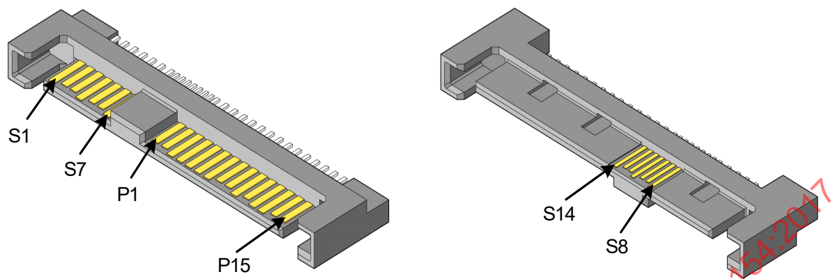
Figure 24 – SAS Drive plug connector
