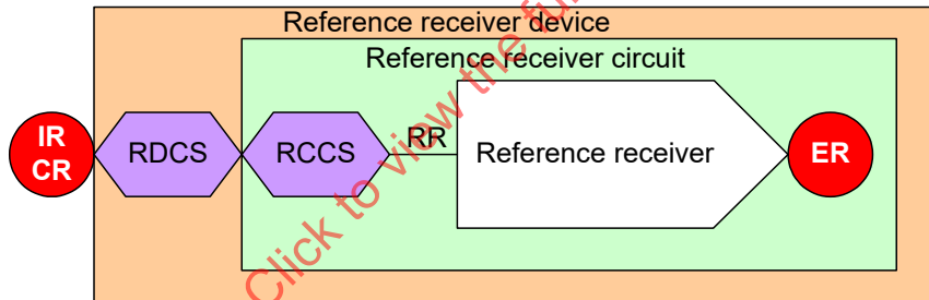
Figure 142 – Reference receiver device for trained 12 Gbit/s
