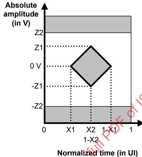
Figure 124 – Receiver device eye mask
