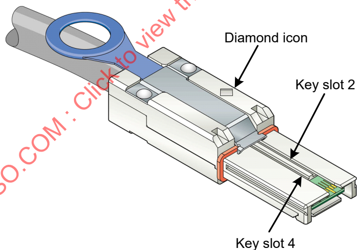
Figure 44 – Mini SAS 4x cable plug connector for untrained 1.5 Gbit/s and 3 Gbit/s that attaches to an enclosure out port
