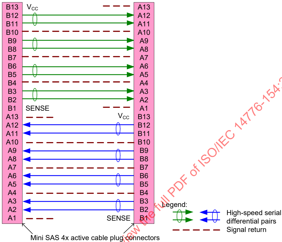
Figure 87 – Mini SAS 4x active external cable assembly
