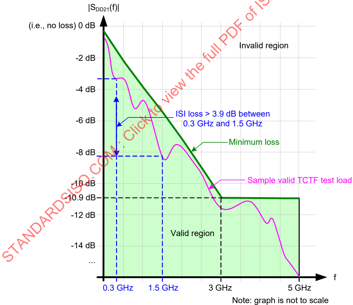
Figure 107 – TCTF test load |S_{DD21}(f)| and ISI loss requirements at IT for untrained 3 Gbit/s
