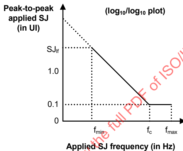
Figure 149 – Applied SJ for trained 1.5 Gbit/s, 3 Gbit/s, 6 Gbit/s and 12 Gbit/s with SSC support
