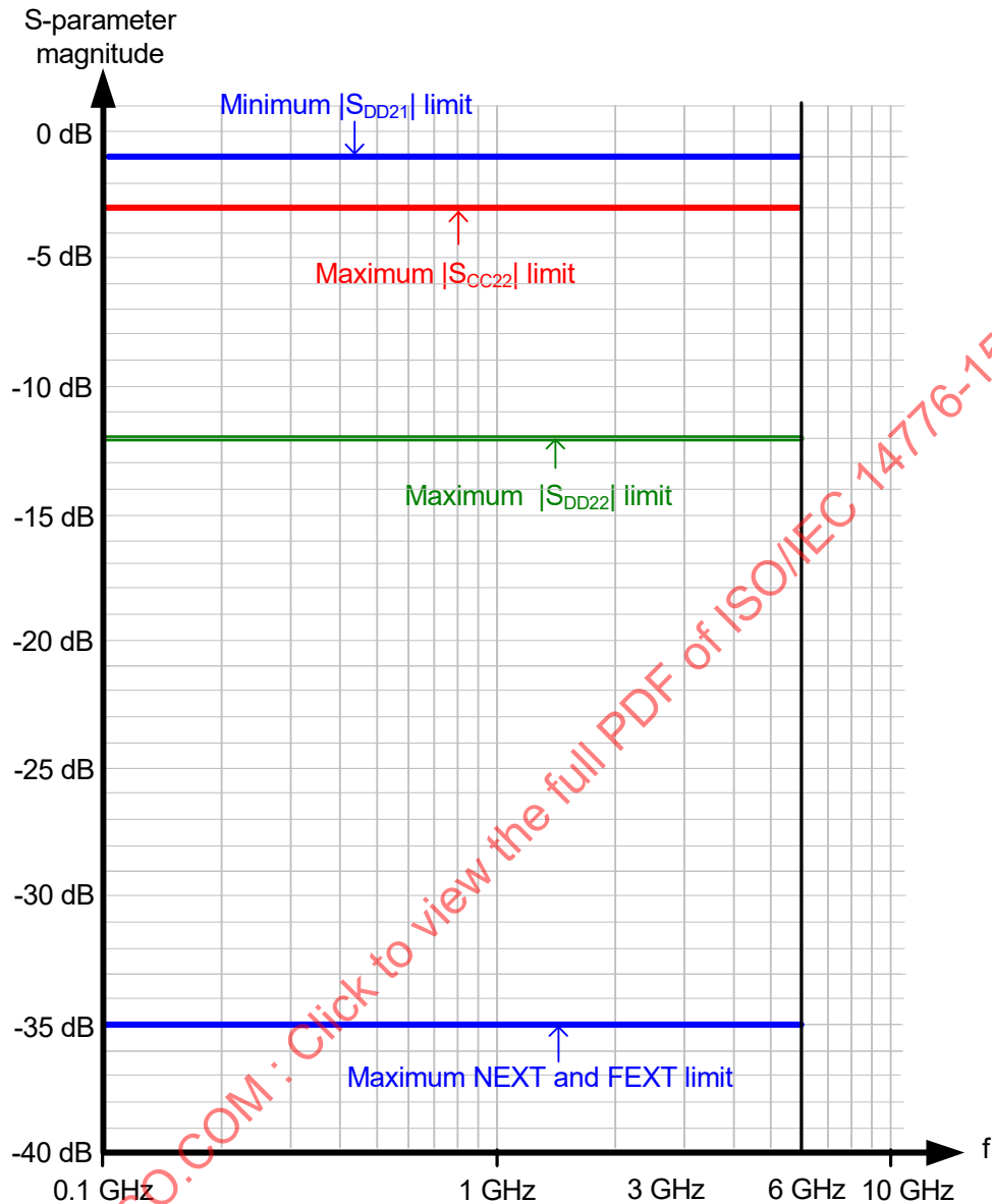
Figure 23 – Recommended |S_{DD21}| , |S_{CC22}| , |S_{DD22}| , NEXT, and FEXT limits for connector mated pairs supporting rates of 12 Gbit/s
