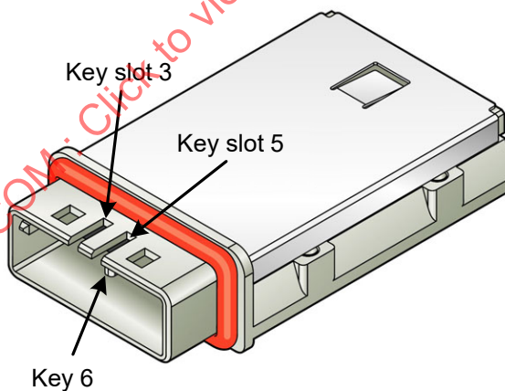
Figure 61 – Mini SAS 4x active receptacle connector - enclosure in port
