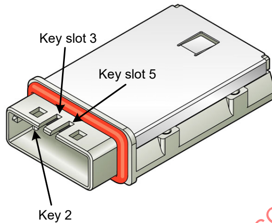
Figure 60 – Mini SAS 4x active receptacle connector - enclosure out port
