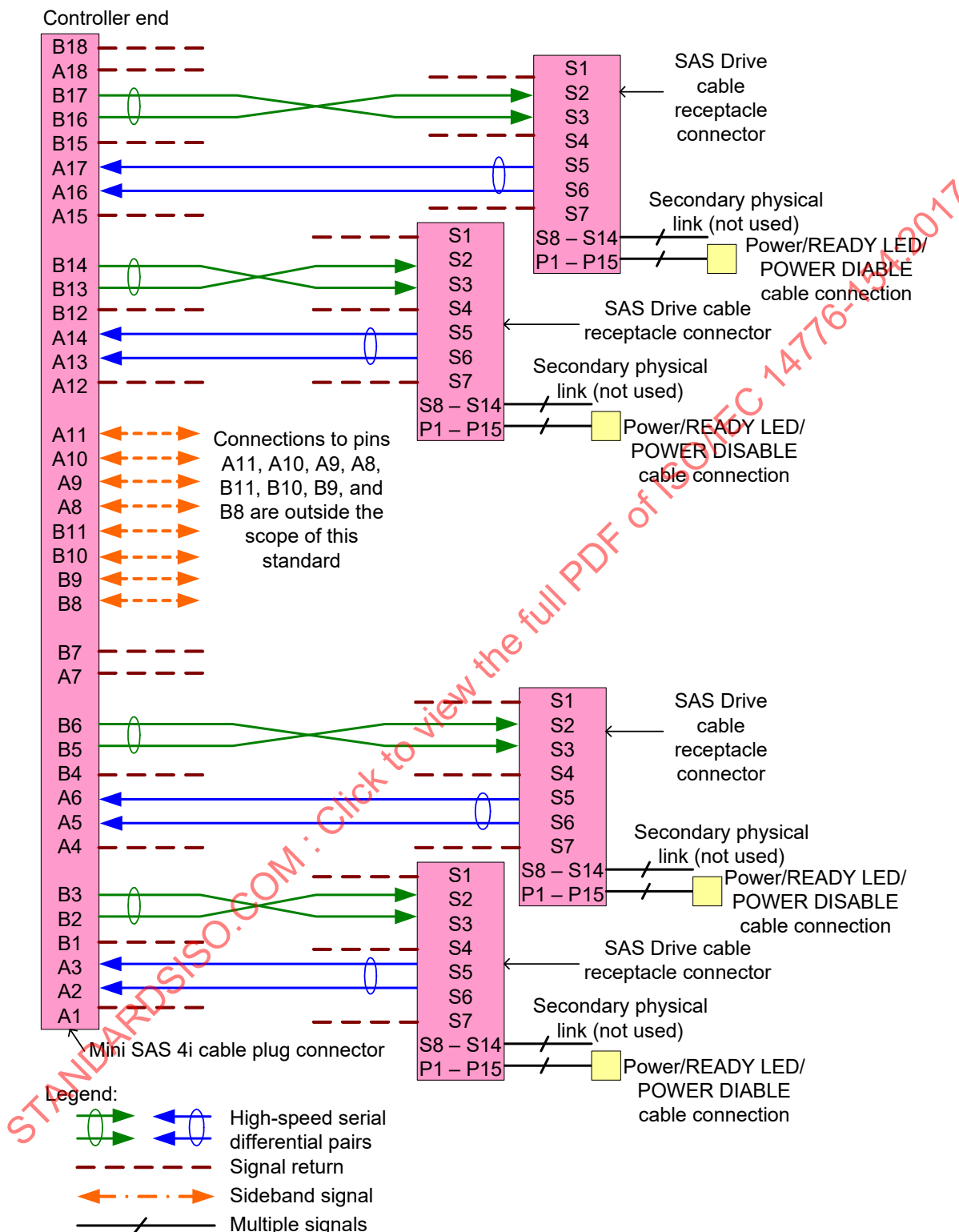
Figure 81 – SAS internal controller-based fanout cable assembly - Mini SAS 4i
