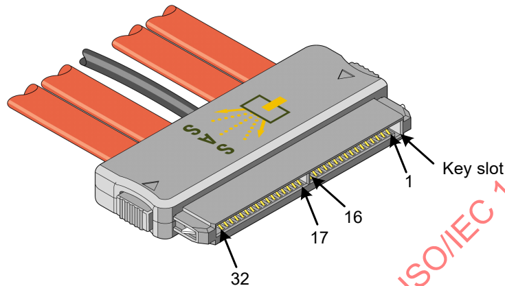
Figure 33 – SAS 4i cable receptacle connector
