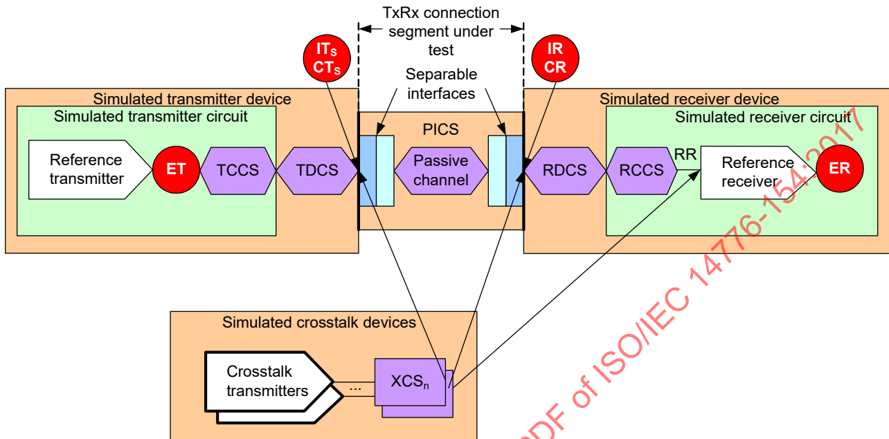
Figure 99 – Example passive TxRx connection compliance testing for trained 12 Gbit/s
