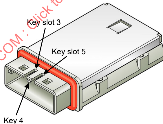
Figure 59 – Mini SAS 4x active receptacle connector - end device or enclosure universal port
