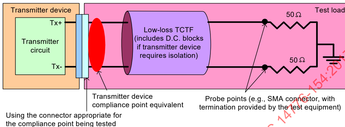
Figure 111 – Low-loss TCTF test load
