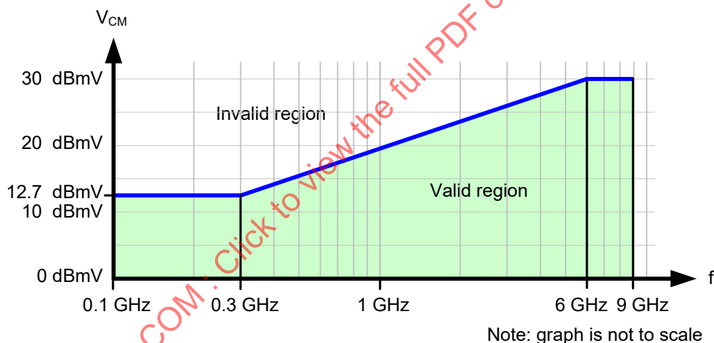
Figure 132 – 12 Gbit/s transmitter device common mode voltage limit
