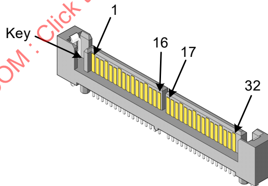
Figure 34 – SAS 4i plug connector
