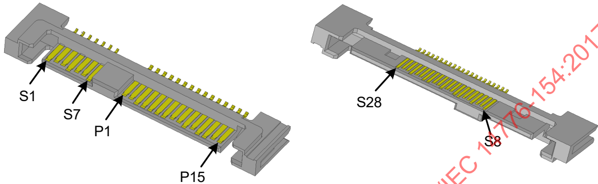
Figure 28 – SAS MultiLink Drive plug connector
