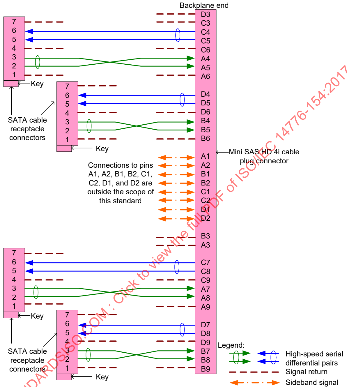
Figure 85 – SAS internal backplane-based fanout cable assembly - Mini SAS HD 4i
