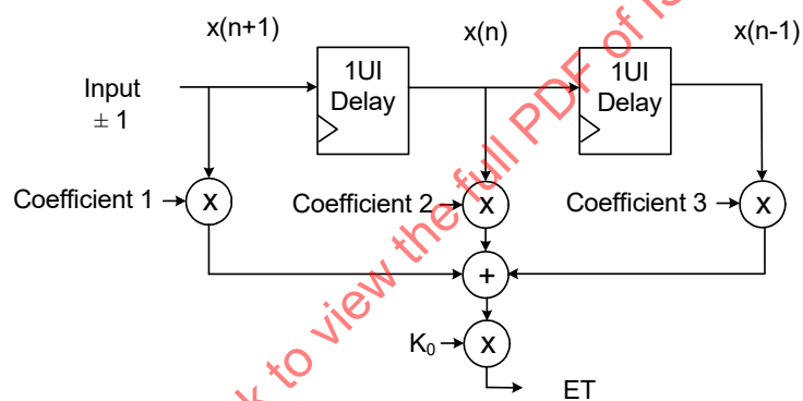
Figure 137 – 12 Gbit/s reference transmitter
