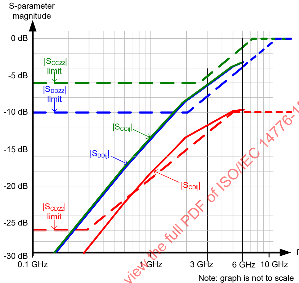
Figure 129 – Trained 1.5 Gbit/s, 3 Gbit/s, and 6 Gbit/s reference transmitter device termination S-parameters model
