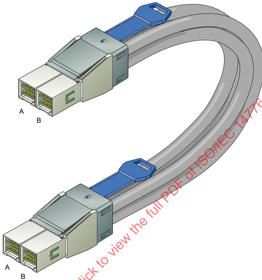
Figure 92 – SAS external cable assembly with Mini SAS HD 8x cable plug connectors
