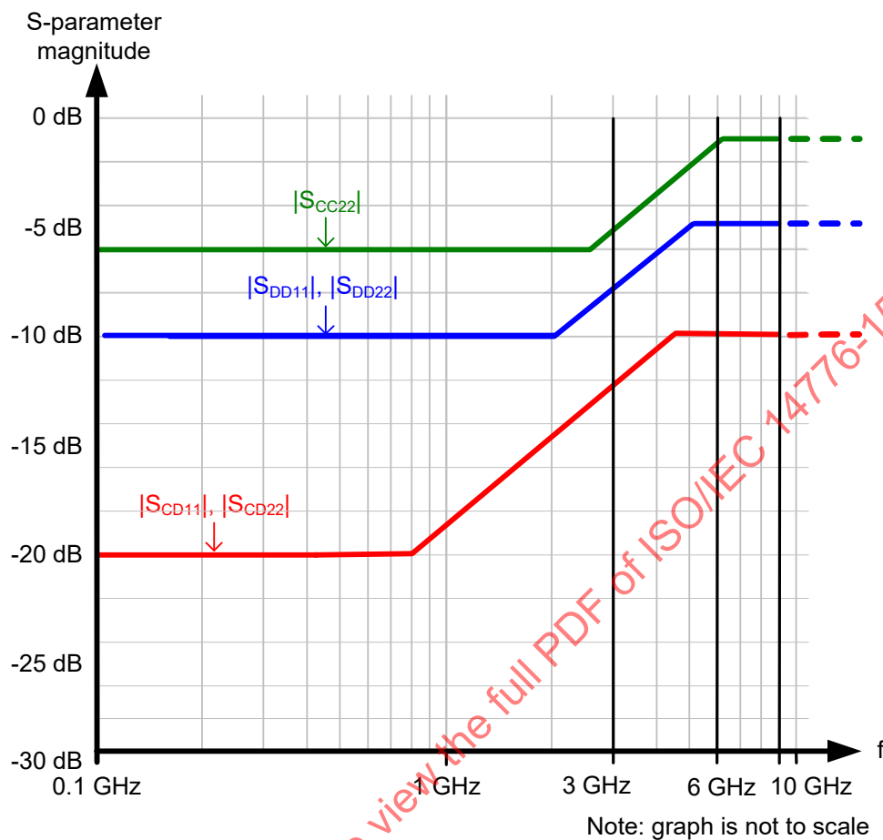
Figure 101 – Active cable S-parameter limits
