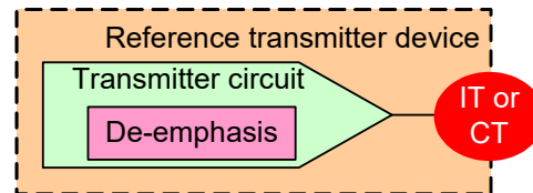
Figure 128 – Trained 1.5 Gbit/s, 3 Gbit/s, and 6 Gbit/s reference transmitter device
