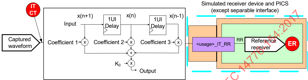
Figure 138 – Simulation of the reference transmitter from a captured signal
