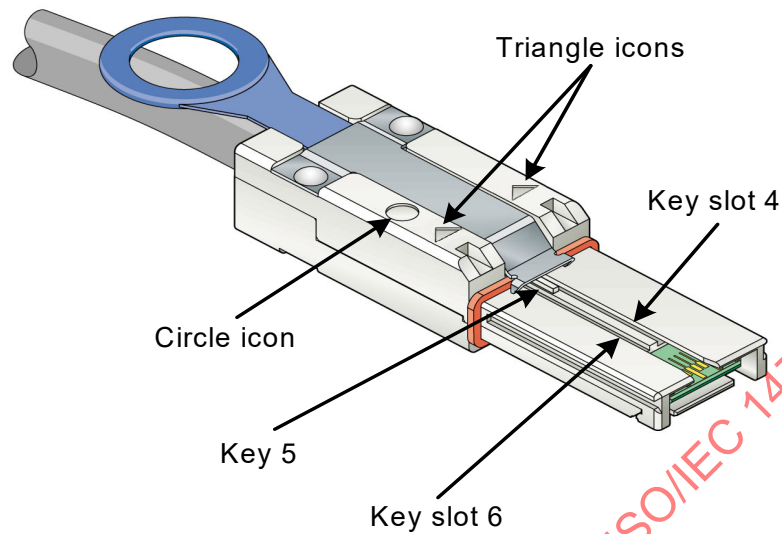
Figure 51 – Mini SAS 4x active cable plug connector for trained 1.5 Gbit/s, 3 Gbit/s, and 6 Gbit/s that attaches to an enclosure in port
