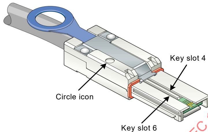
Figure 45 – Mini SAS 4x cable plug connector for untrained 1.5 Gbit/s and 3 Gbit/s that attaches to an enclosure in port
