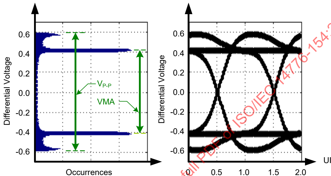
Figure 130 – Transmitter equalization measurement
