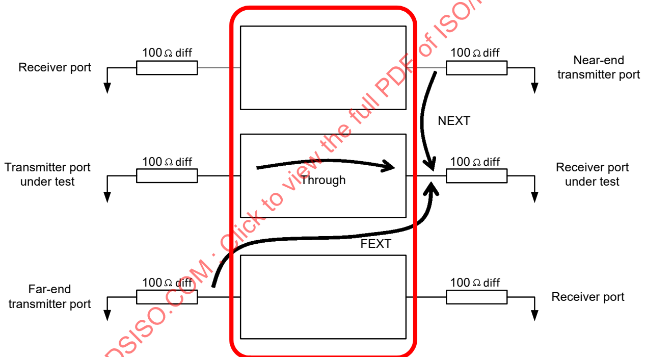
Figure 117 – NEXT and FEXT measurement definition
