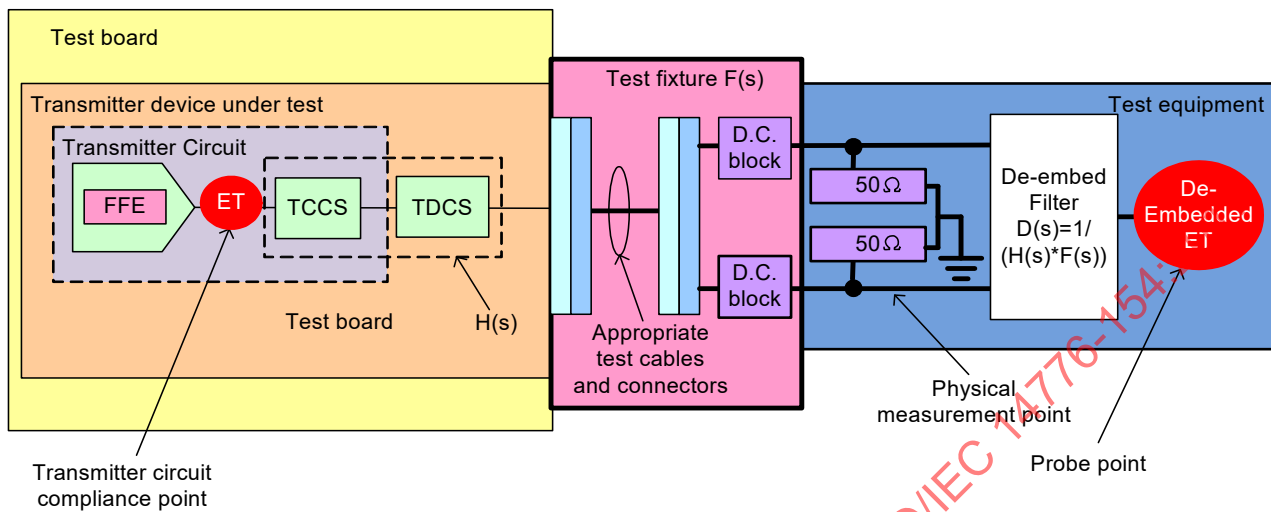
Figure 133 – Transmitter circuit compliance test configuration
