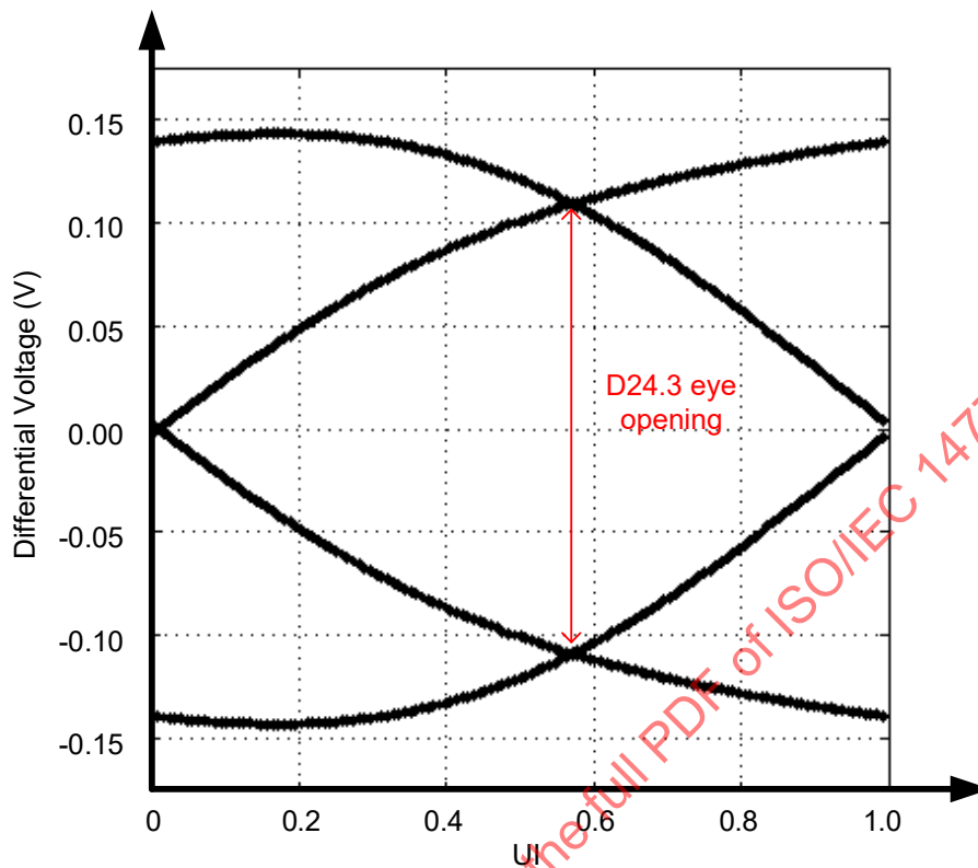
Figure 145 – Stressed receiver device jitter tolerance test D24.3 eye opening for trained 1.5 Gbit/s, 3 Gbit/s, and 6 Gbit/s
