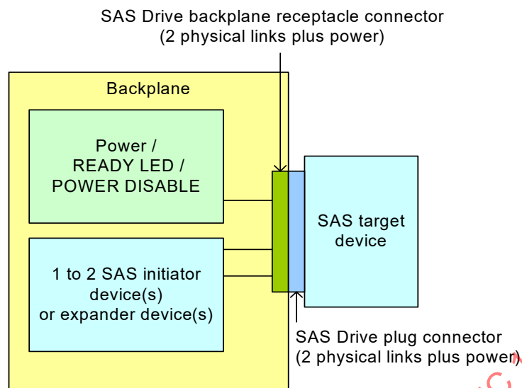
Figure 17 – SAS Drive backplane environment
