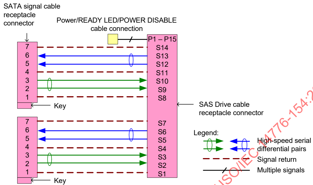
Figure 70 – Dual-port SAS Drive cable assembly
