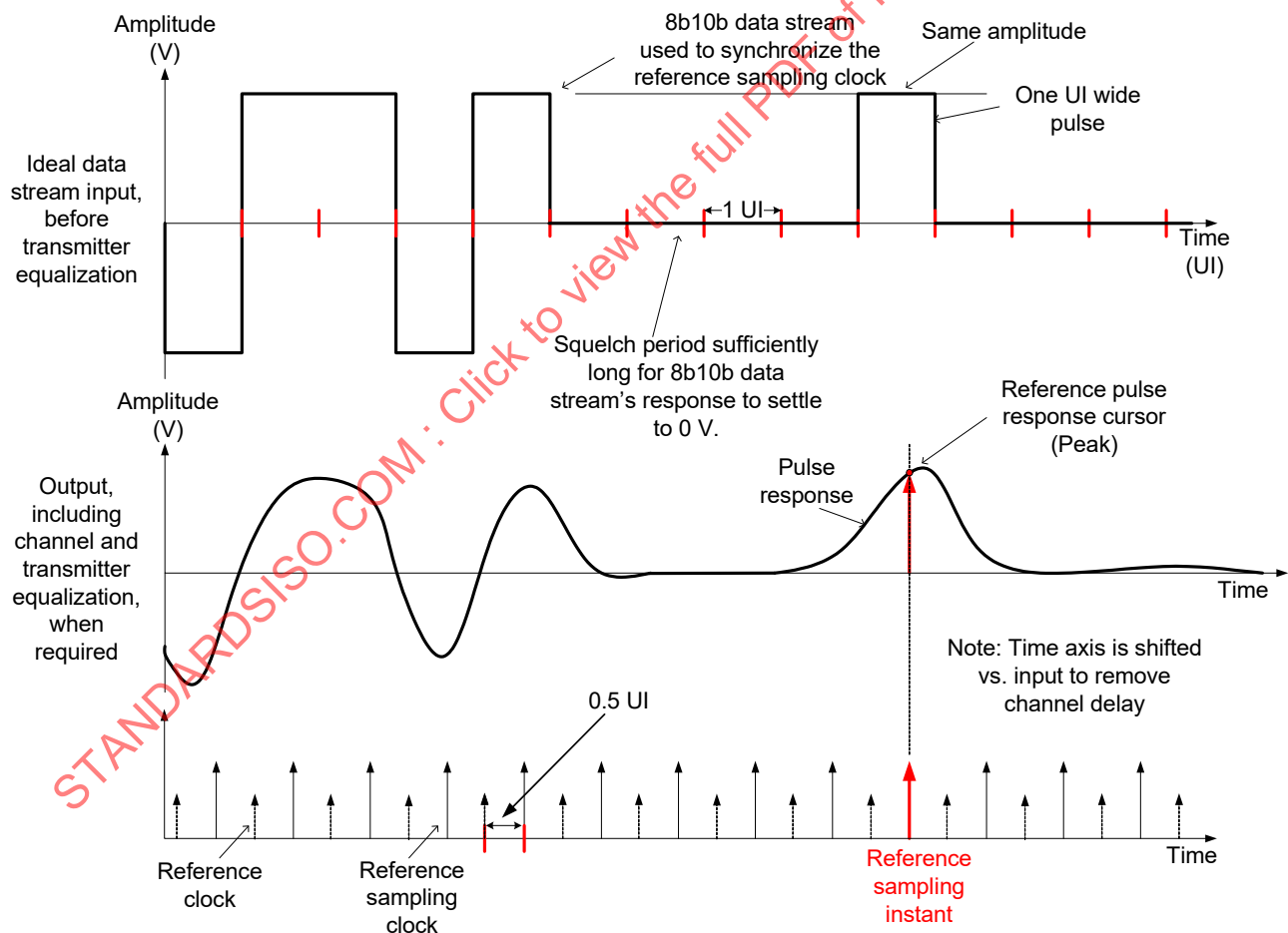
Figure 118 – Reference sampling point and reference pulse response cursor
