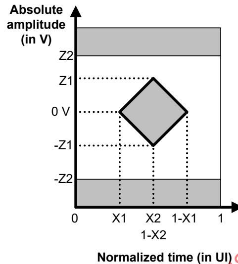
Figure 102 – Active cable eye mask for 12 Gbit/s
