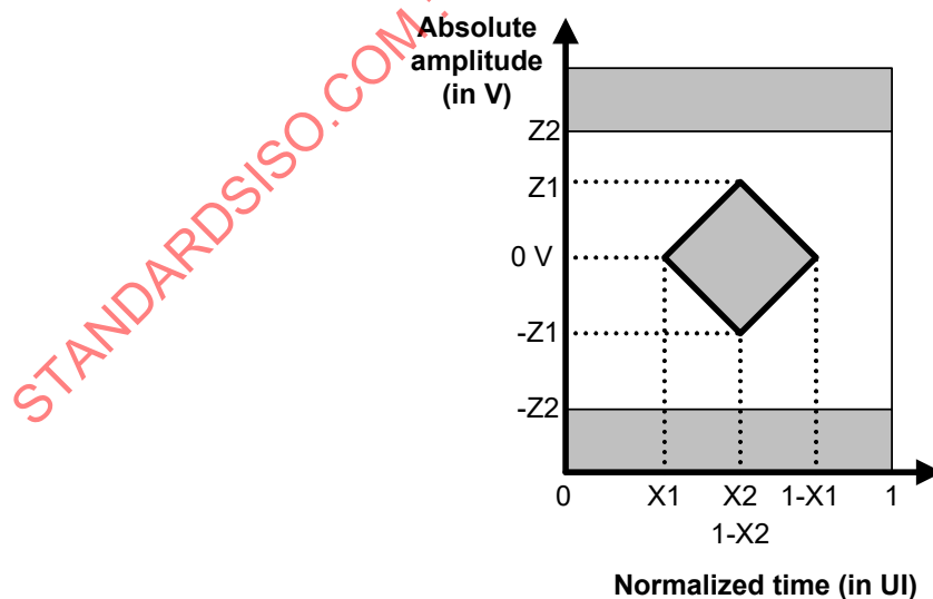
Figure 123 – Transmitter device eye mask
