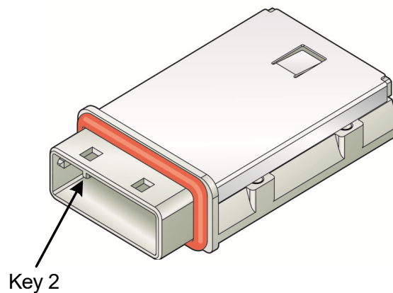
Figure 54 – Mini SAS 4x receptacle connector - enclosure out port for untrained 1.5 Gbit/s and 3 Gbit/s
