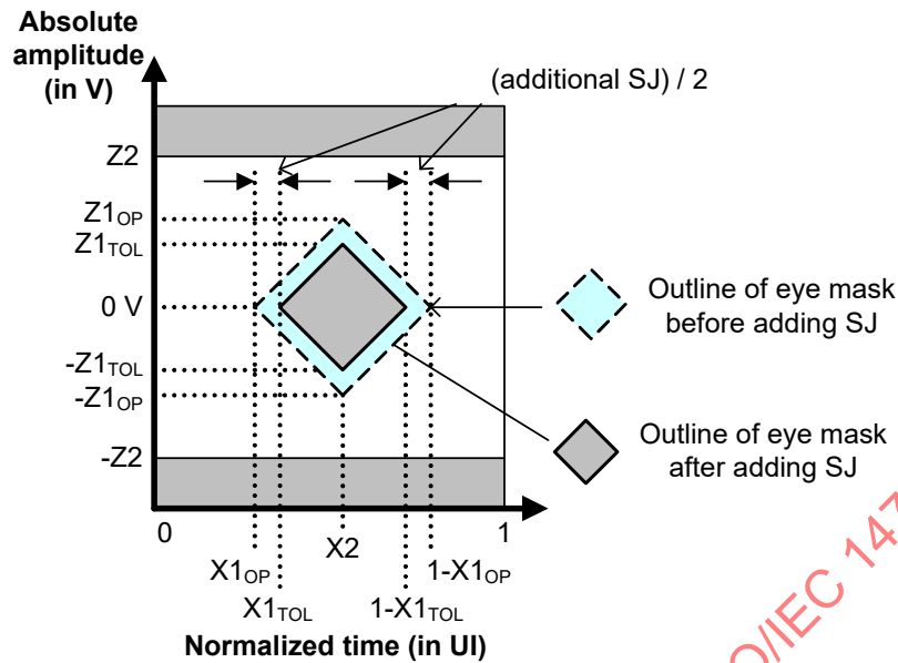
Figure 125 – Deriving a receiver device jitter tolerance eye mask for untrained 1.5 Gbit/s and 3 Gbit/s
