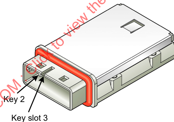
Figure 57 – Mini SAS 4x receptacle connector - enclosure out port for trained 1.5 Gbit/s, 3 Gbit/s, and 6 Gbit/s and for untrained 1.5 Gbit/s and 3 Gbit/s
