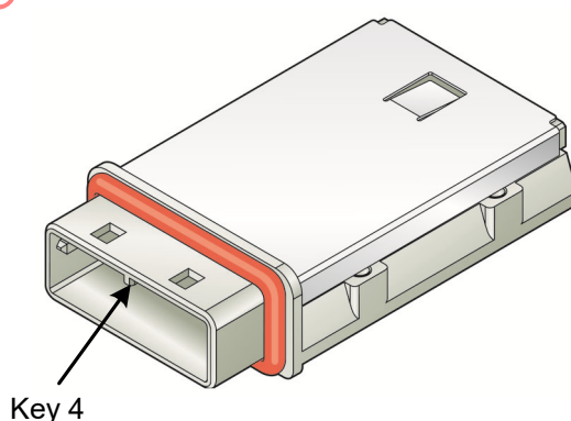
Figure 53 – Mini SAS 4x receptacle connector - end device or enclosure universal port for untrained 1.5 Gbit/s and 3 Gbit/s
