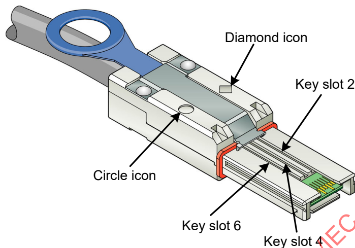
Figure 43 – Mini SAS 4x cable plug connector for untrained 1.5 Gbit/s and 3 Gbit/s that attaches to an enclosure out port or an enclosure in port
