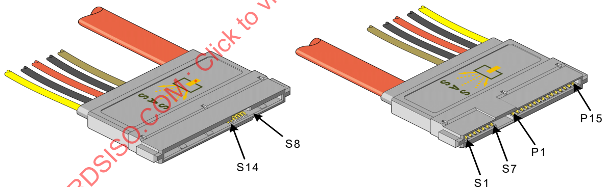
Figure 25 – Single-port SAS Drive cable receptacle connector
