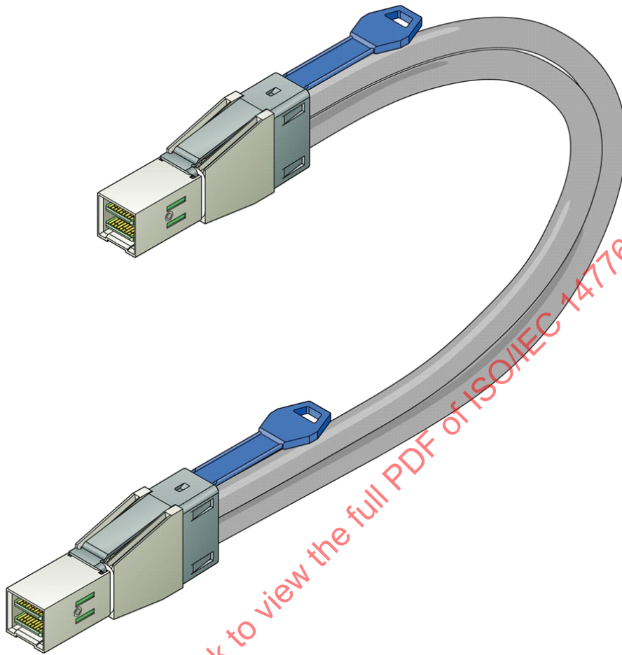
Figure 90 – SAS external cable assembly with Mini SAS HD 4x cable plug connectors
