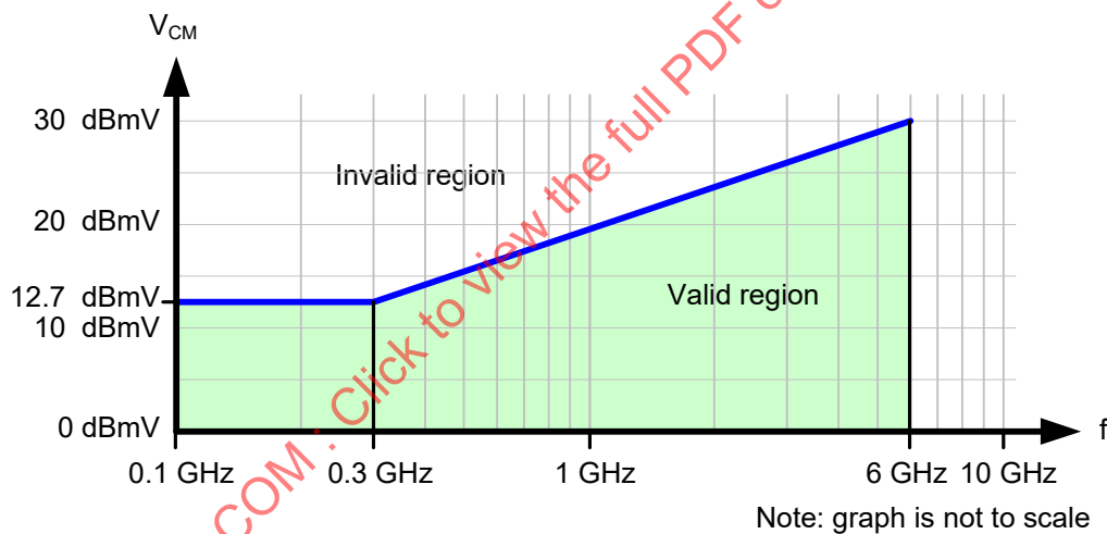
Figure 126 – Transmitter device common mode voltage limit
