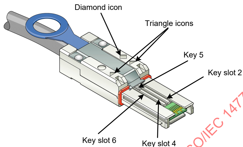
Figure 49 – Mini SAS 4x active cable plug connector for trained 1.5 Gbit/s, 3 Gbit/s, and 6 Gbit/s that attaches to an enclosure out port or an enclosure in port
