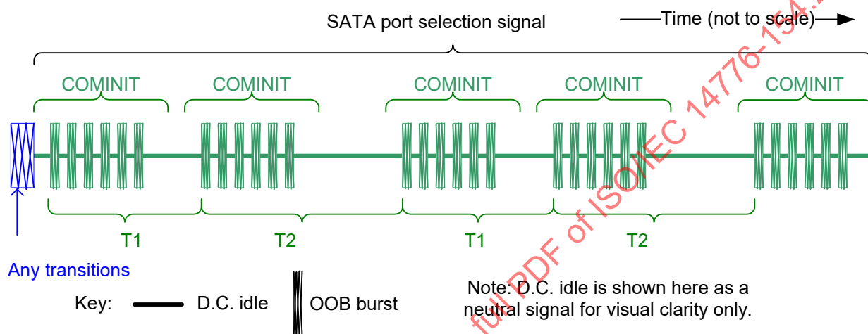
Figure 152 – SATA port selection signal
