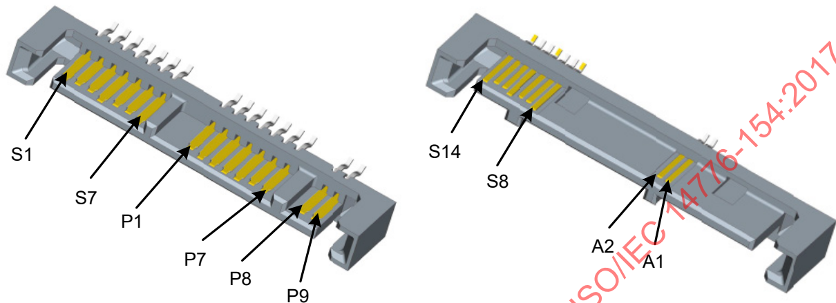
Figure 31 – Micro SAS plug connector
