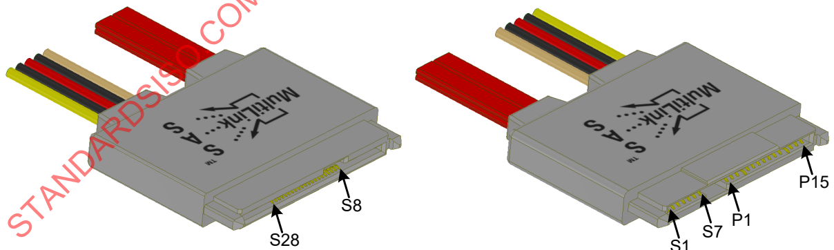
Figure 29 – SAS MultiLink Drive cable receptacle connector
