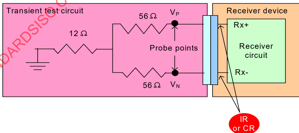
Figure 122 – Receiver device transient test circuit
