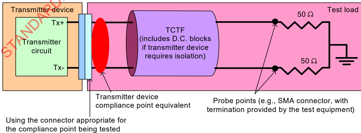
Figure 106 – TCTF test load
