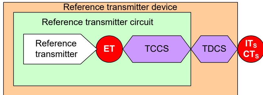
Figure 136 – 12 Gbit/s reference transmitter device
