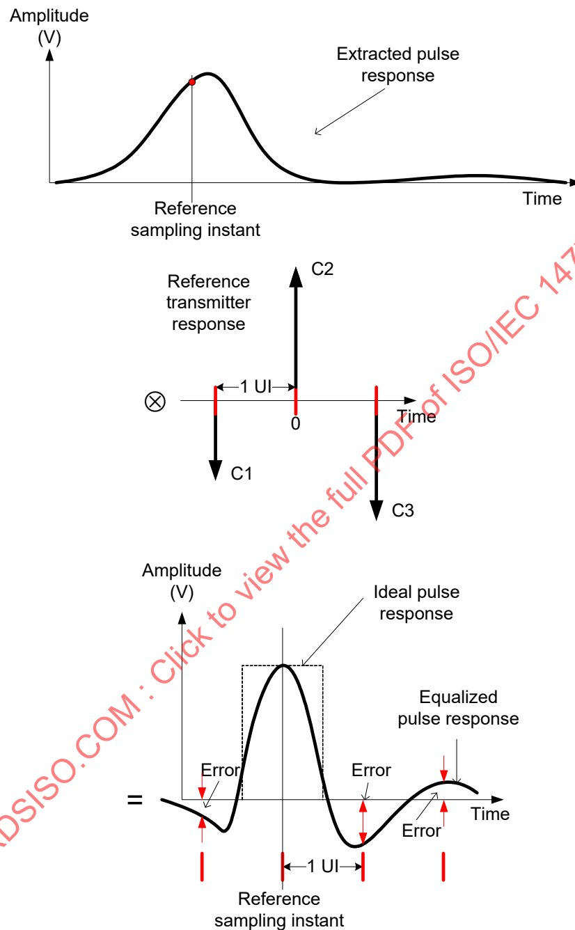
Figure 119 – Reference transmitter coefficient error computation
