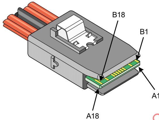
Figure 35 – Mini SAS 4i cable plug connector
