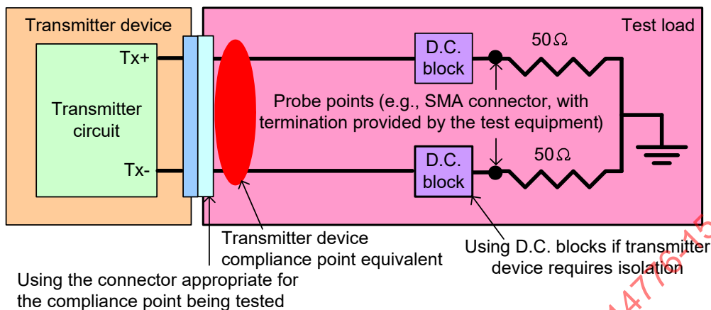
Figure 103 – Zero-length test load for transmitter device compliance point
