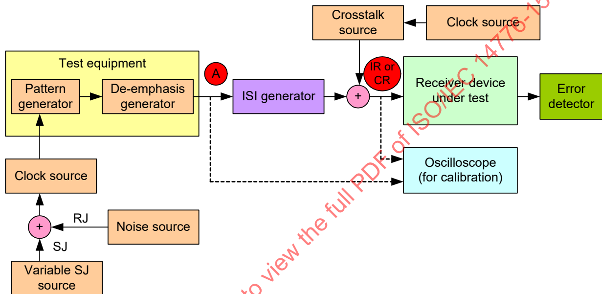
Figure 144 – Stressed receiver device jitter tolerance test block diagram for trained 1.5 Gbit/s, 3 Gbit/s, and 6 Gbit/s
