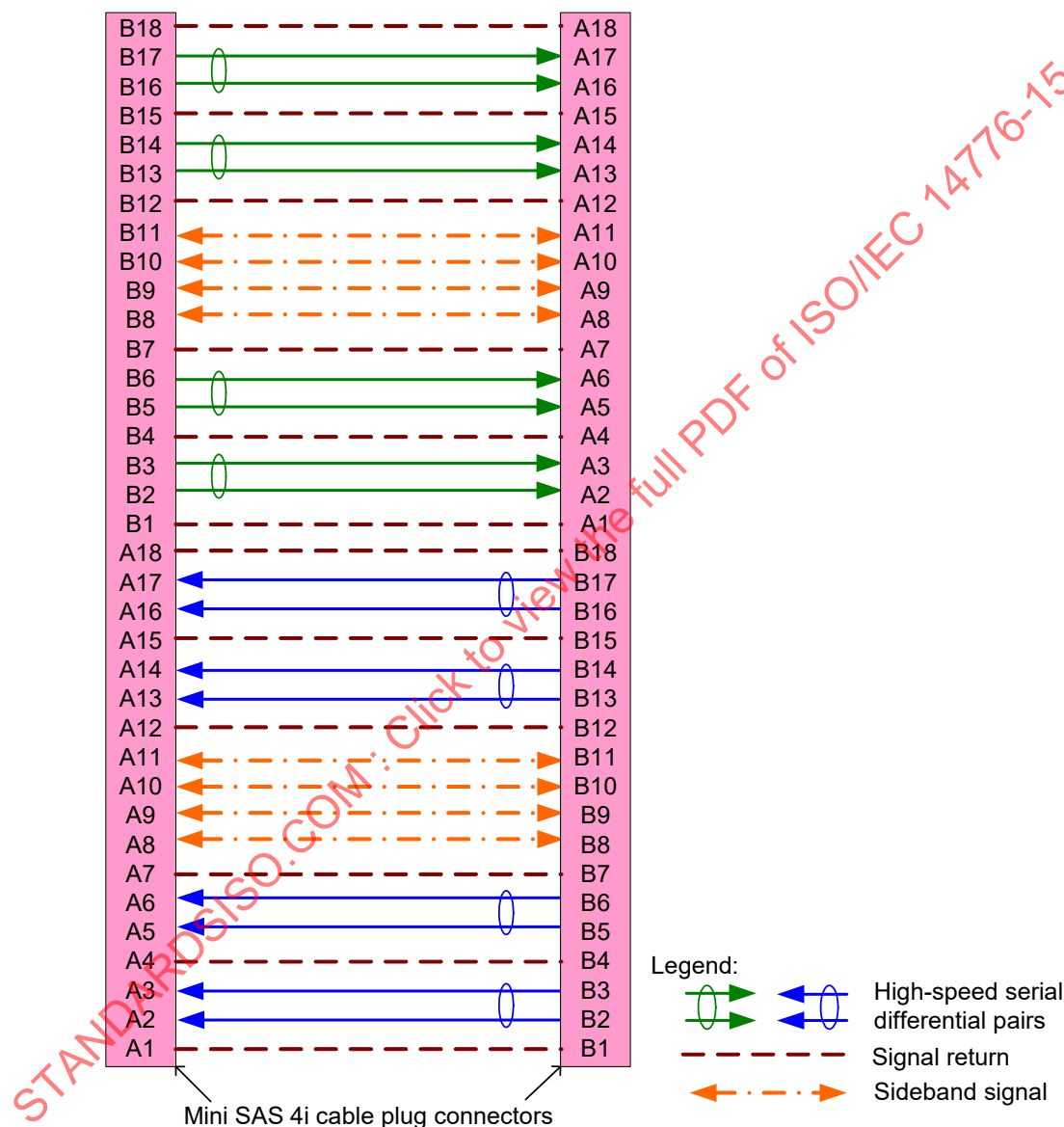
Figure 73 – SAS internal symmetric cable assembly - Mini SAS 4i
