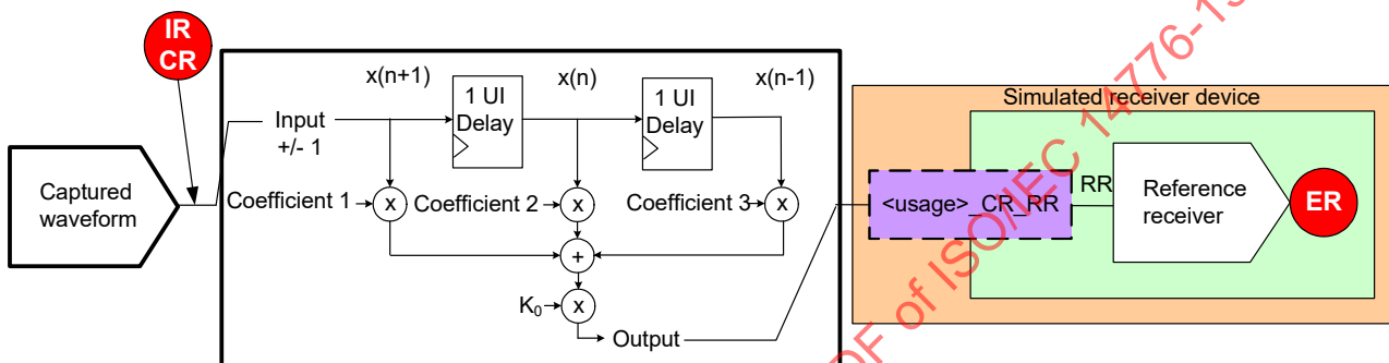
Figure 147 – Simulation of the reference transmitter from a captured signal
