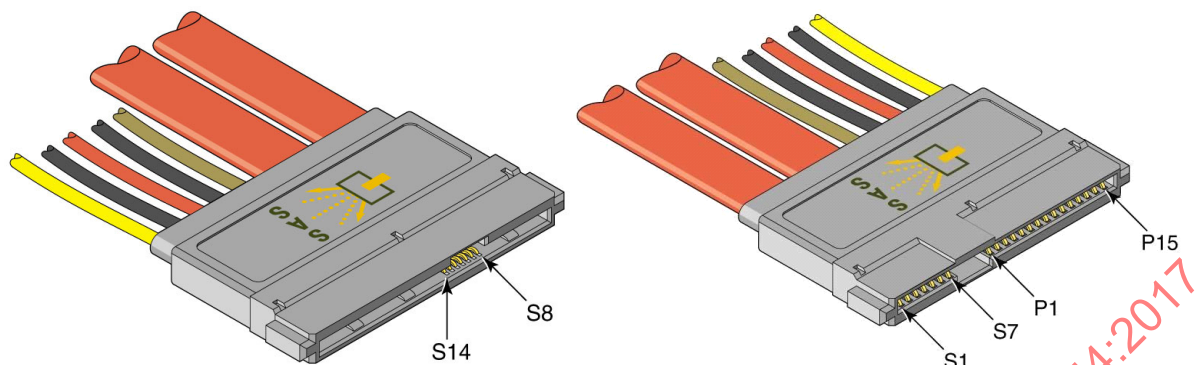
Figure 26 – Dual-port SAS Drive cable receptacle connector
