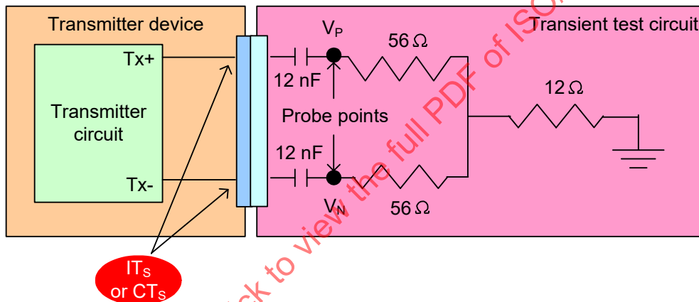
Figure 121 – Transmitter device transient test circuit
