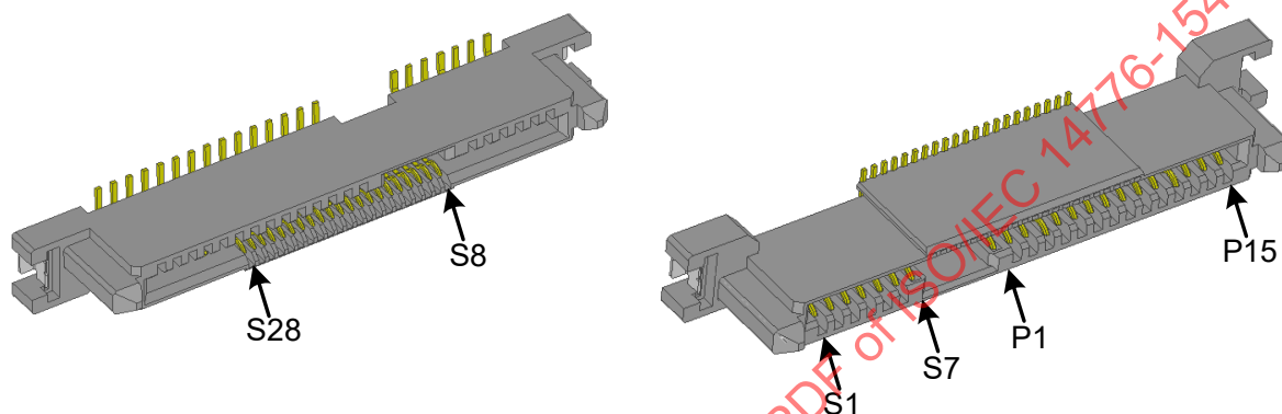
Figure 30 – SAS MultiLink Drive backplane receptacle connector
