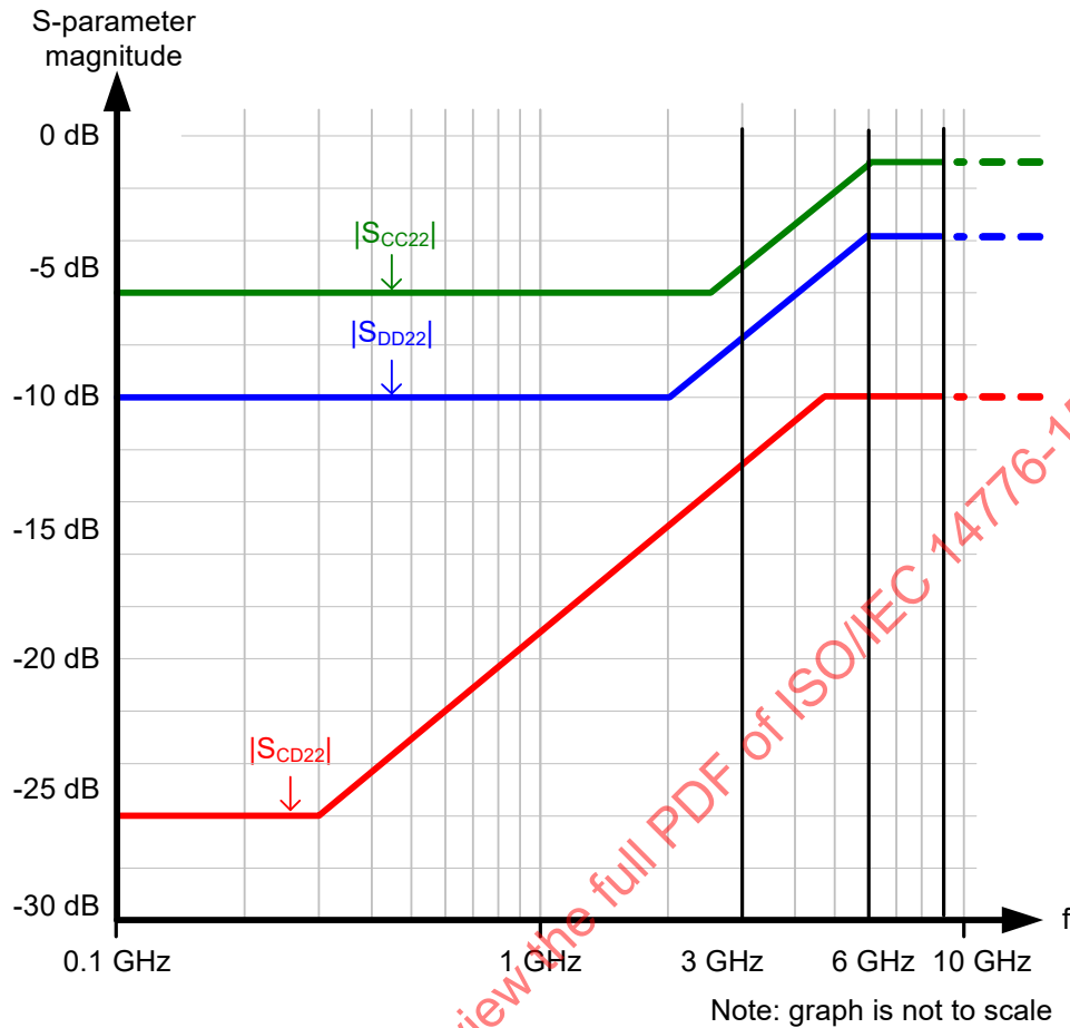
Figure 127 – Transmitter device |S_{CC22}| , |S_{DD22}| , and |S_{CD22}| limits
