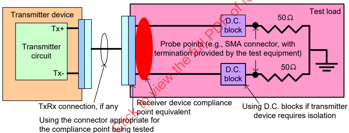
Figure 104 – Zero-length test load for receiver device compliance point
