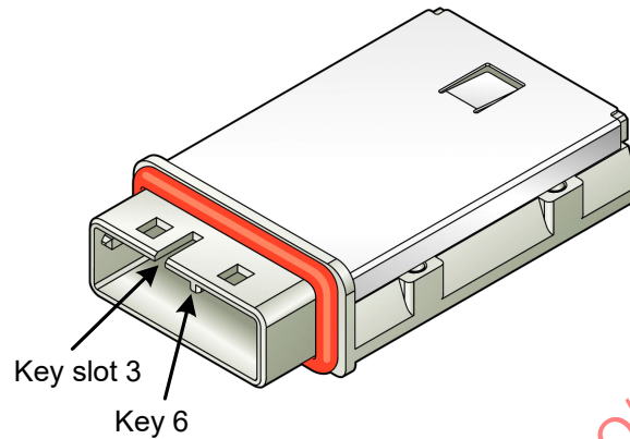
Figure 58 – Mini SAS 4x receptacle connector - enclosure in port for trained 1.5 Gbit/s, 3 Gbit/s, and 6 Gbit/s and for untrained 1.5 Gbit/s and 3 Gbit/s
