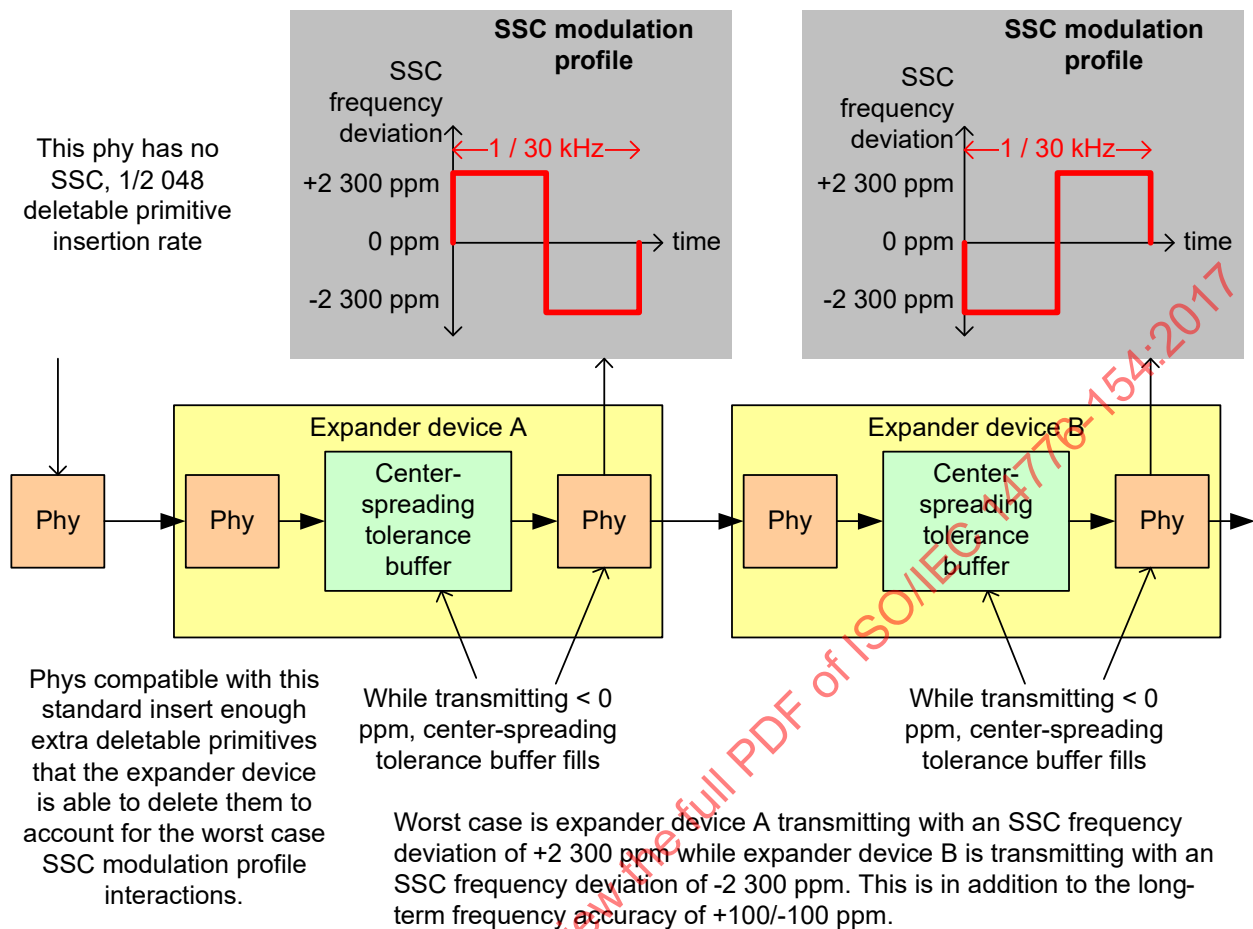
Figure 150 – Center-spreading tolerance buffer
