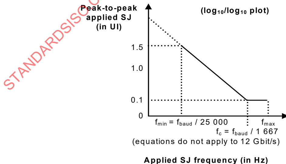
Figure 148 – Applied SJ for trained 1.5 Gbit/s, 3 Gbit/s, 6 Gbit/s, and 12 Gbit/s without SSC support
