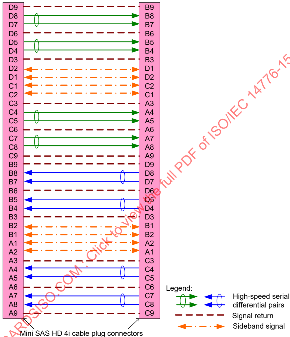
Figure 74 – SAS internal symmetric cable assembly - Mini SAS HD 4i
