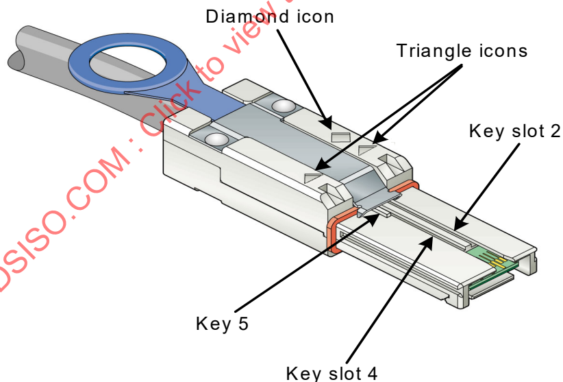
Figure 50 – Mini SAS 4x active cable plug connector for trained 1.5 Gbit/s, 3 Gbit/s, and 6 Gbit/s that attaches to an enclosure out port
