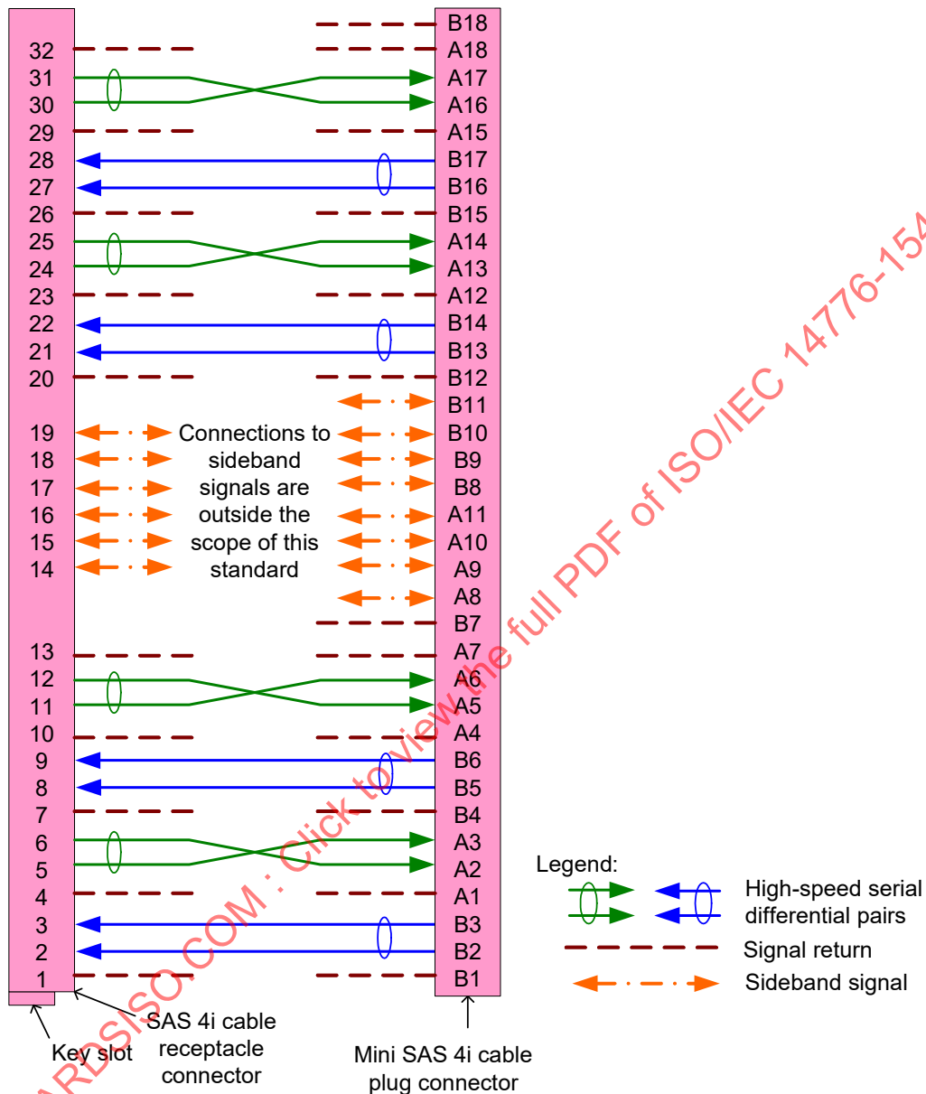
Figure 76 – SAS internal symmetric cable assembly - SAS 4i to Mini SAS 4i with vendor-specific sideband signals
