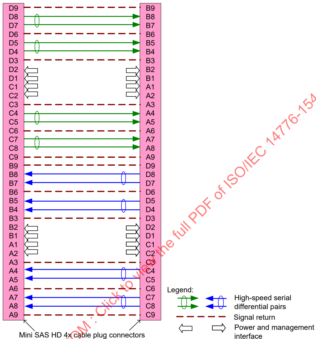
Figure 89 – SAS external cable assembly - Mini SAS HD 4x
