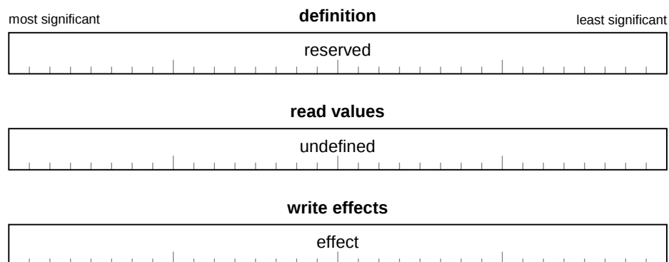
Figure 31 – DOORBELL format
