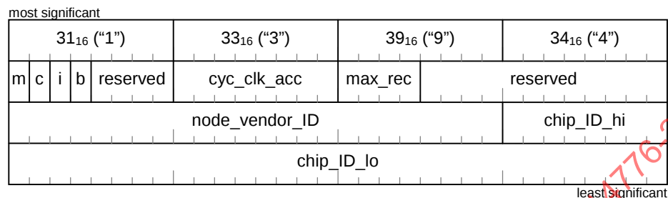
Figure 34 – Bus information block format
