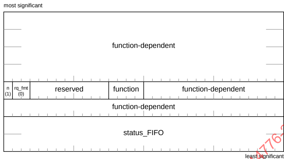
Figure 15 – Management ORB
