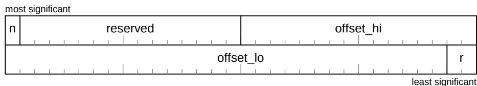
Figure 10 – ORB pointer
