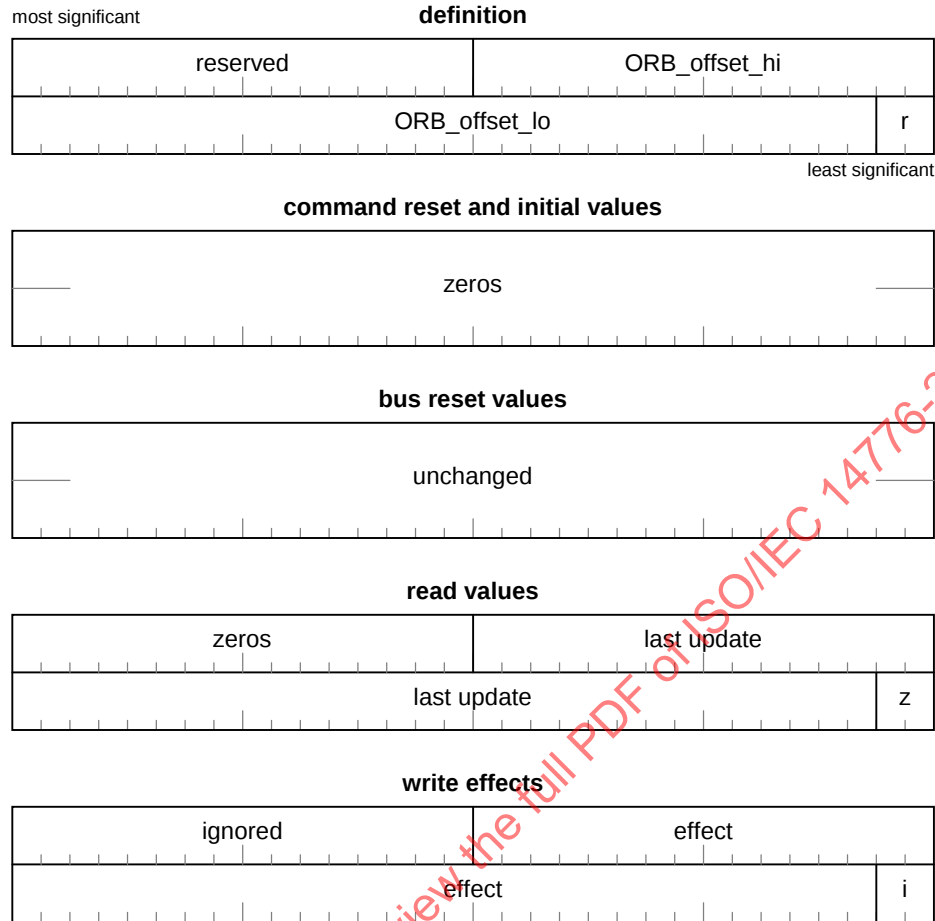
Figure 30 – ORB_POINTER format
