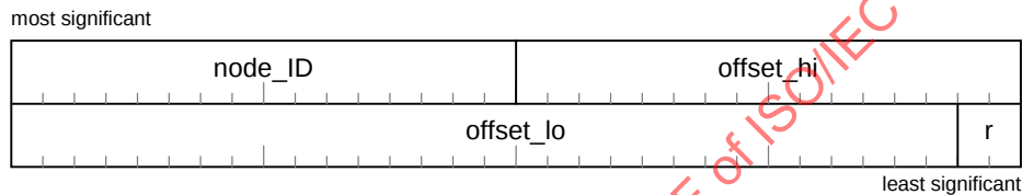
Figure 9 – Address pointer
