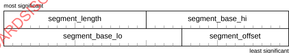
Figure 24 – Page table element (when page_size equals four)
