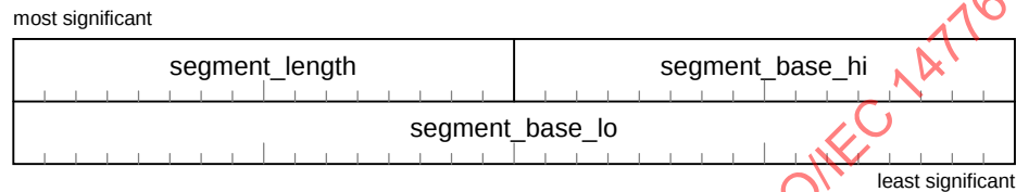
Figure 23 – Page table element (unrestricted page table)
