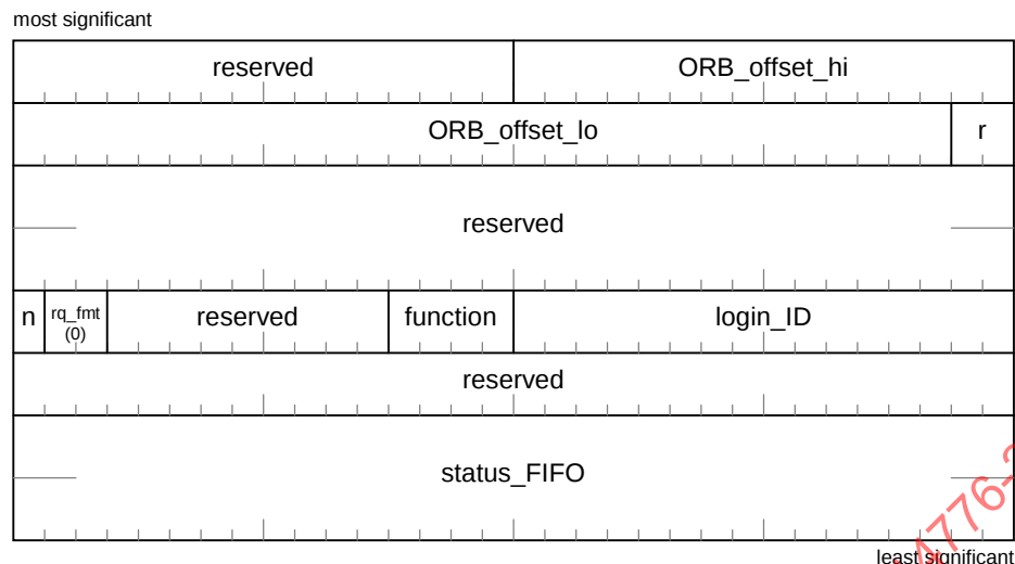
Figure 22 – Task management ORB
