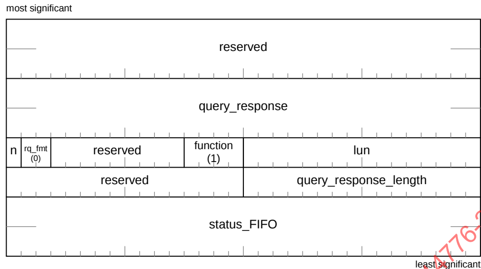
Figure 18 – Query logins ORB
