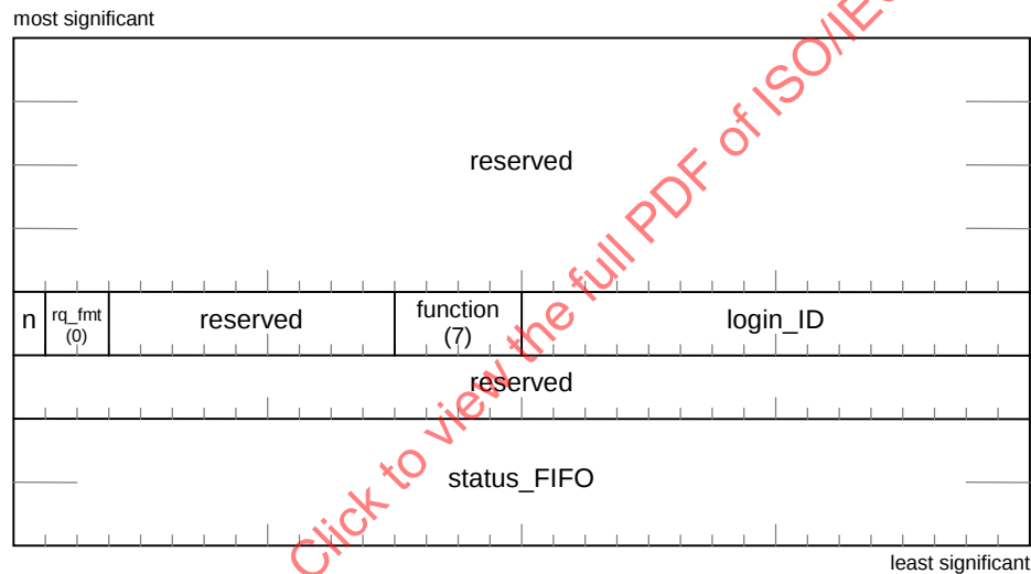
Figure 21 – Logout ORB
