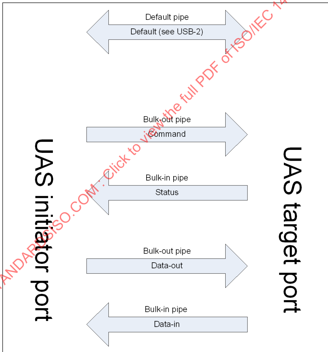
Figure 3 – USB Model
