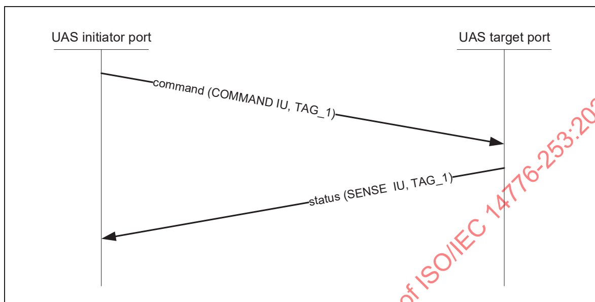
Figure 6 – Non-data transfer with Sense
