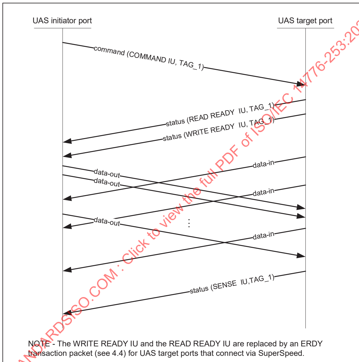
Figure 11 – Bi-directional Data Transfer
