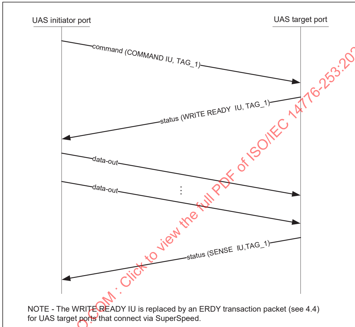
Figure 8 – Write Data Transfer
