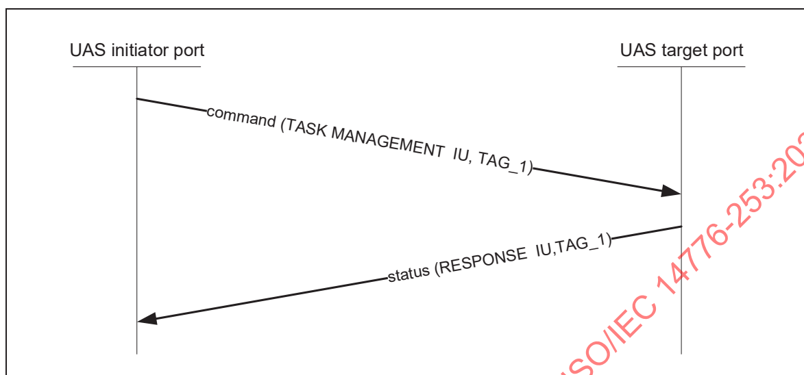
Figure 10 – Task Management
