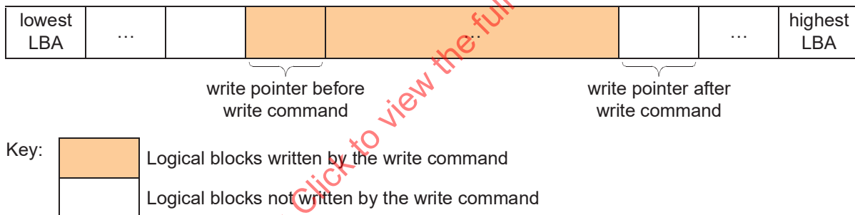
Figure 12 – Example write command that starts at the write pointer
