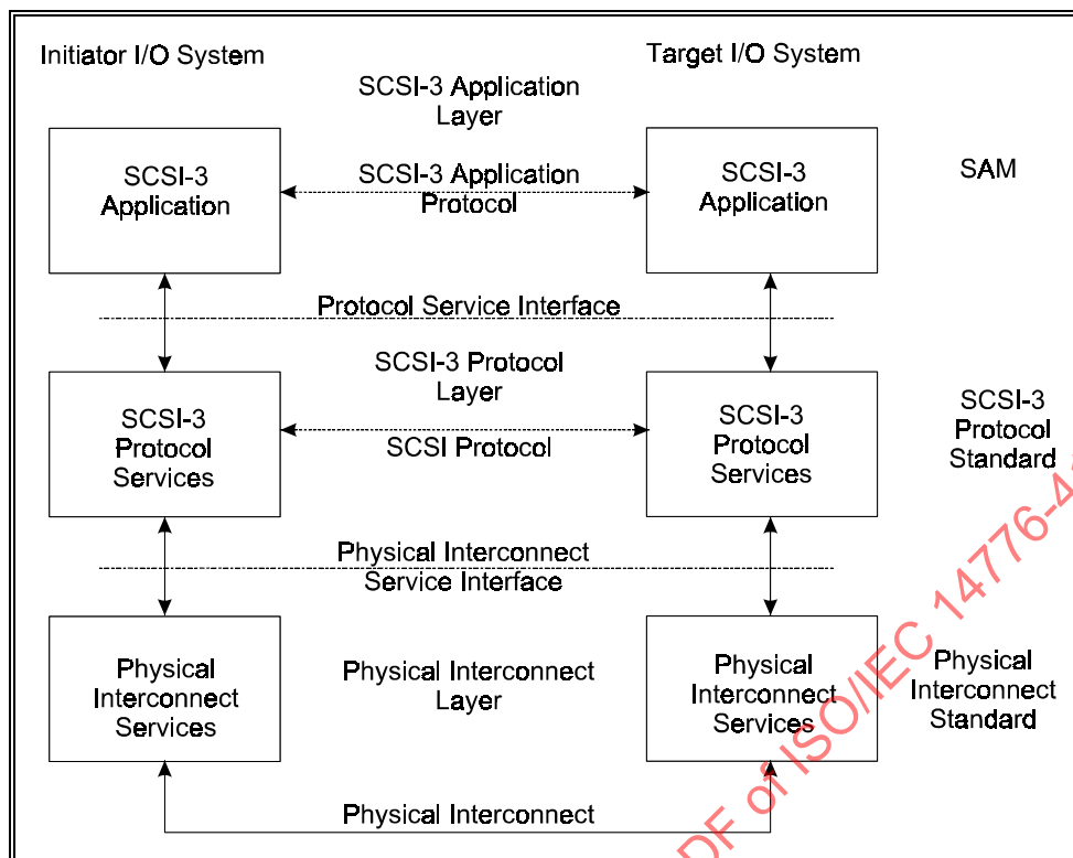
Figure 15 – Protocol Service Reference Model
