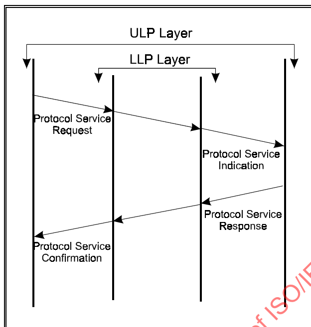
Figure 16 – Protocol Service Model
