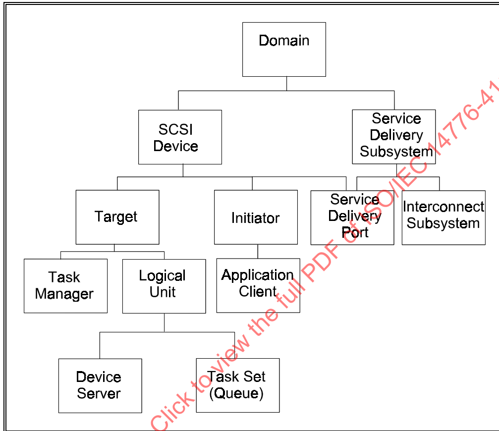
Figure 7 – SCSI Hierarchy
