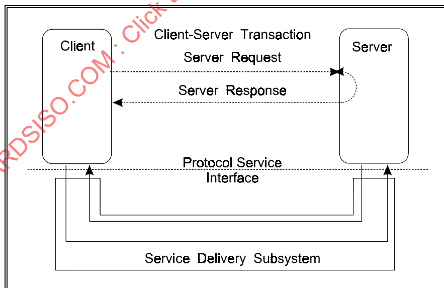
Figure 4 – Client-Server Model
