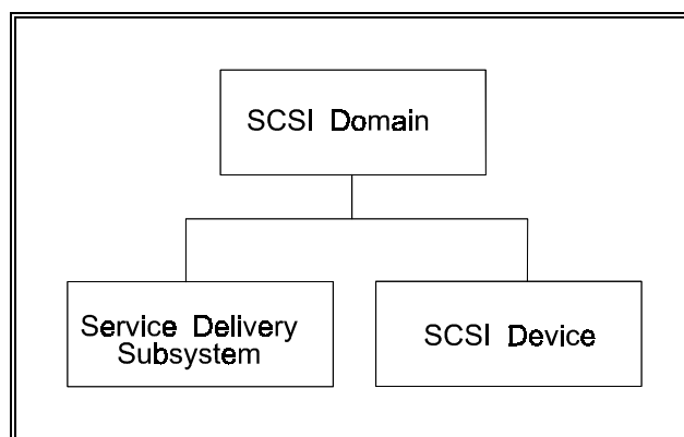
Figure 9 – Domain Hierarchy
