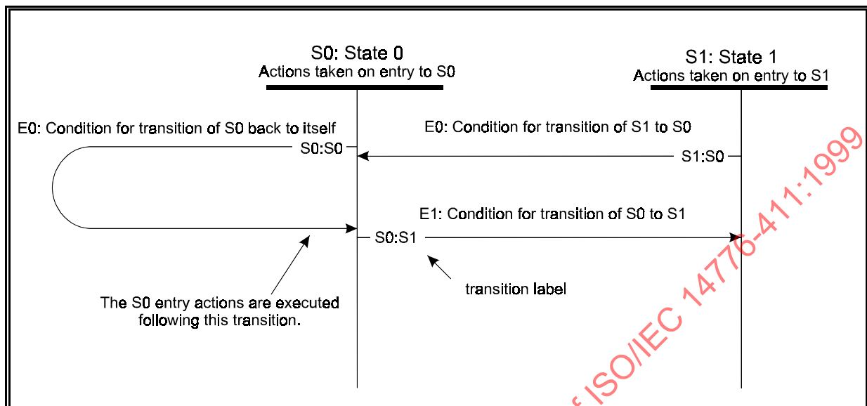
Figure 3 – State Diagram
