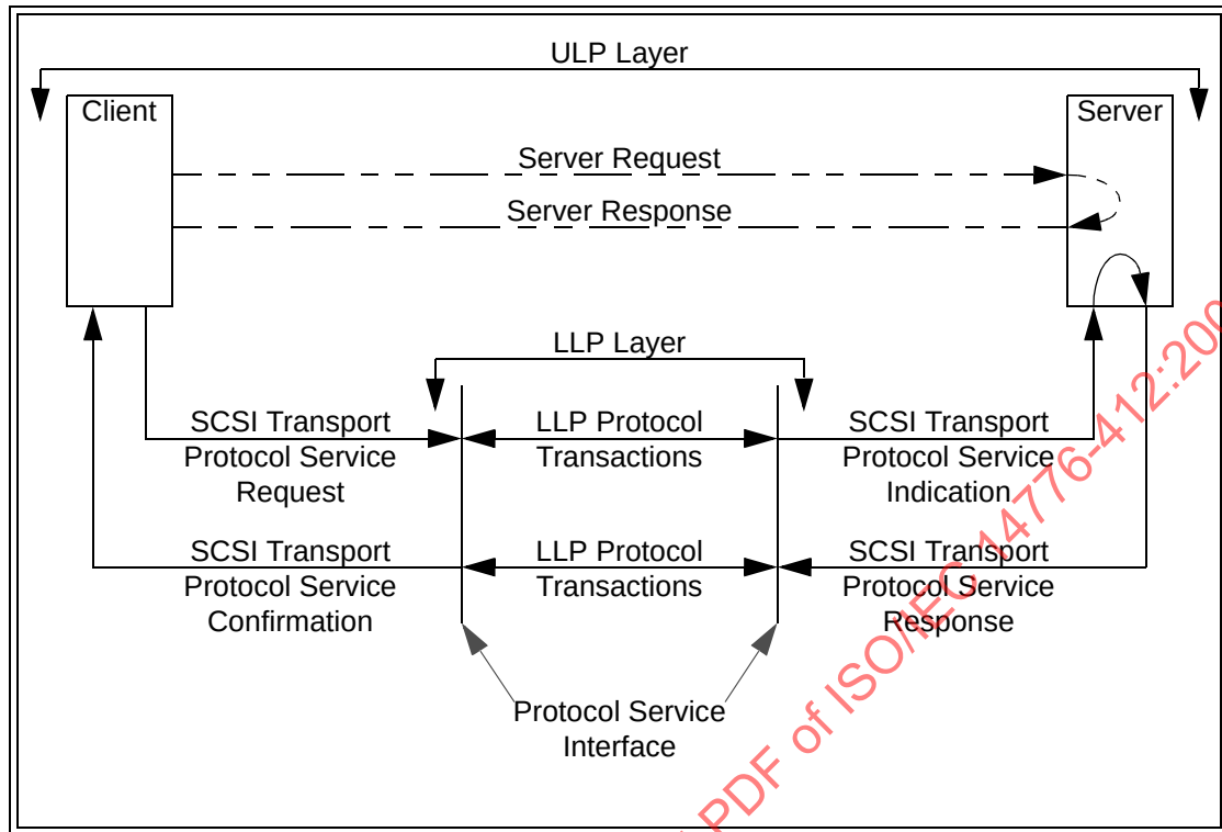
Figure 26 — Request-Response ULP transaction and related LLP services
