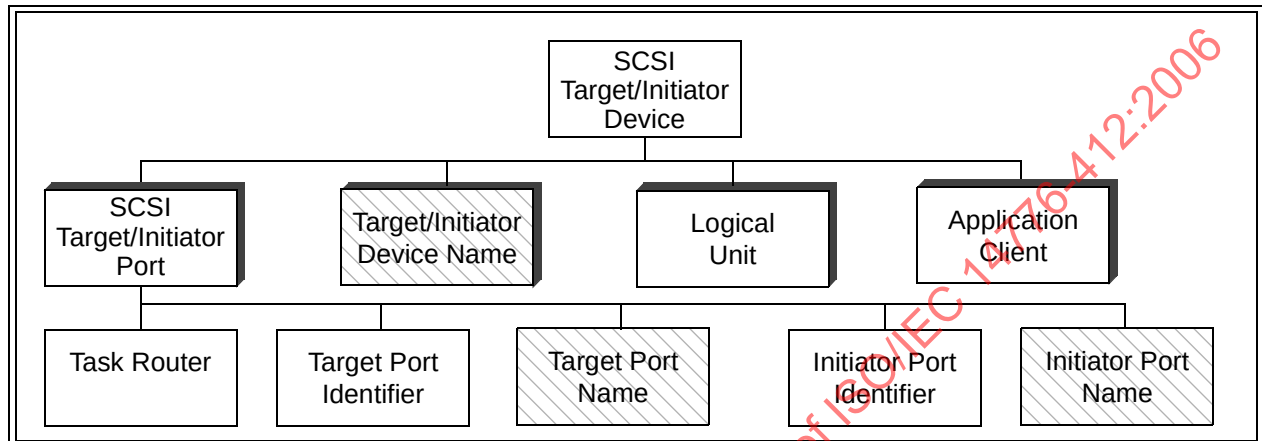
Figure 12 — SCSI target/initiator device model
