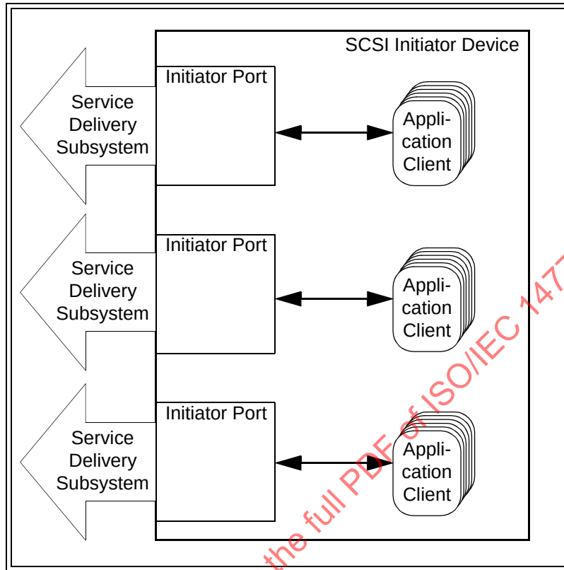
Figure 17 — Multiple port SCSI initiator device structure model
