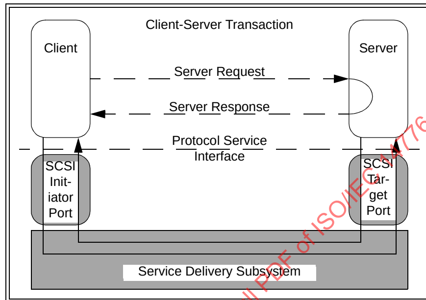
Figure 4 — Client-Server model
