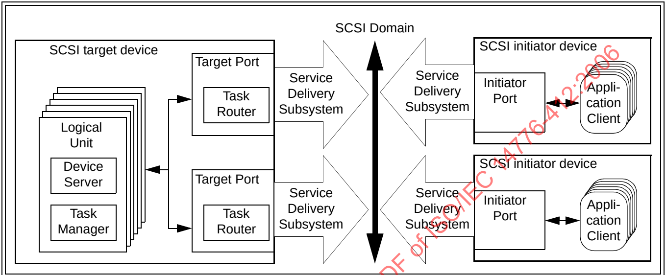
Figure 19 — SCSI target device configured in a single SCSI domain
