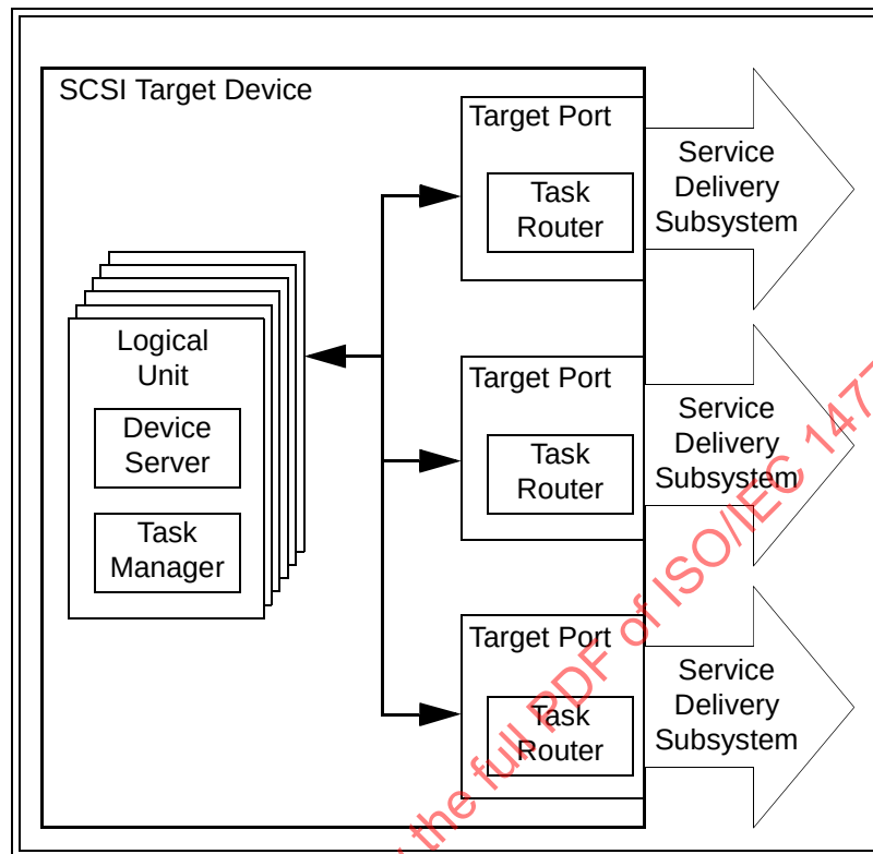
Figure 16 — Multiple port target SCSI device structure model
