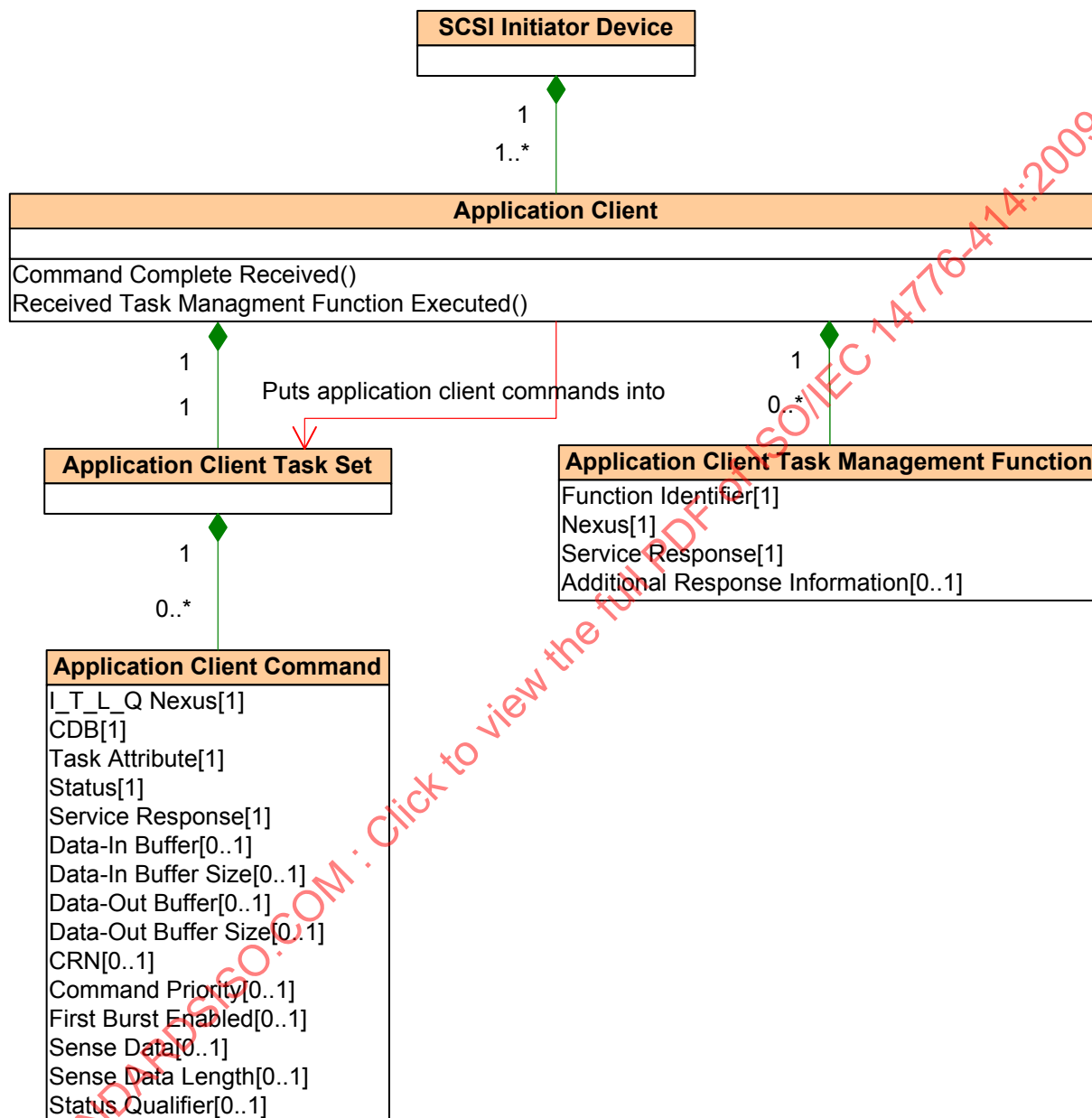
Figure 17 — SCSI Initiator Device class diagram
