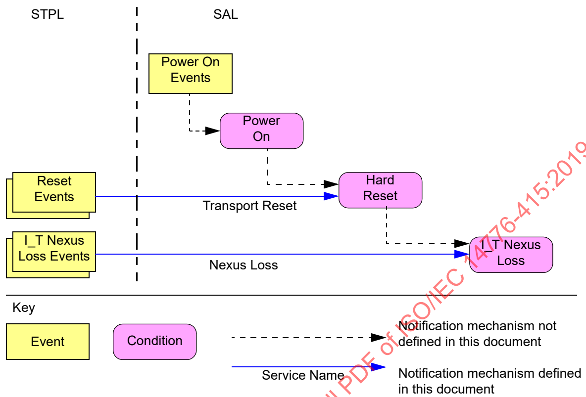
Figure 42 — Events and event notifications for SCSI initiator devices
