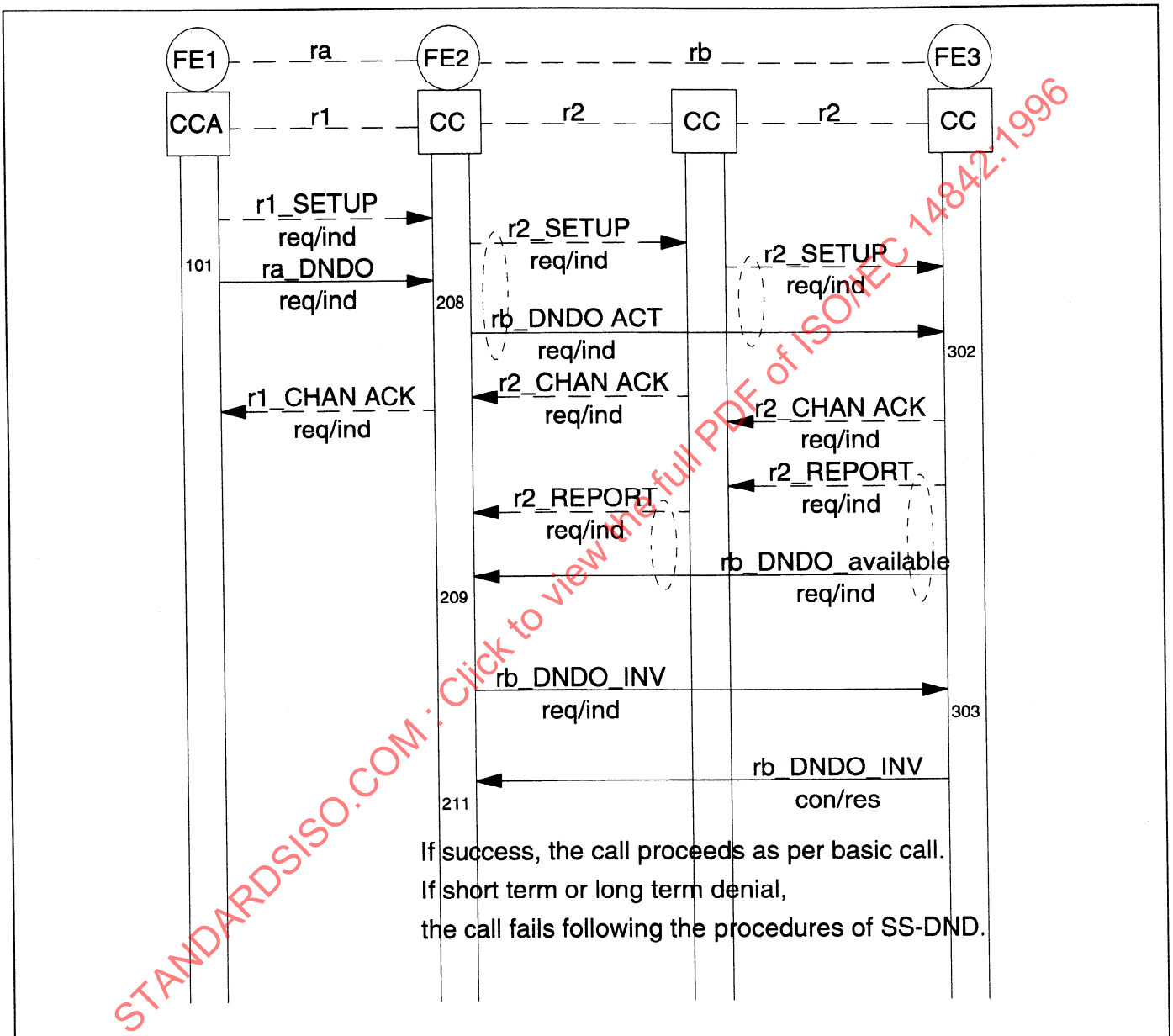
Figure 18 - Information flow sequence - normal operation of SS-DNDO - immediate invocation, path retention method
