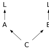
Figure 3 — Non-virtual base
