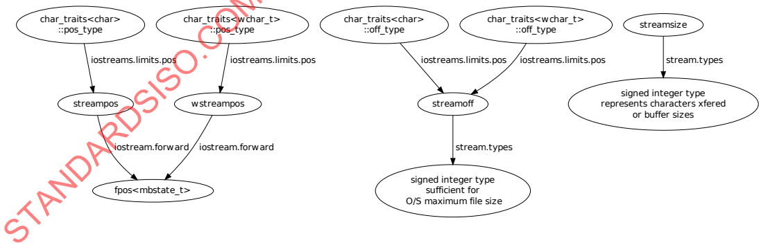
Figure 7 — Stream position, offset, and size types [non-normative]
