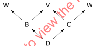
Figure 6 — Name lookup
