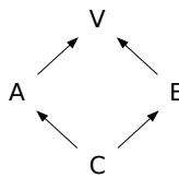
Figure 4 — Virtual base
