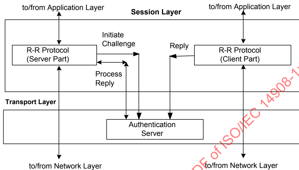
Figure 23 — Session layer—internal structuring
