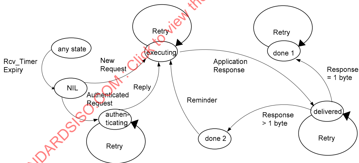
Figure 28 — Request-response protocol—simplified server FSM
