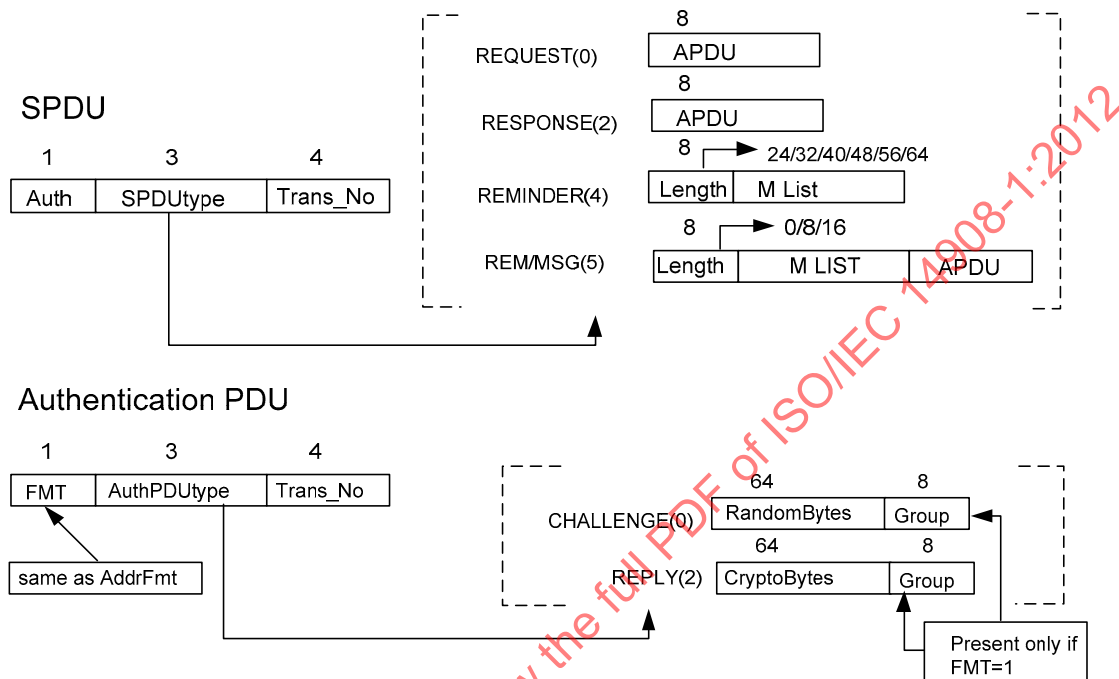
Figure 24 — SPDU types and formats
