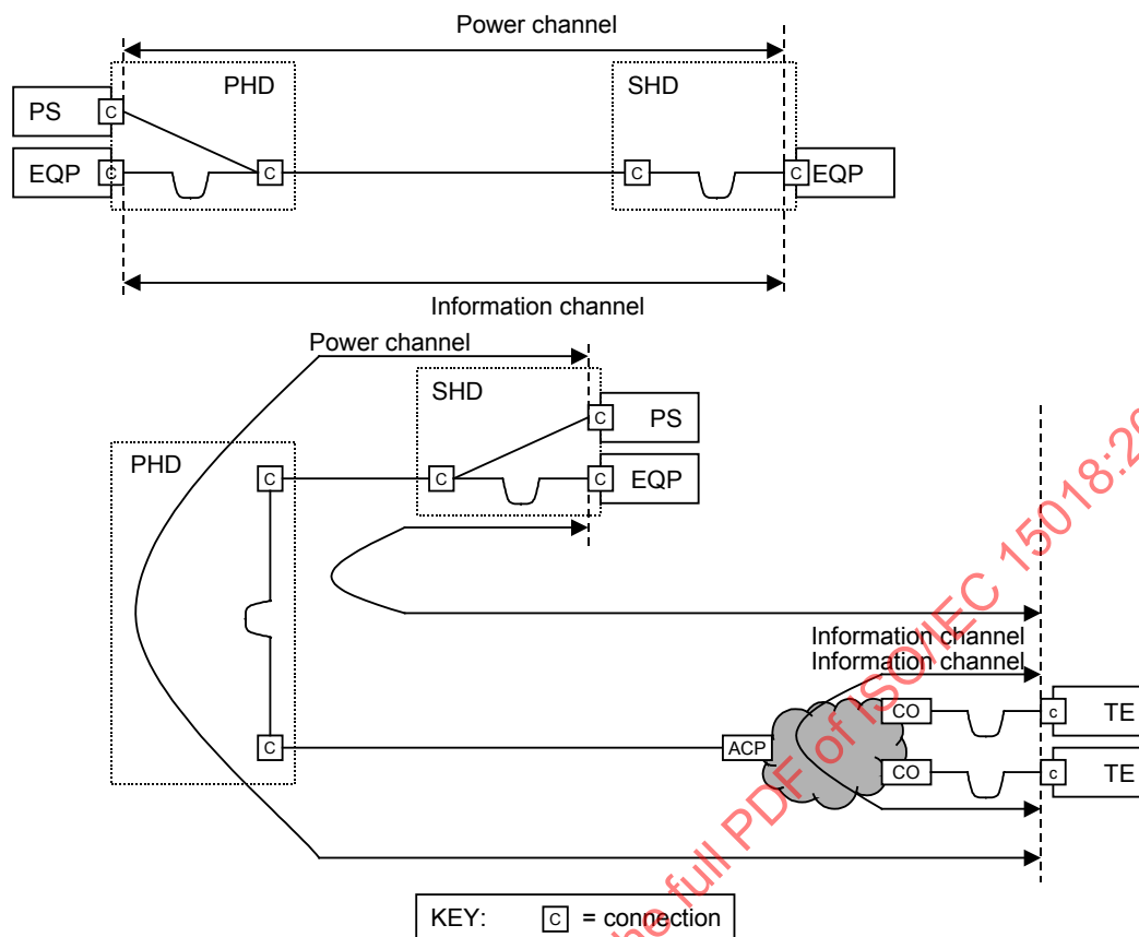
Figure 15 – Reference implementations for CCCB channels with PHD and SHD
