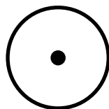
Figure 19 – Conductor assignment of IEC 61169-2 and IEC 61169-24 (Type F) connector
