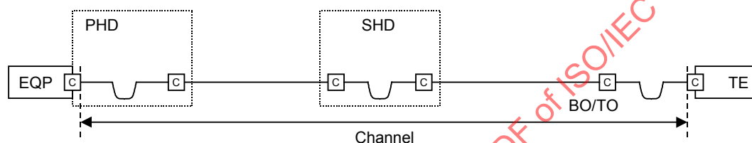
Figure 13 B – Model with four connections
