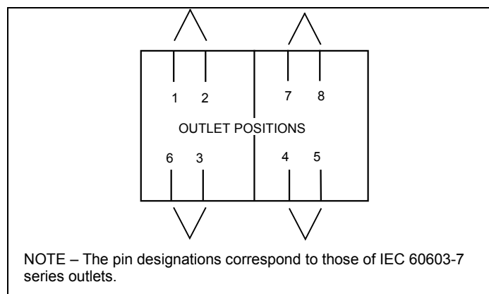
Figure 17 – Pin grouping assignments for 61076-3-104 outlet (front view)
