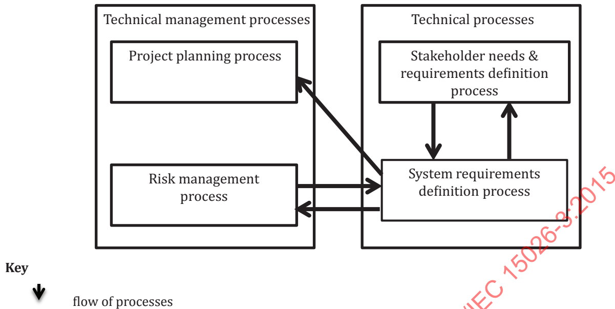
Figure 5 — Related processes in ISO/IEC/IEEE 15288 to the system integrity level determination process (informative)
