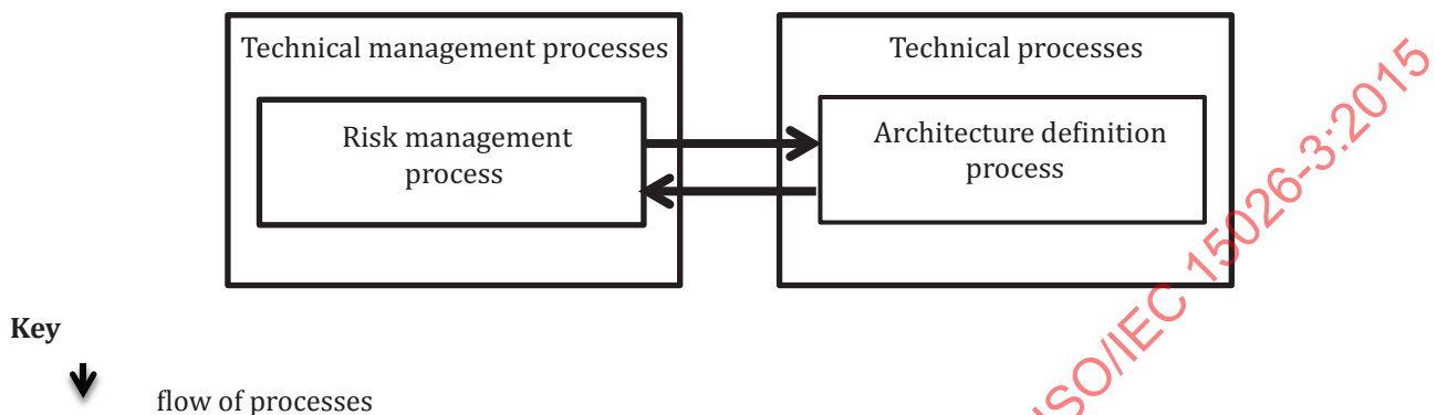
Figure 6 — Related processes in ISO/IEC/IEEE 15288 to the system element integrity level determination process (informative)
