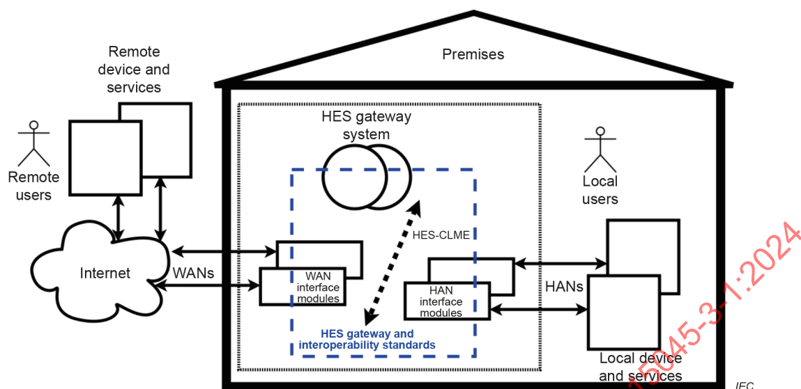
Figure 2 – HES gateway generalized architecture
