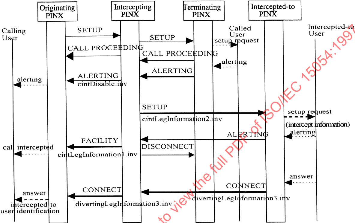
Figure B.2.1 - Message sequence for successful invocation of ANF-CINT using interception delayed procedures
