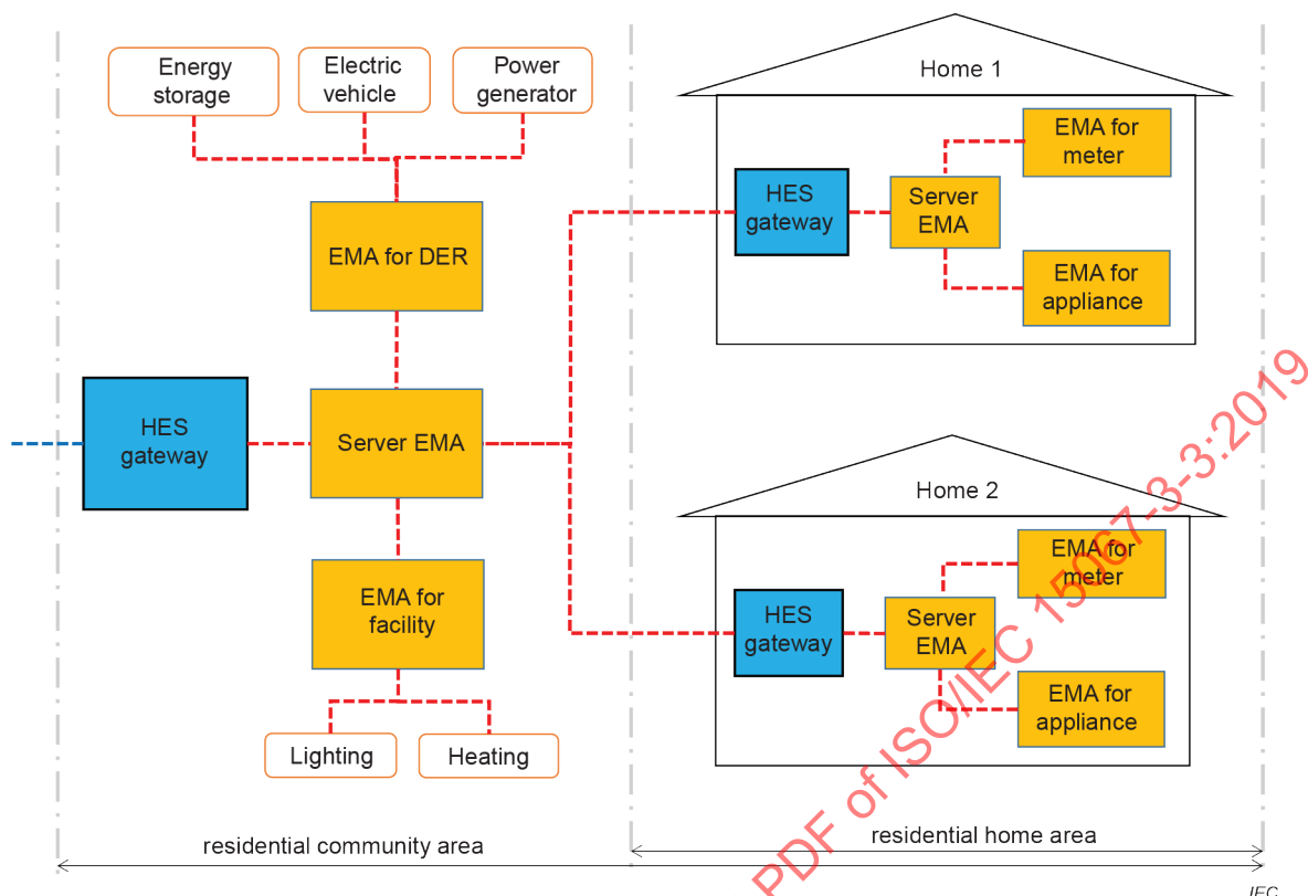
Figure A.2 – Example of local EMA topology model for a residential community
