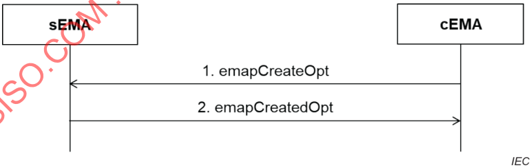
Figure 35 – Interaction diagram: Create opt
