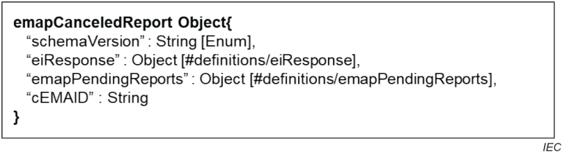
Figure 34 – emapCanceledReport simplified message format
