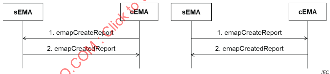
Figure 24 – Interaction diagram: Request report – Push operation
