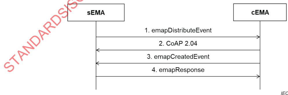
Figure 17 – Event interaction diagram – Push operation
