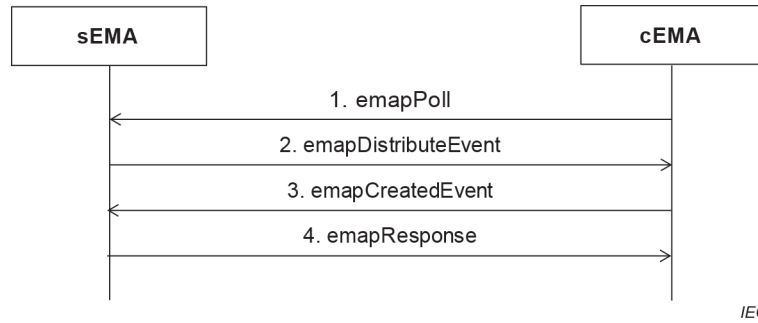
Figure 44 – Interaction diagram: Poll (emapDistributeEvent reply)
