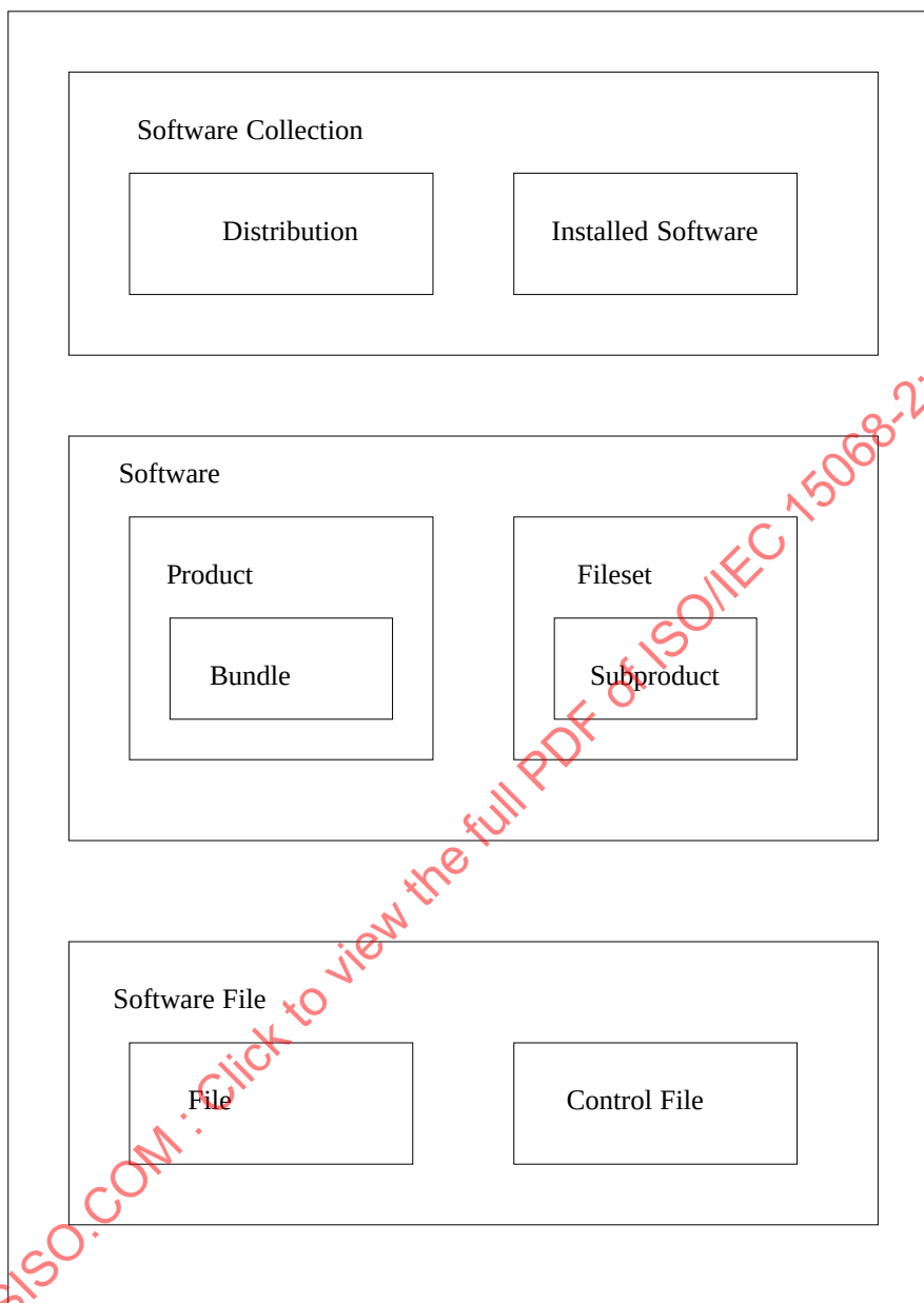
Figure B-4 – Software Object Inheritance
