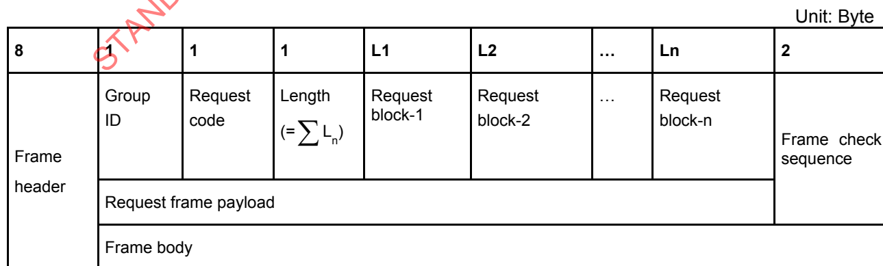
Figure 26 – Request frame format
