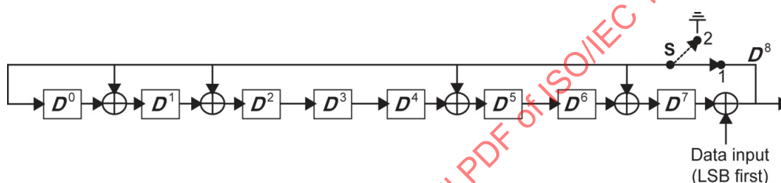
Figure 14 – Encoder of header check sequence
