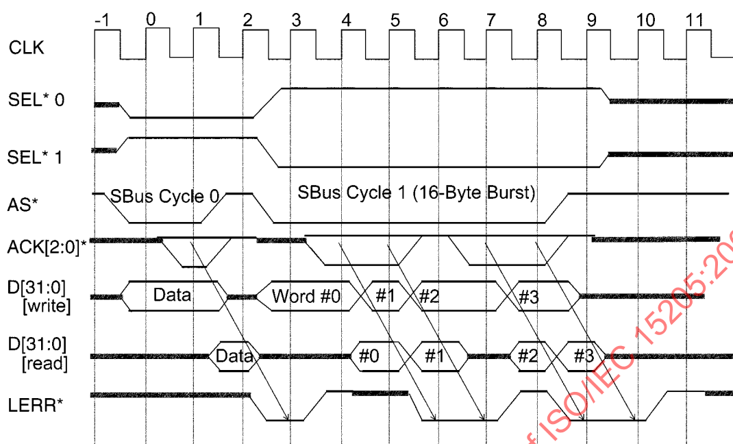
Figure 11 – Example of LERR* timing
