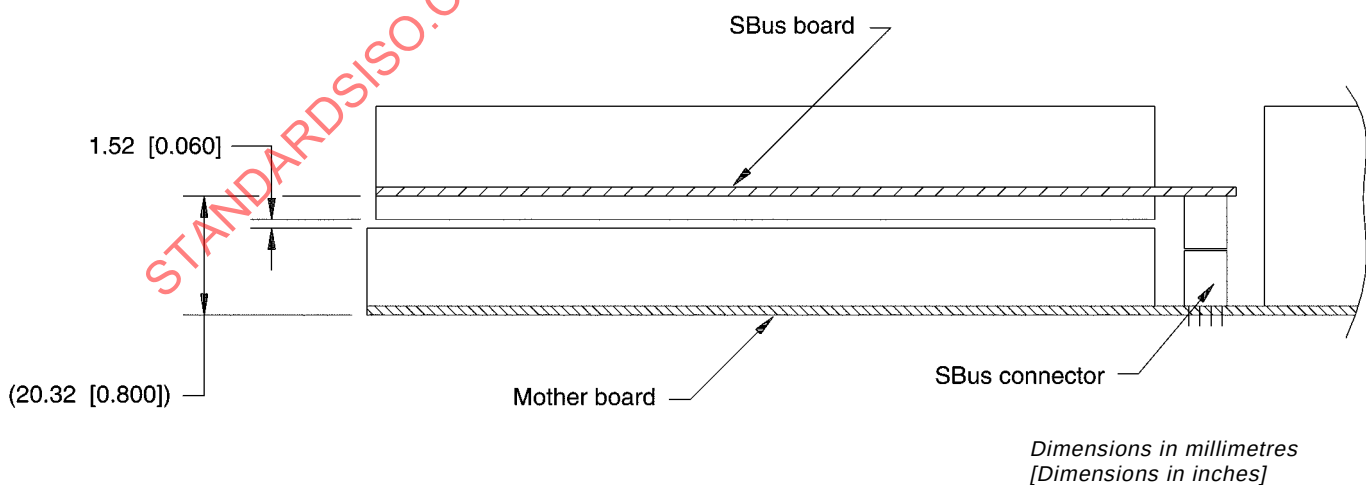
Figure 26 – Minimum component gap
