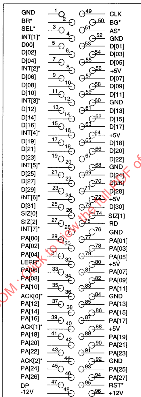
Figure 23 – Bus Slot signal location
