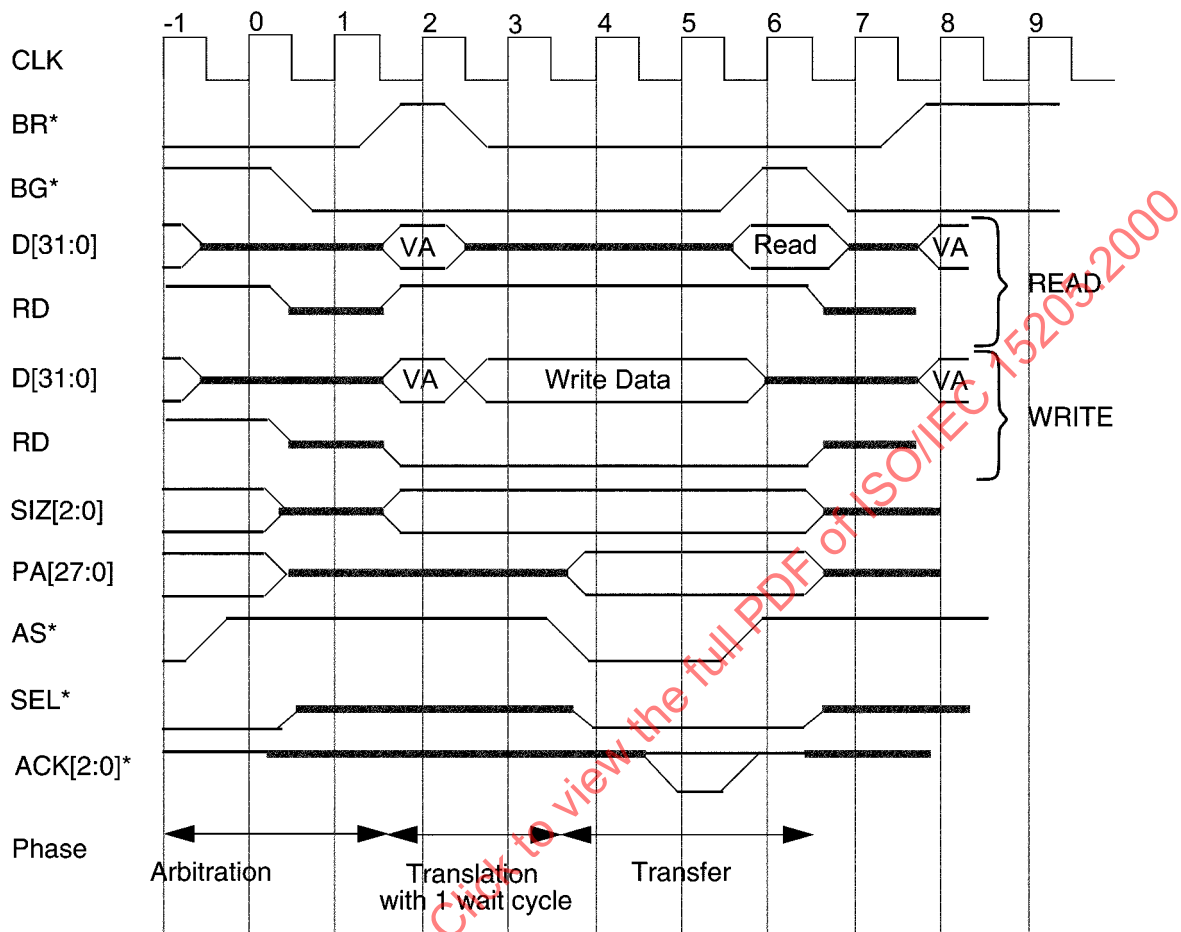
Figure 13 – Example of 32-bit symmetric SBus cycle
