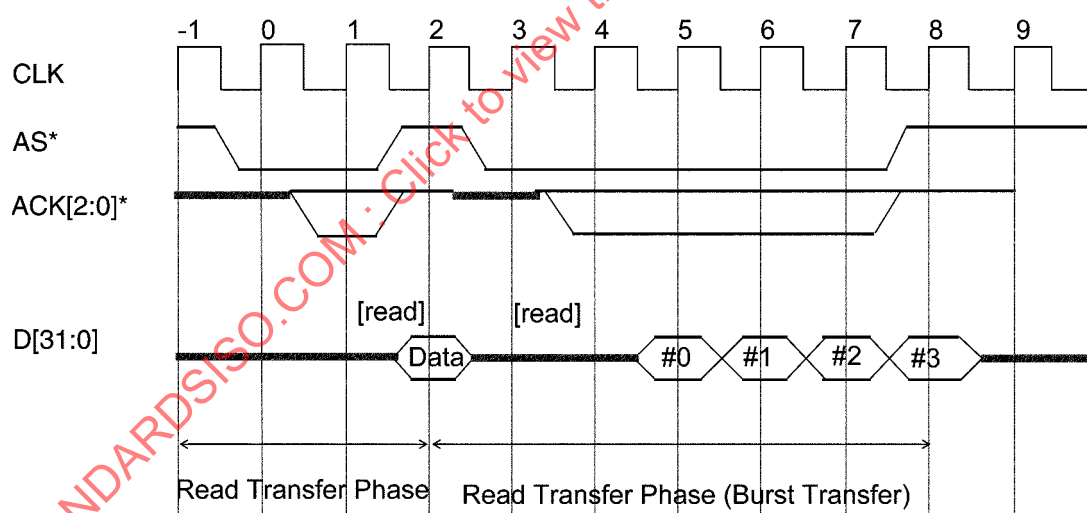
Figure 16 – Read following read, fastest case 32-bit asymmetric SBus cycle
