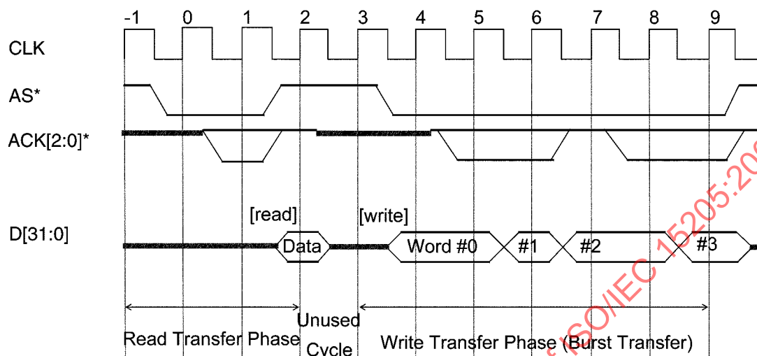
Figure 17 – Write following read, asymmetric SBus cycle
