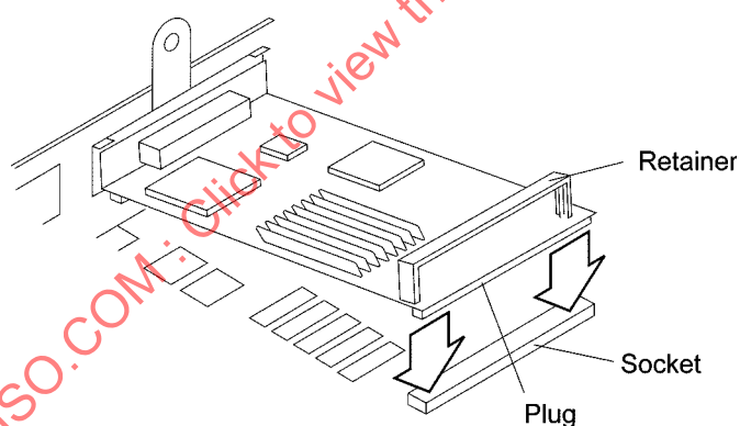
Figure 38 – SBus installation example
