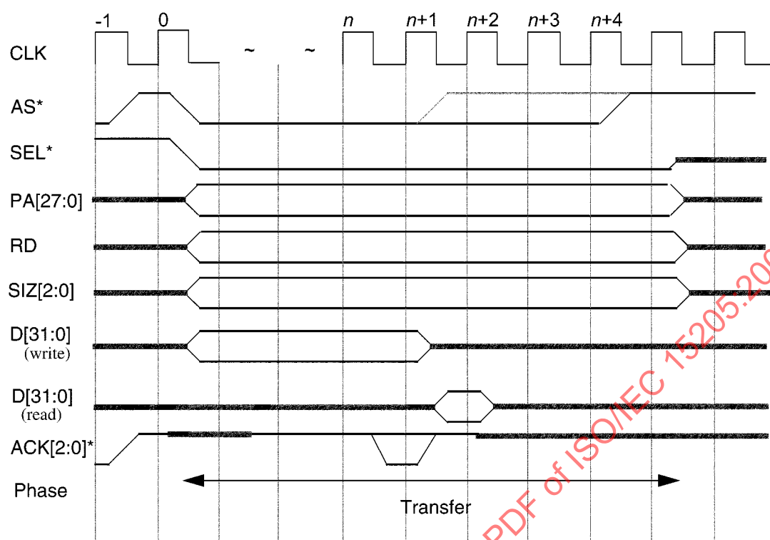
Figure 15 – 32-bit Transfer Phase, asymmetric SBus cycle
