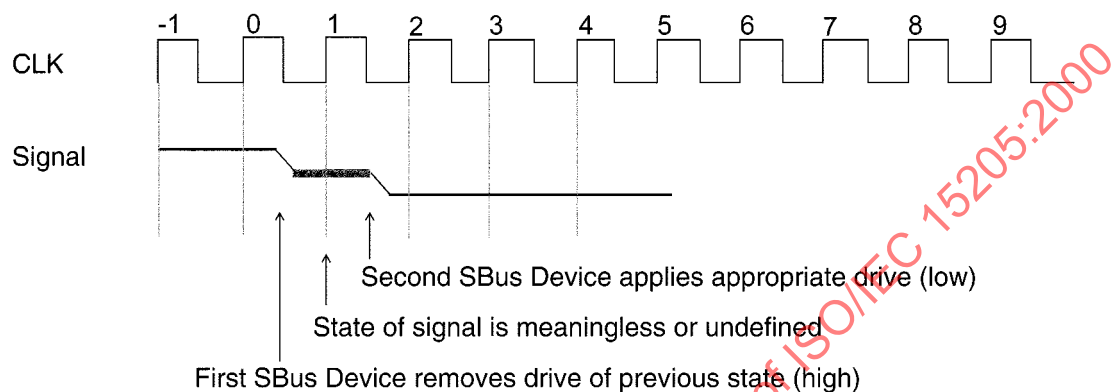
Figure 7 – Example of driver overlap protection
