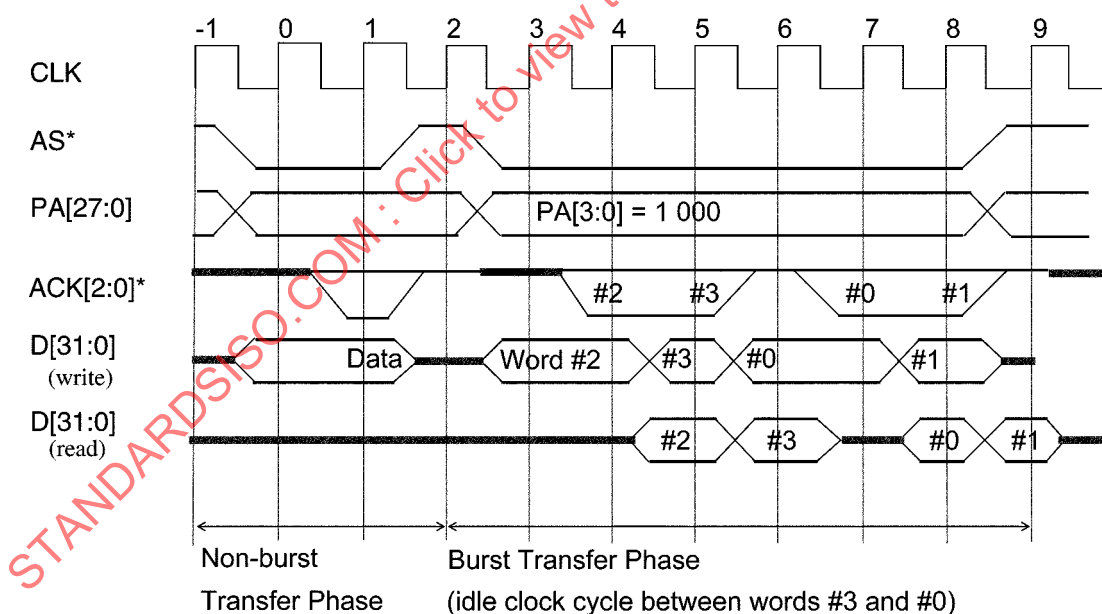
Figure 19 – Burst Transfer Phase, asymmetric cycles, 32-bit transfers, address wrapping
