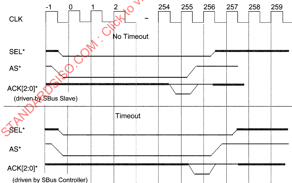
Figure 20 – Bus timeouts
