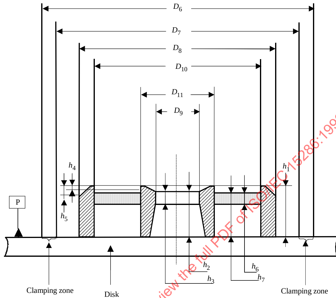
Figure 2 - Hub dimensions
