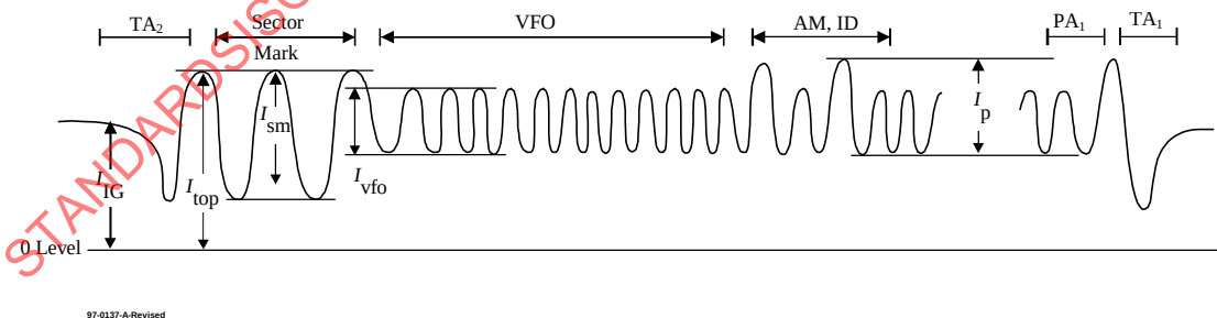
Figure 25c - Signals from Headers in Channel 1
