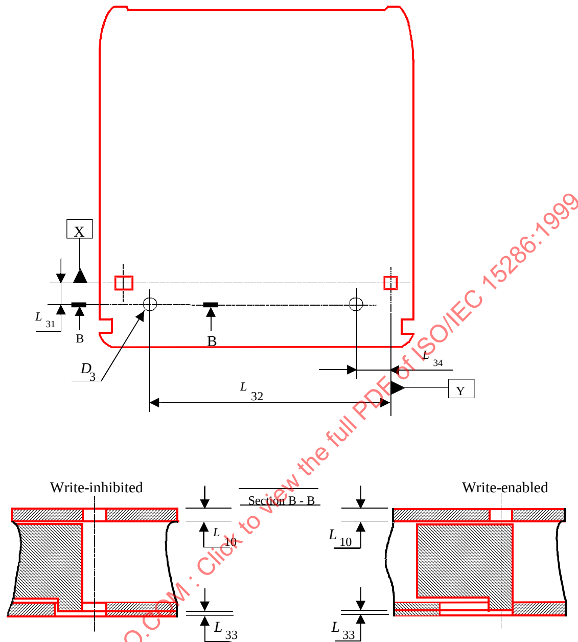
Figure 8 - Write-Inhibit holes
