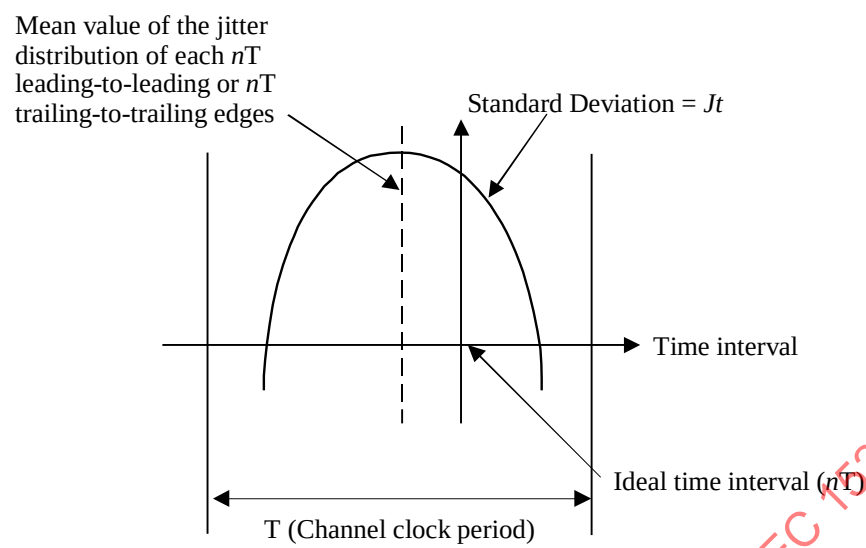
Figure J.1 - Measured distribution of timing jitter
