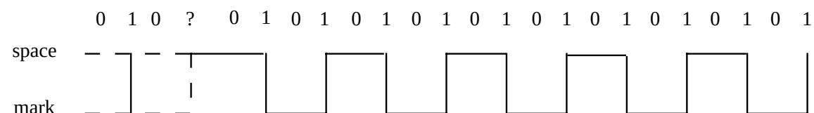
Figure 20 - Postamble pattern
