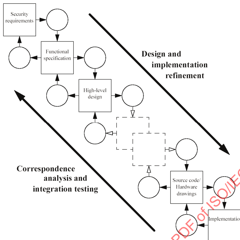
Figure 4 - TOE development model
