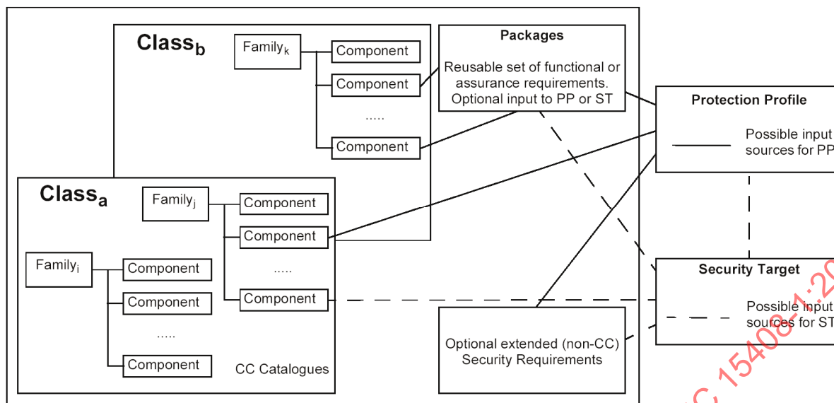
Figure 7 - Organisation and construction of requirements
