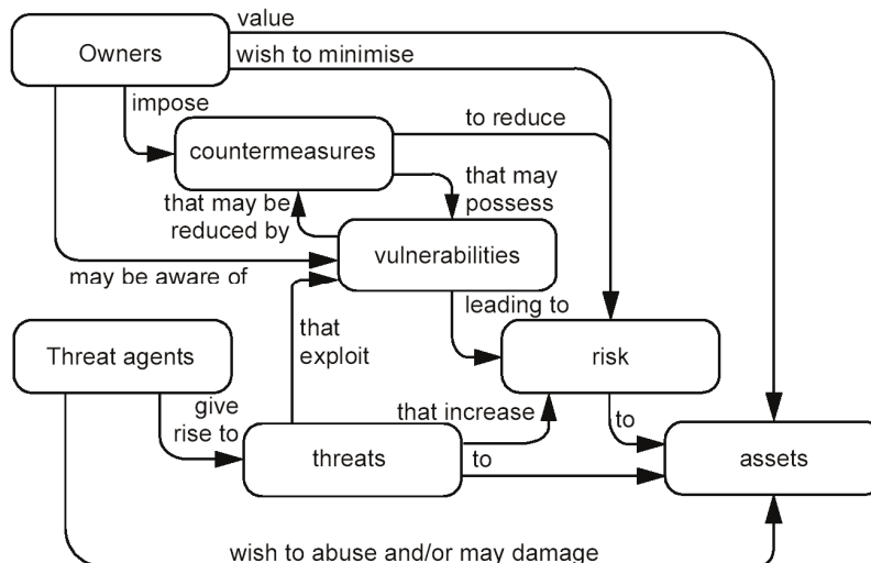
Figure 2 - Security concepts and relationships
