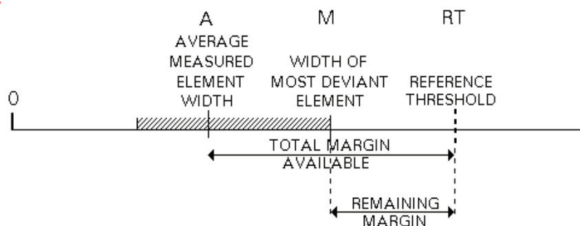
Figure 6 — Principle of decodability measurement
