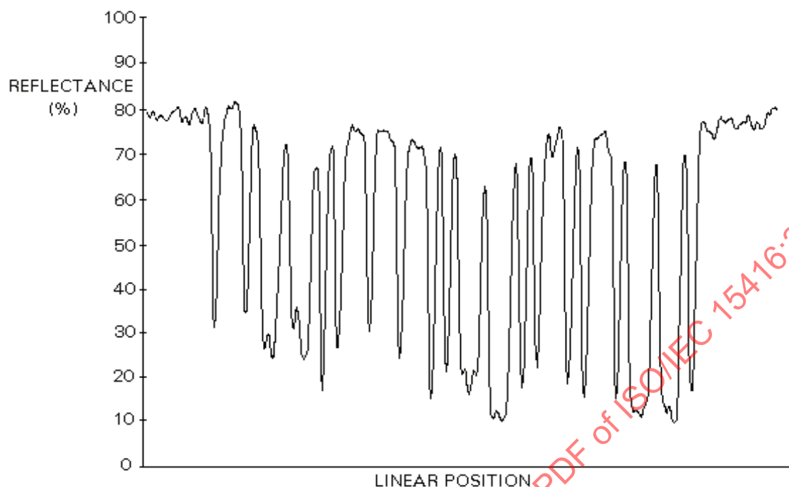
Figure 3 — Scan reflectance profile
