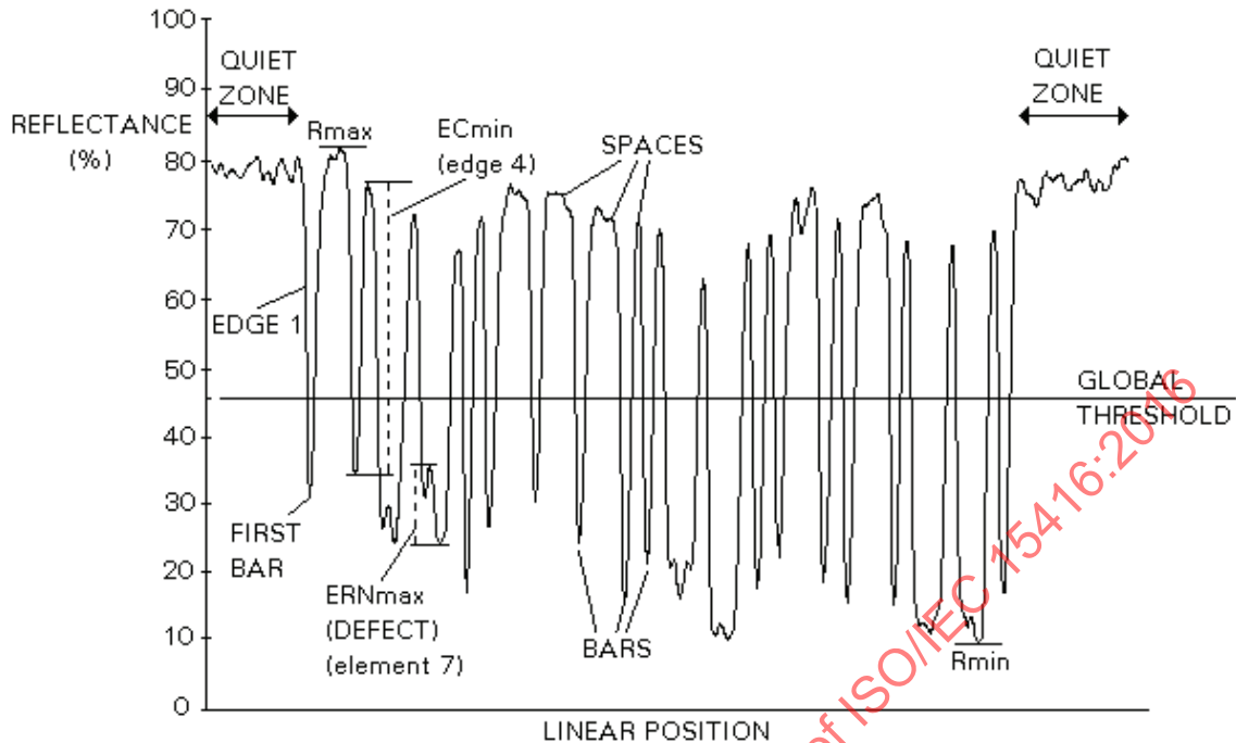
Figure 4 — Features of scan reflectance profile
