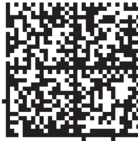
Figure A.3 — Test symbol with fixed pattern damage (data matrix)
