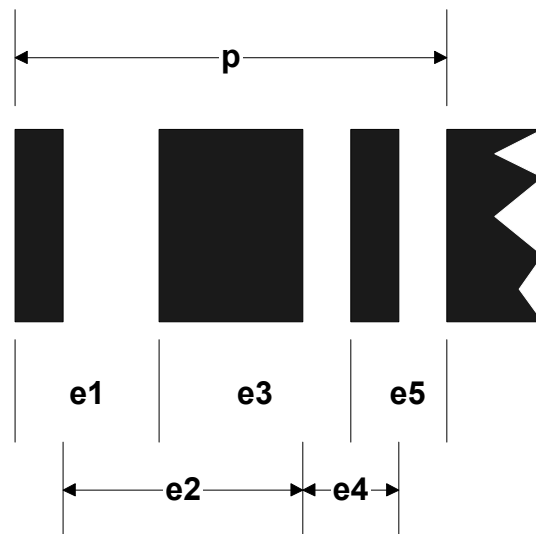
Figure K.1 — Decode Measurements
