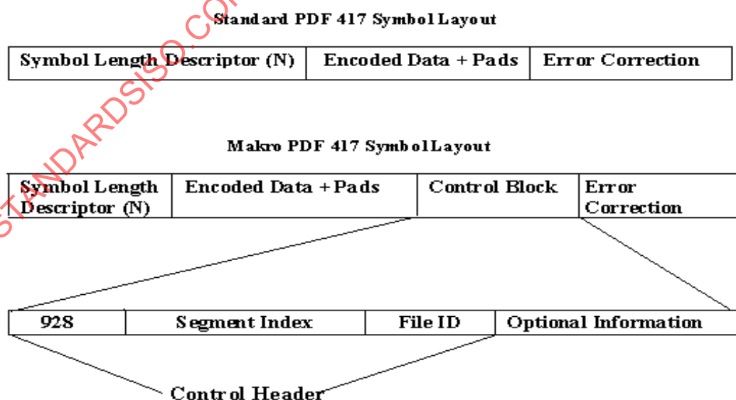
Figure H.1 — PDF417 Symbol Layouts
