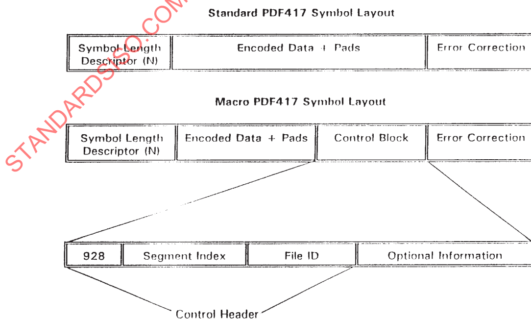
Figure H.1 — PDF417 Symbol Layouts
