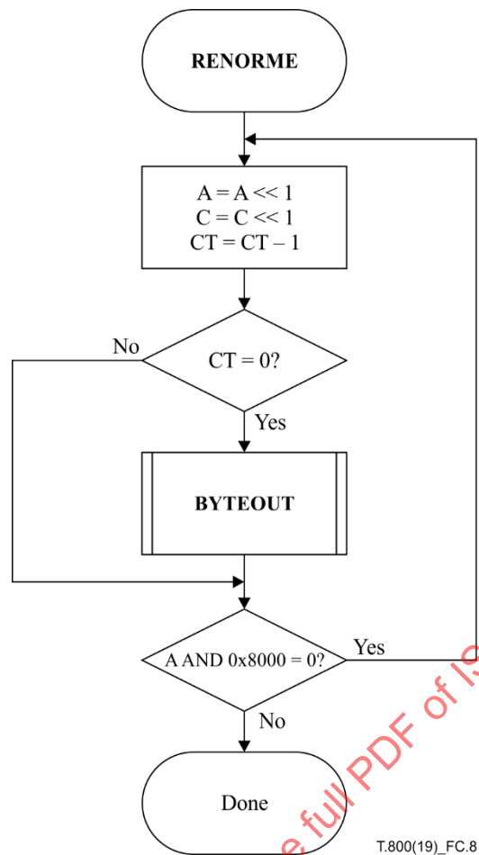
Figure C.8 – Encoder renormalization procedure
