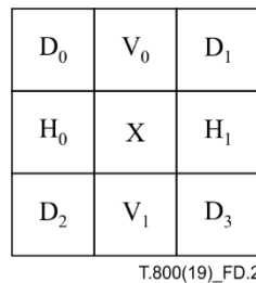
Figure D.2 – Neighbours states used to form the context
