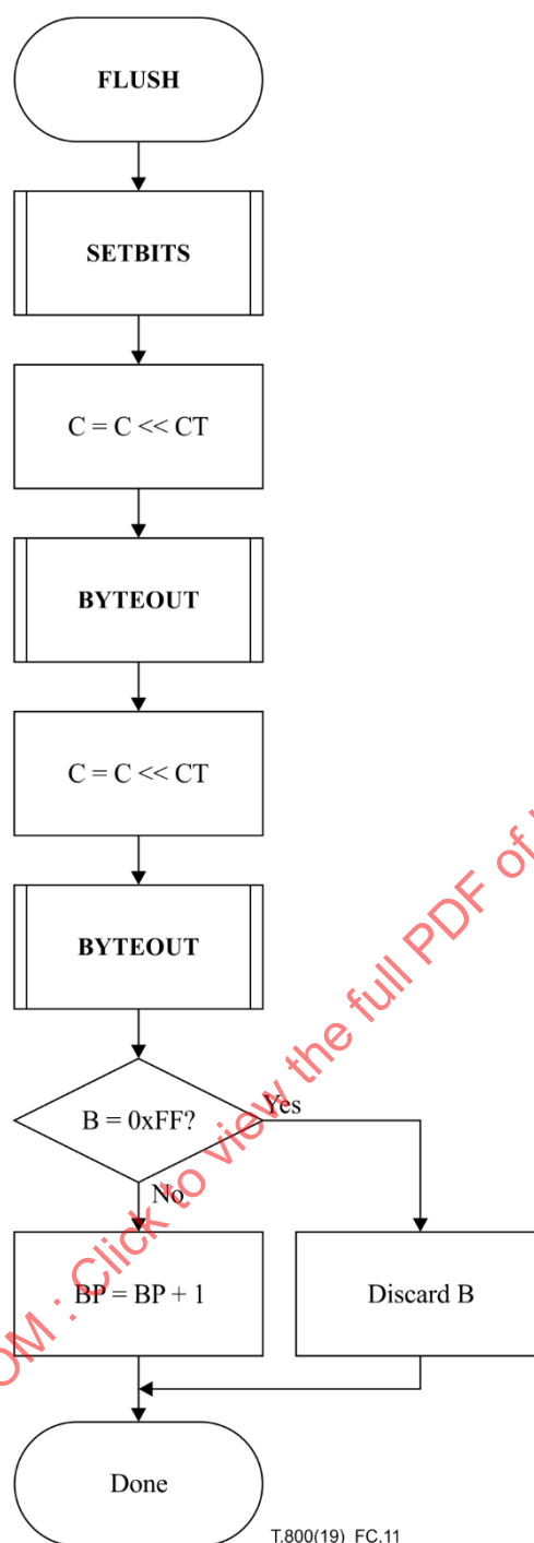
Figure C.11 – FLUSH procedure
