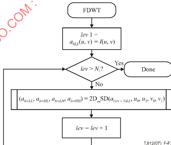
Figure F.3 – The FDWT procedure
