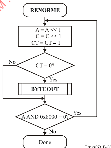
Figure C.8 – Encoder renormalization procedure
