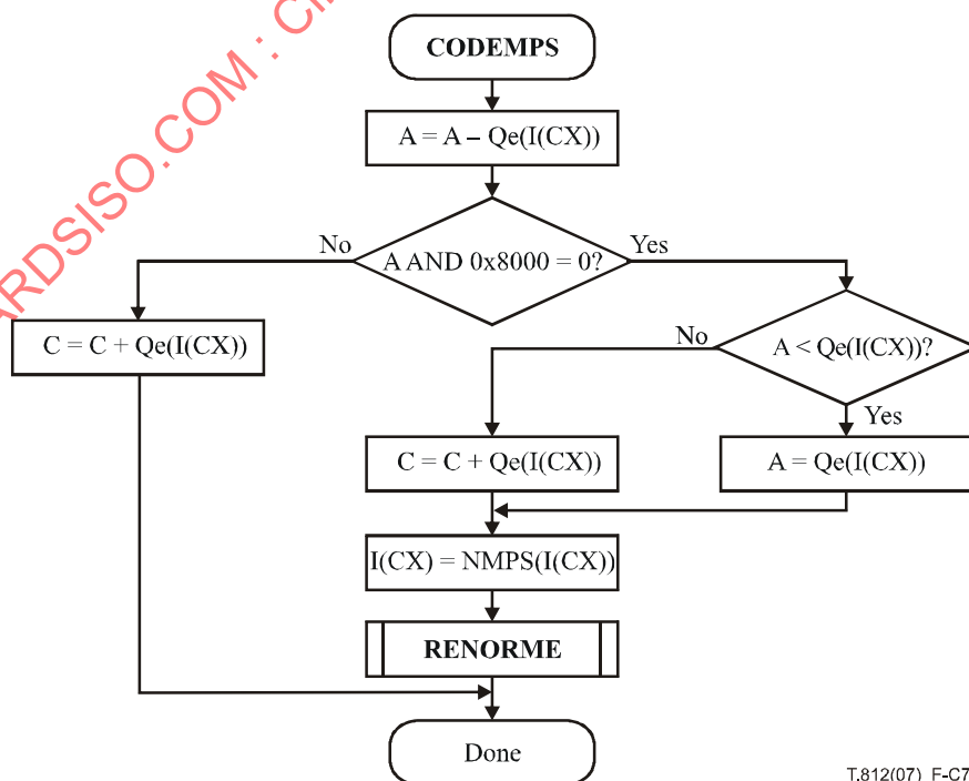
Figure C.7 – CODEMPS procedure with conditional MPS/LPS exchange
