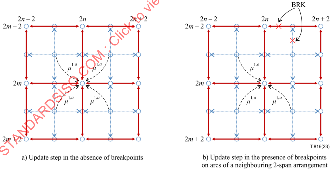
Figure 20 – Phase 1 update step for (even, even) location (2n, 2m)
