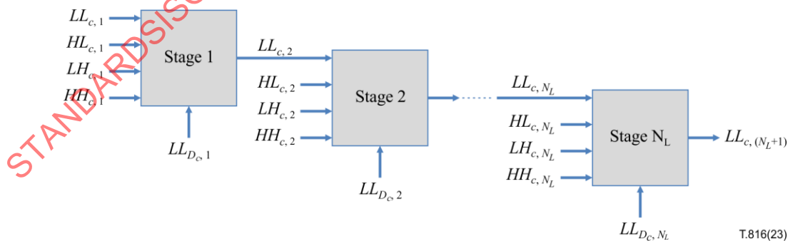
Figure 5 – Stages of the breakpoint dependent inverse discrete wavelet transform
