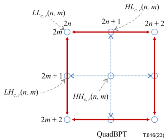
Figure 19 – Interleaving of sub-band coefficients to a quadrilateral grid for a given resolution r
