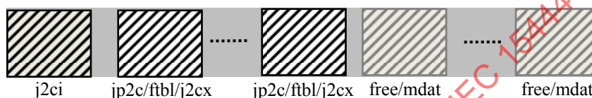
Figure M-44 – Organization of the contents of a Multiple Codestream box
