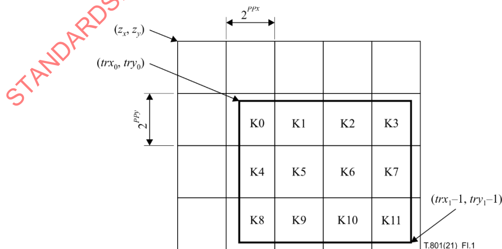
Figure I.1 – Precincts of one reduced resolution (modified Figure B.8 of Rec. ITU-T T.800 | ISO/IEC 15444-1)
