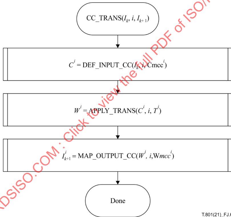
Figure J.6 – Procedure CC_TRANS
