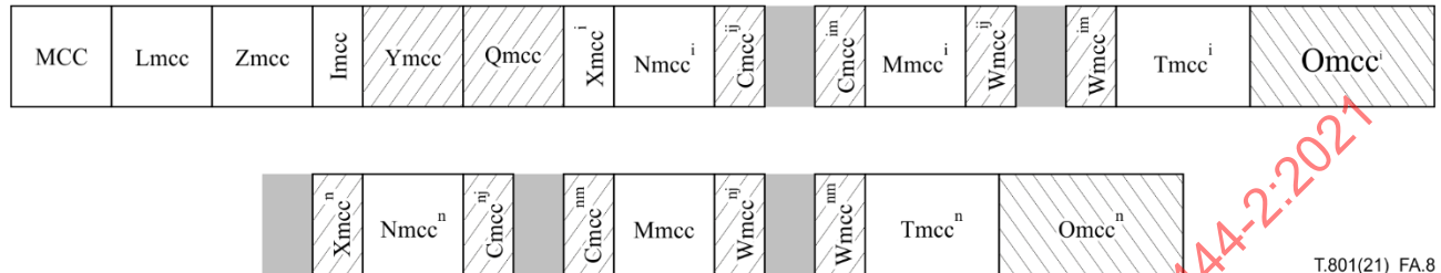
Figure A.8 – Multiple component collection syntax
