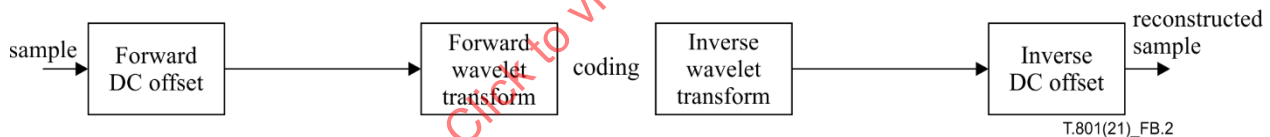
Figure B.2 – Placement of the DC offset without multiple component transformation
