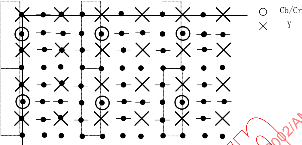
Figure C.3 — 4:2:0 format (co-sited)
