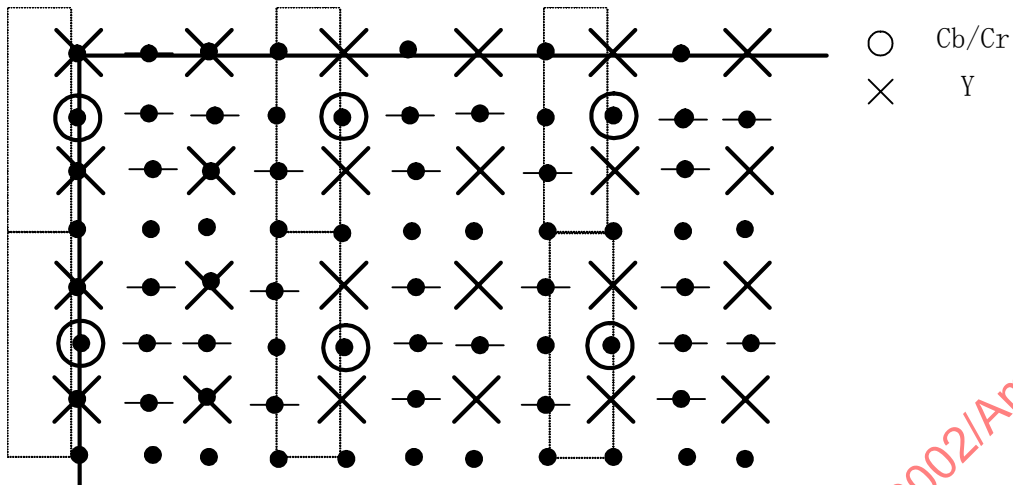
Figure C.3 — 4:2:0 format (co-sited)
