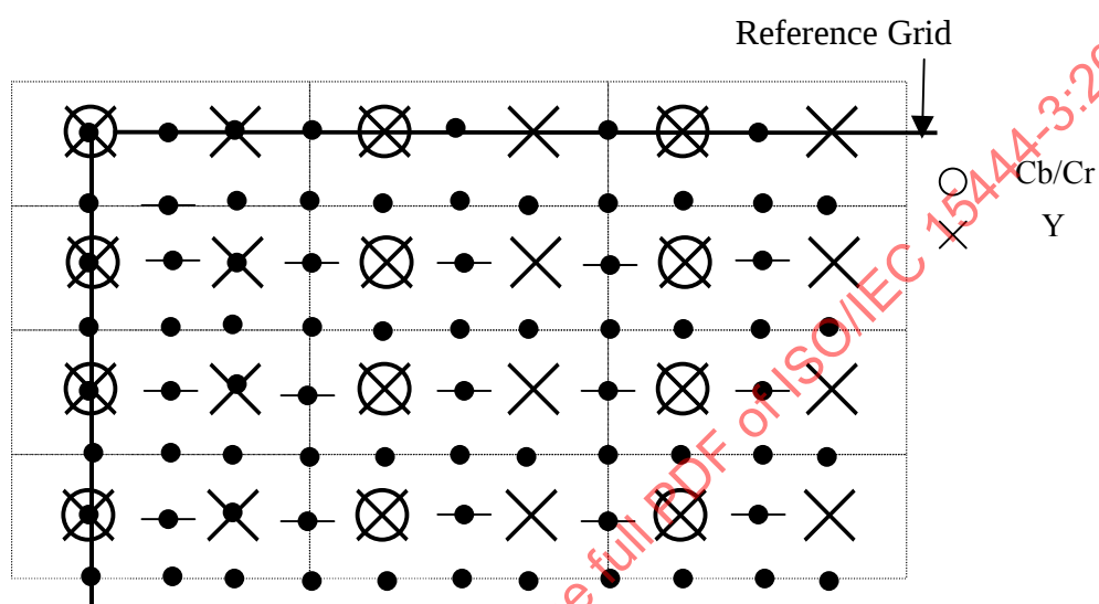
Figure C.1 — 4:2:2 format (co-sited)
