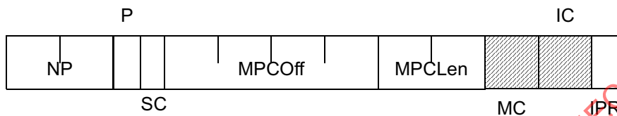
Figure B-1 Organization of the contents of a Compound Image Header box
