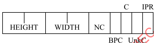
Figure B-20 Organization of the contents of an Image Header box
