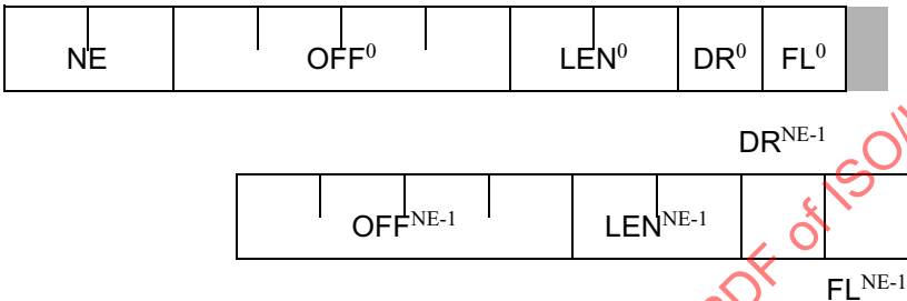
Figure B-5 Organization of the contents of a Page Table box
