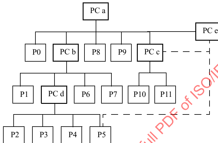
Figure 2 — Example of page collections and pages (Informative)
