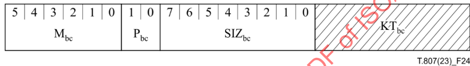
Figure 24 – Block cipher template syntax
