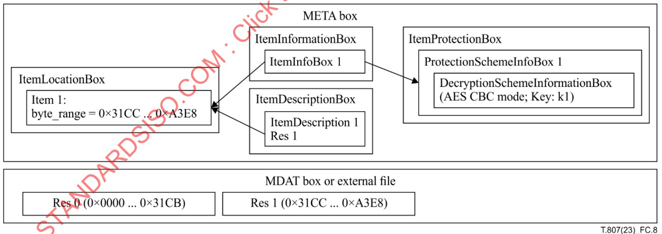
Figure C.8 – Example 2: Secure transcoding to lower resolution (discarding resolution 2)
