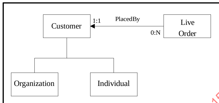
Figure 4 – Example of CDIF graphical notation
