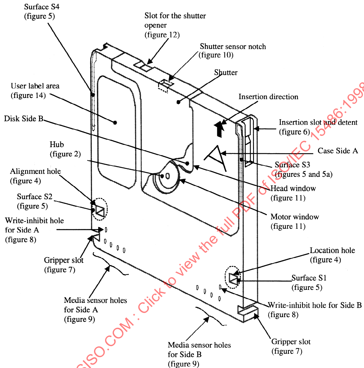
Figure 3 - Case
