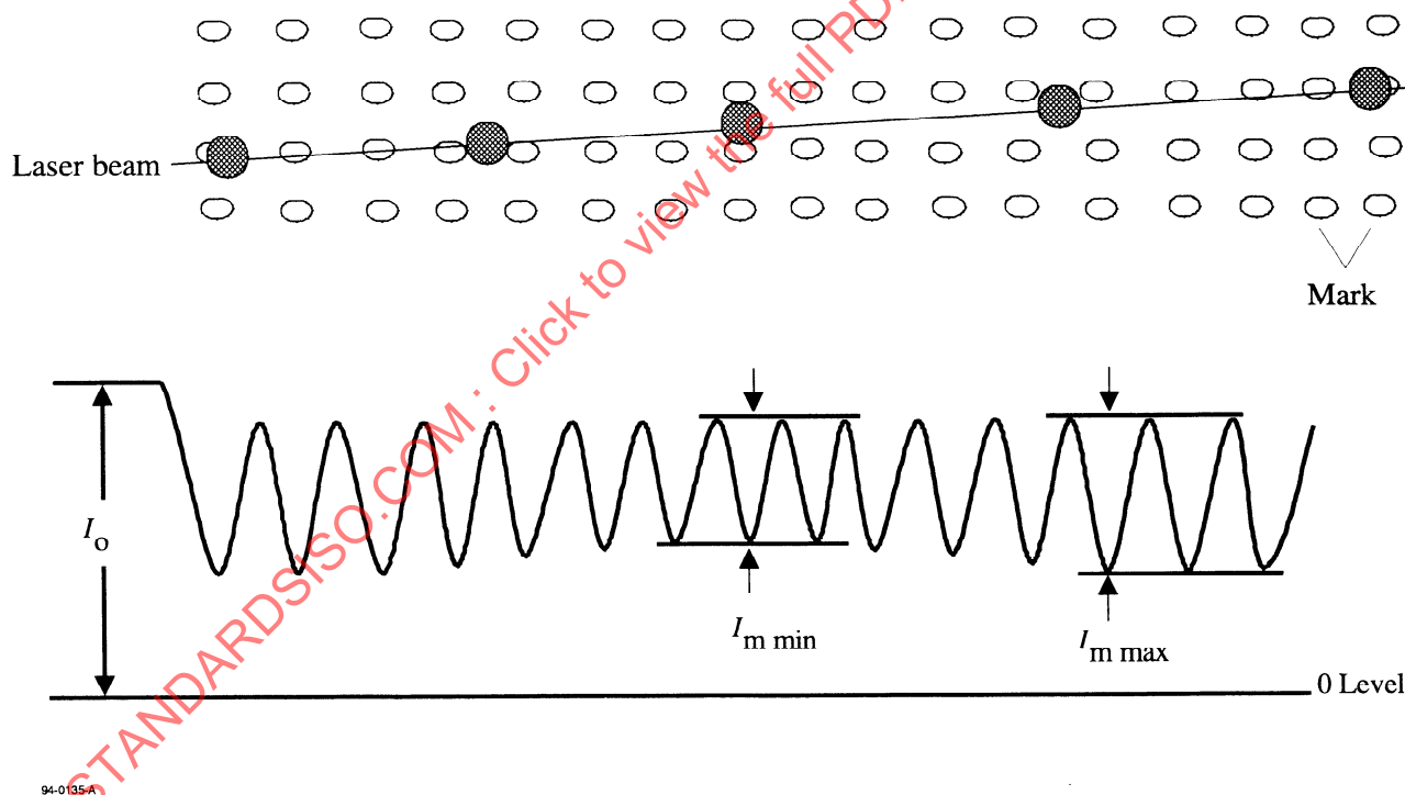
Figure 24 - Path of the laser beam when crossing tracks and the resulting PEP signals
