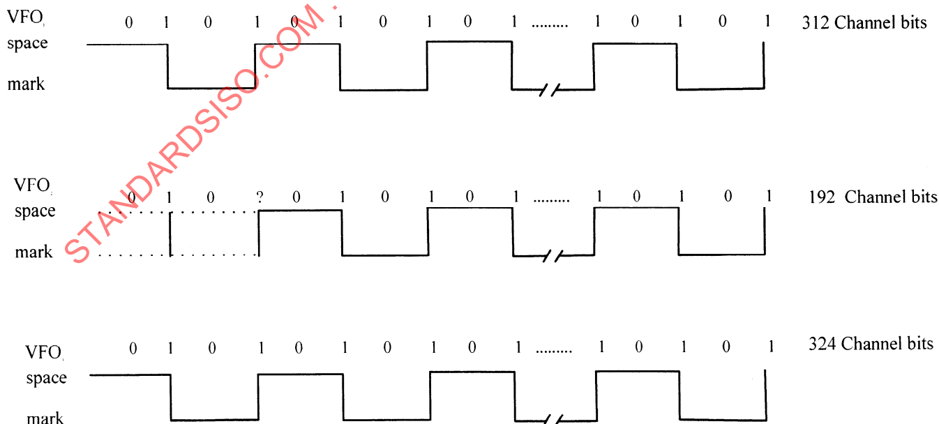
Figure 17 - VFO Field Patterns
