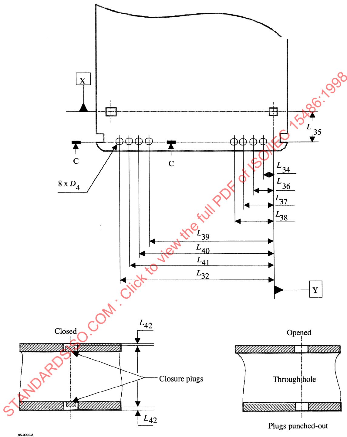
Figure 9 - Media ID sensor holes
