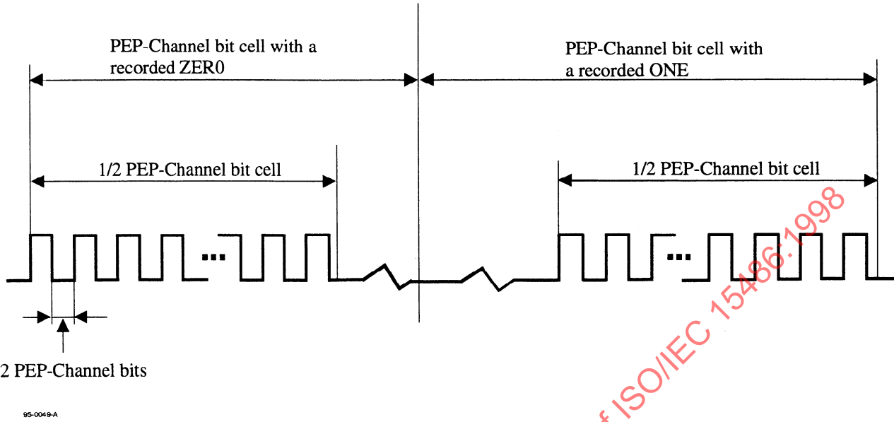
Figure 20 - Example of phase-encoded modulation in the PEP Zone
