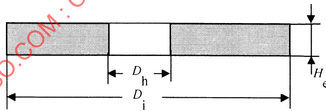
Figure D.2 - Calibration plate of the test device
