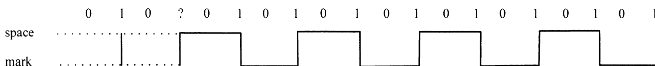
Figure 18 - Postamble pattern
