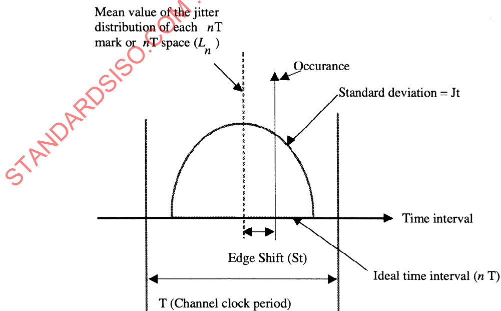
Figure J.1 - Measured timing distribution yielding Jitter J(t) and Edge Shift S(t)
