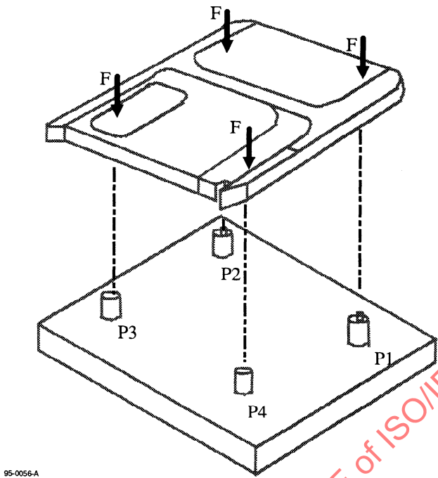
Figure C.1 - Compliance gauge
