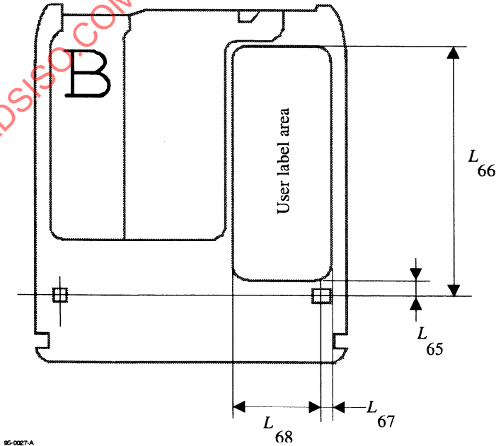
Figure 14c - User label on Side B
