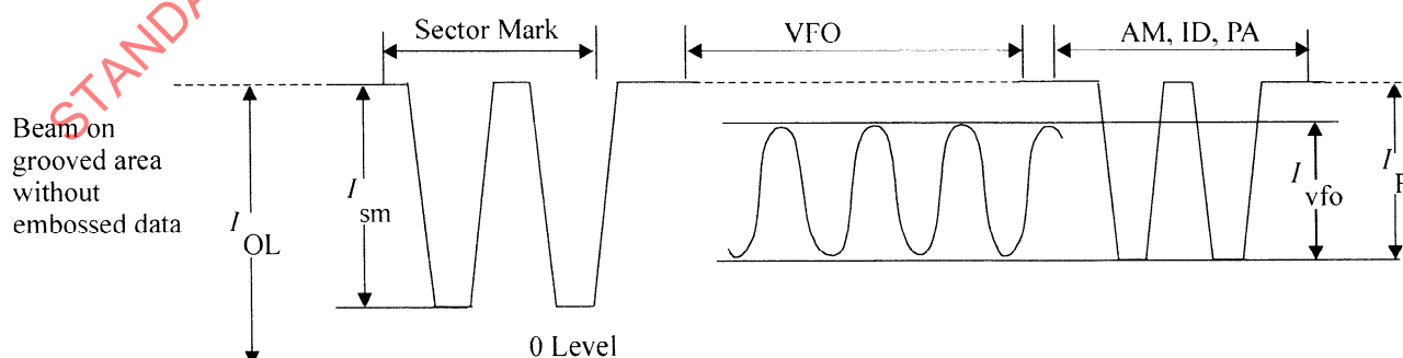
Figure 23b - Signals from grooves in Channel 1
