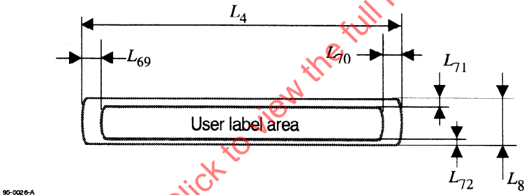
Figure 14b - User label area on bottom surface
