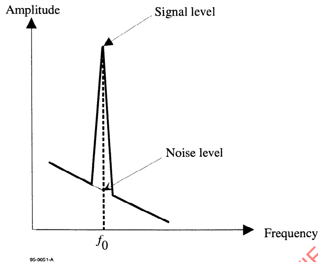
Figure 26 - Amplitude versus frequency for the WORM-optical signal
