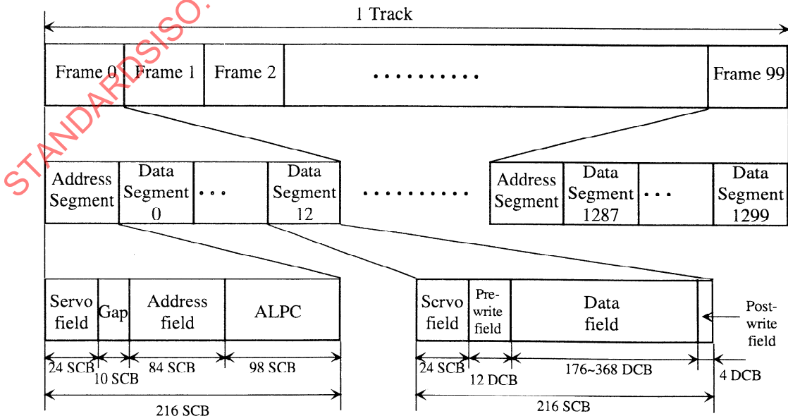
Figure 15 - Track layout
