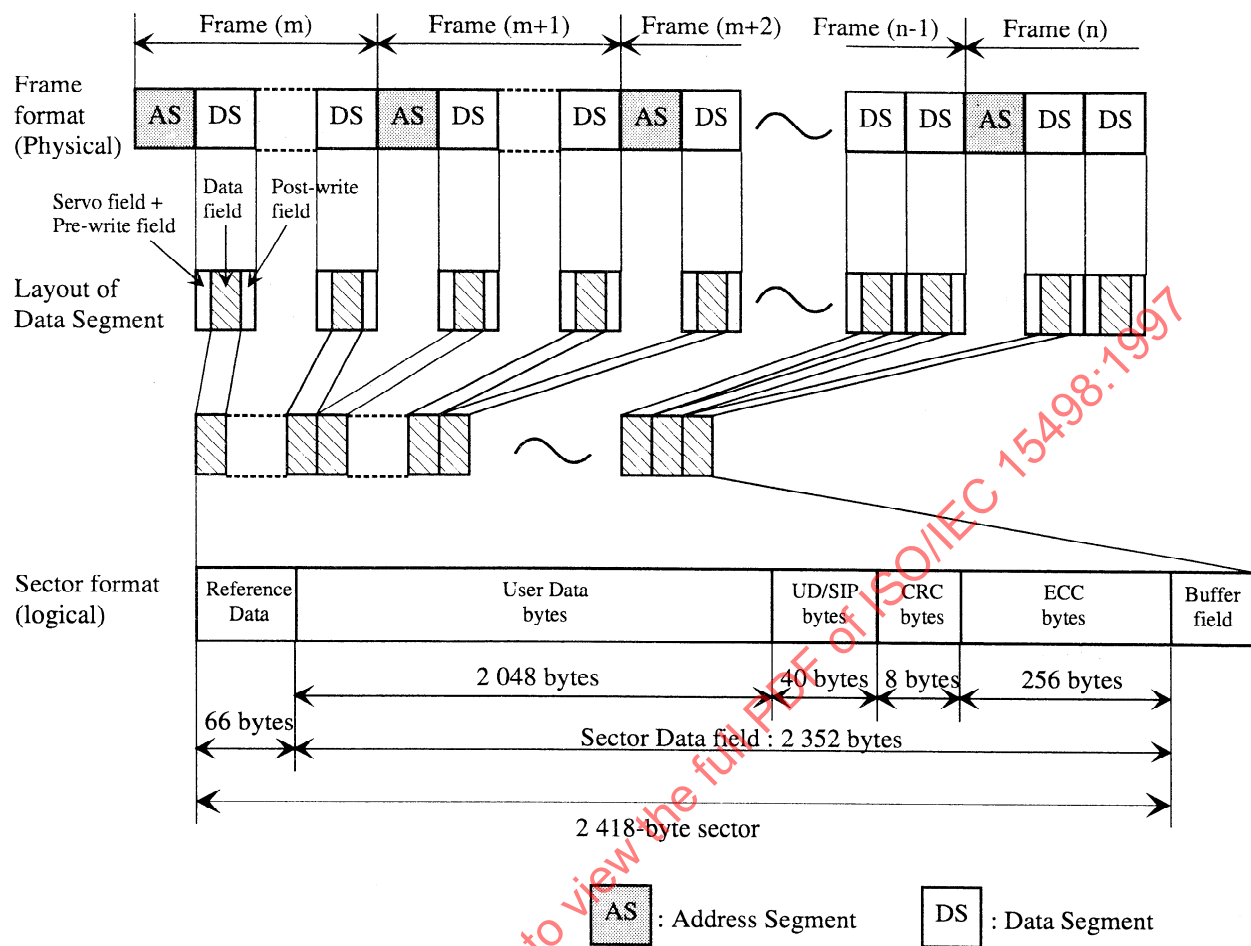
Figure 19 - Sector format
