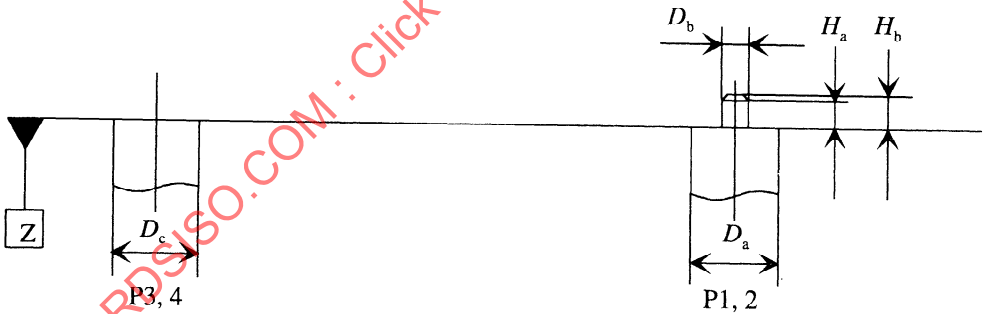
Figure B.2 - Detail of posts
