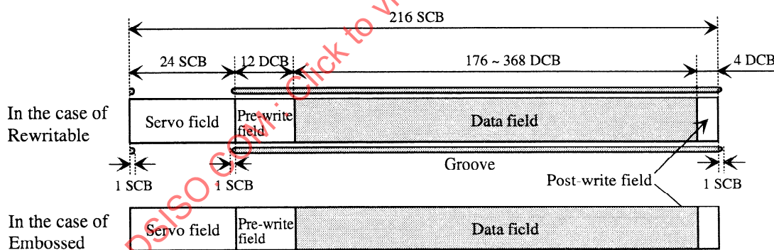
Figure 17 - Layout of the Data Segment
