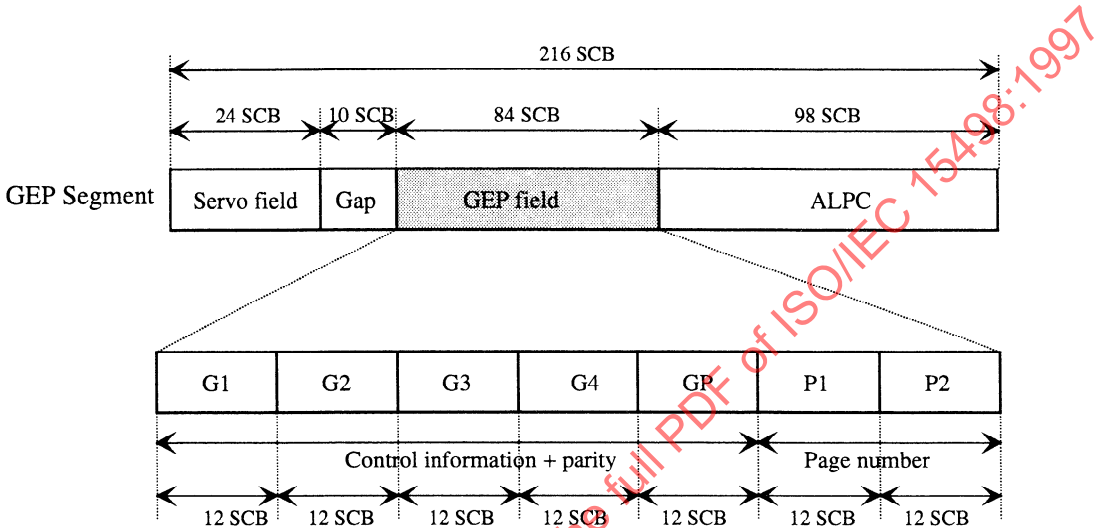
Figure 22 - Layout of the GEP Zone
