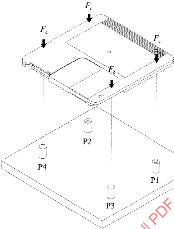
Figure B.1 - Compliance gauge
