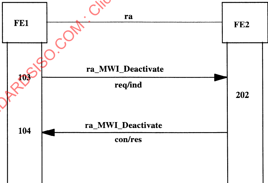
Figure 4 - Information flow sequence for deactivation of SS-MWI
