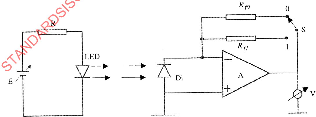
Figure B.2 - Measuring circuitry
