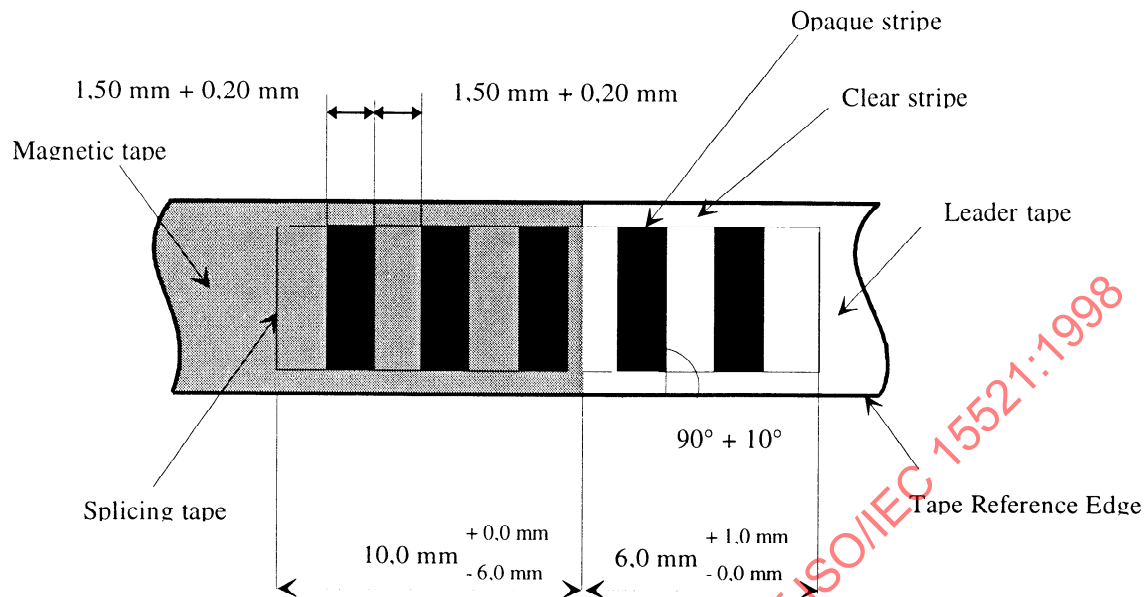
Figure 29 - Splicing tape at PBOT
