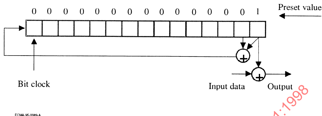
Figure 33 - Shift register
