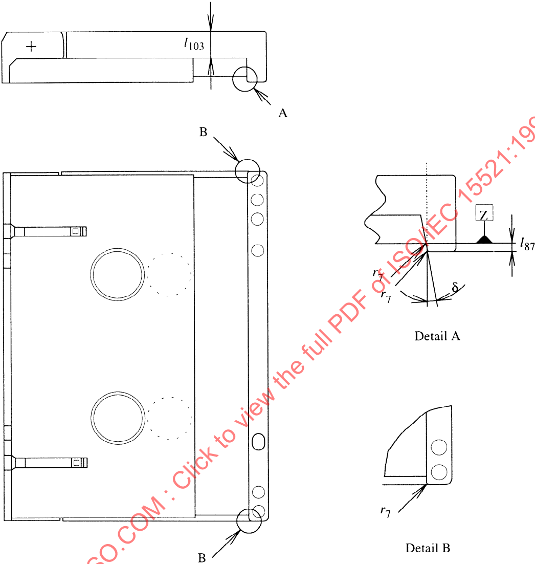
Figure 23 - Bottom side, both corners
