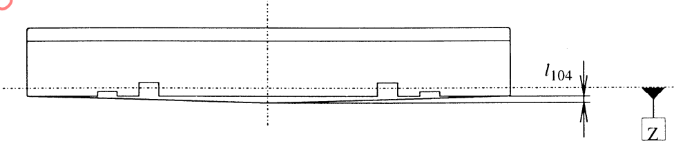
Figure 24 - Front side, slider bowdown
