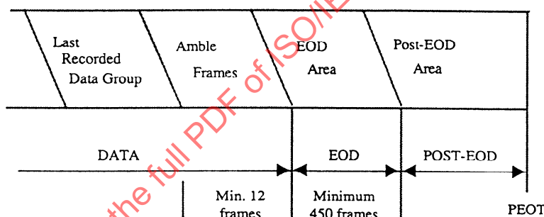
Figure 54 - Layout of a Single Data Space tape
