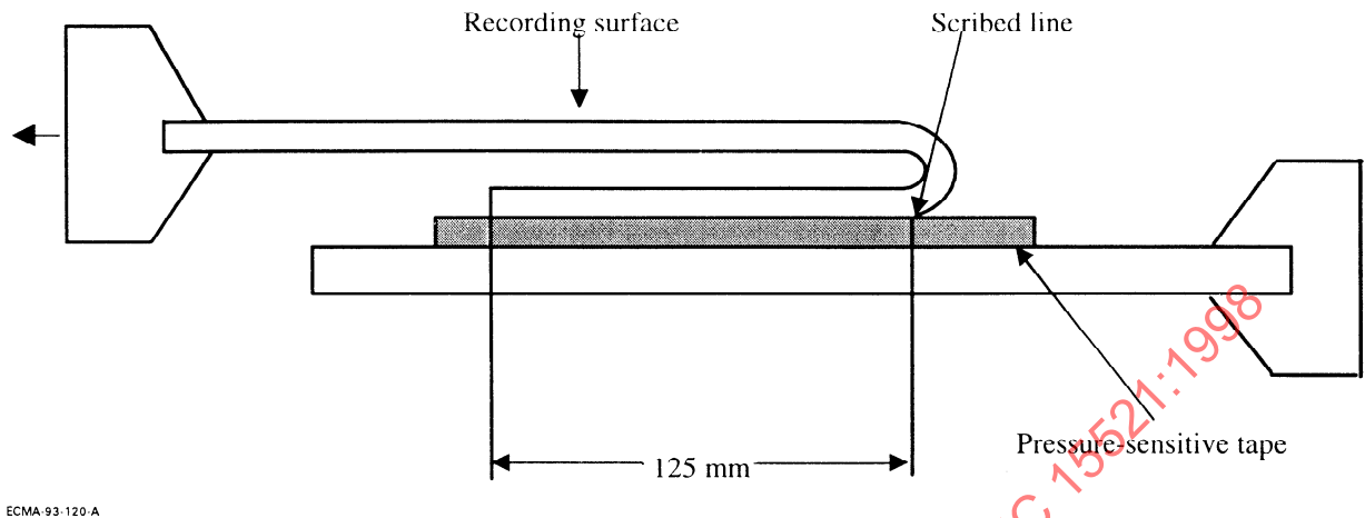
Figure 27 - Measurement of coating adhesion
