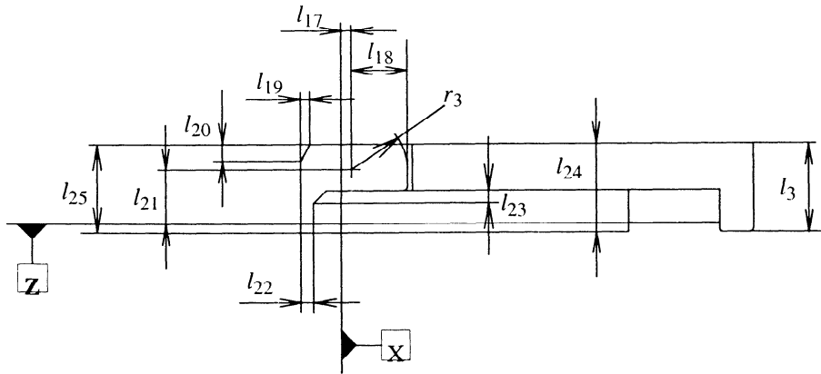
Figure 7 - Left side, lid closed
