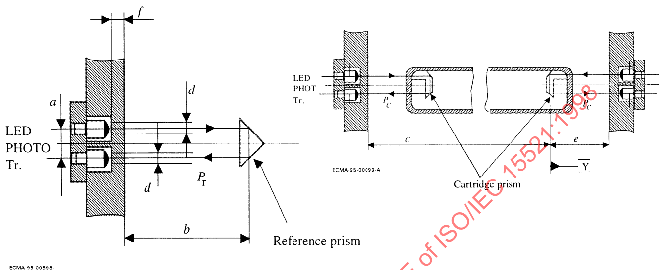
Figure A.1 - Reference prism
