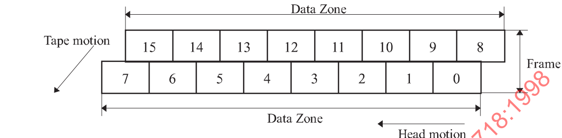
Figure 31 - Arrangement of Information Blocks in original or even times rewritten Frame
