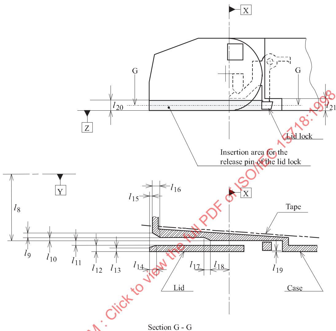
Figure 14 - Lid release insertion channel
