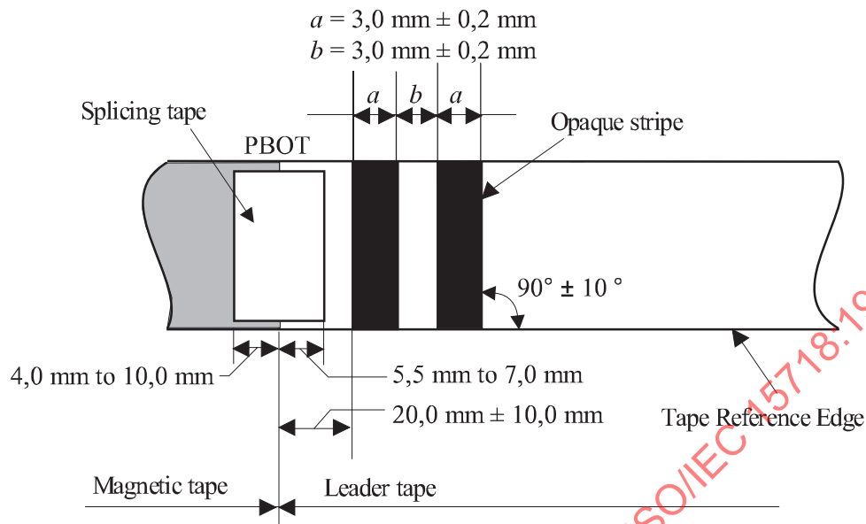
Figure 27 - Leader tape at PBOT
