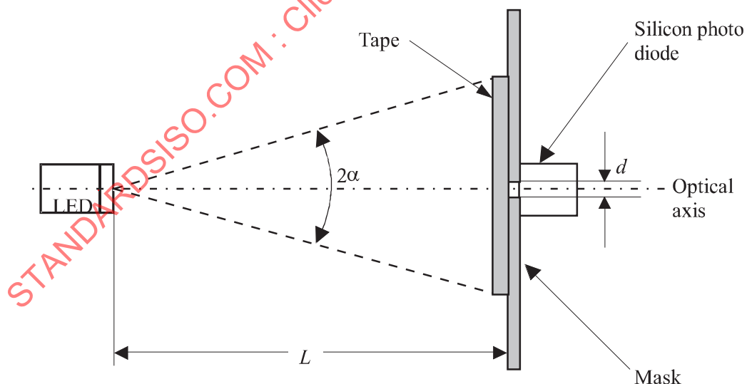
Figure A.1 - Optical arrangement
