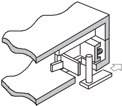
Figure 16 - Reel lock and release
