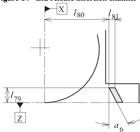
Figure 14 - Lid release insertion channel
