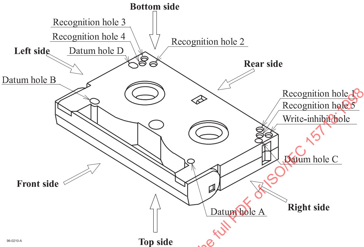
Figure 2 - Tape cartridge assembly bottom view, lid closed
