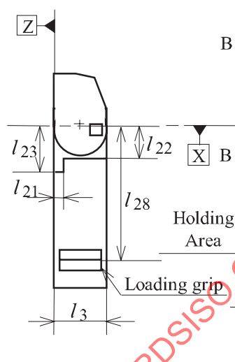
Figure 5 - Left side, lid closed
