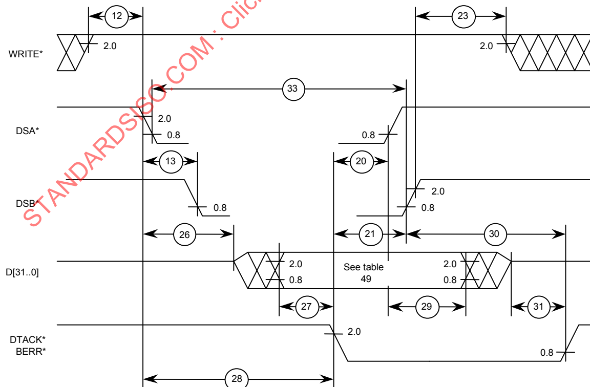
Figure 67 – Interrupt handler – Status/ID transfer timing double-byte and quad-byte interrupt acknowledge cycles
