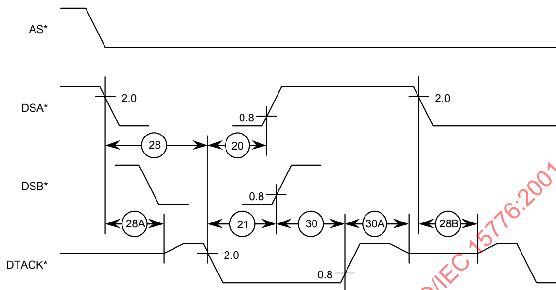
Figure 38 – Rescinding DTACK timing
