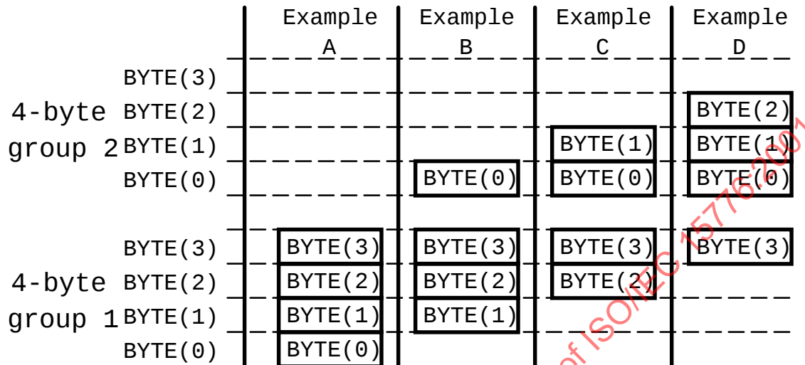
Figure 9 – Four ways in which 32 bits of data might be stored in memory
