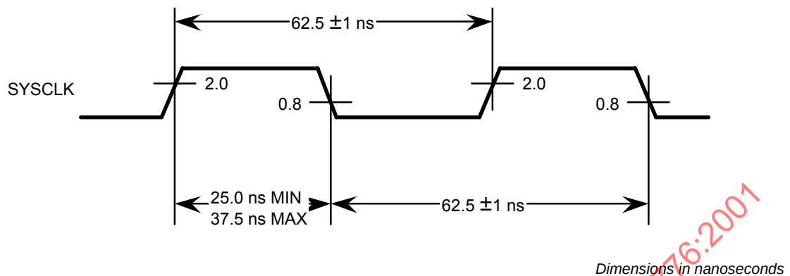
Figure 72 – System clock driver timing
