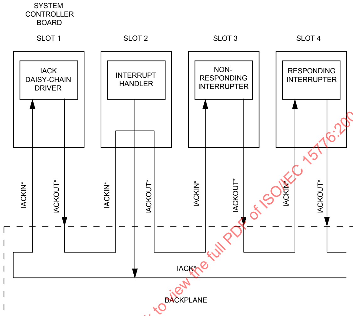
Figure 50 – IACKIN*/IACKOUT* DAISY-CHAIN
