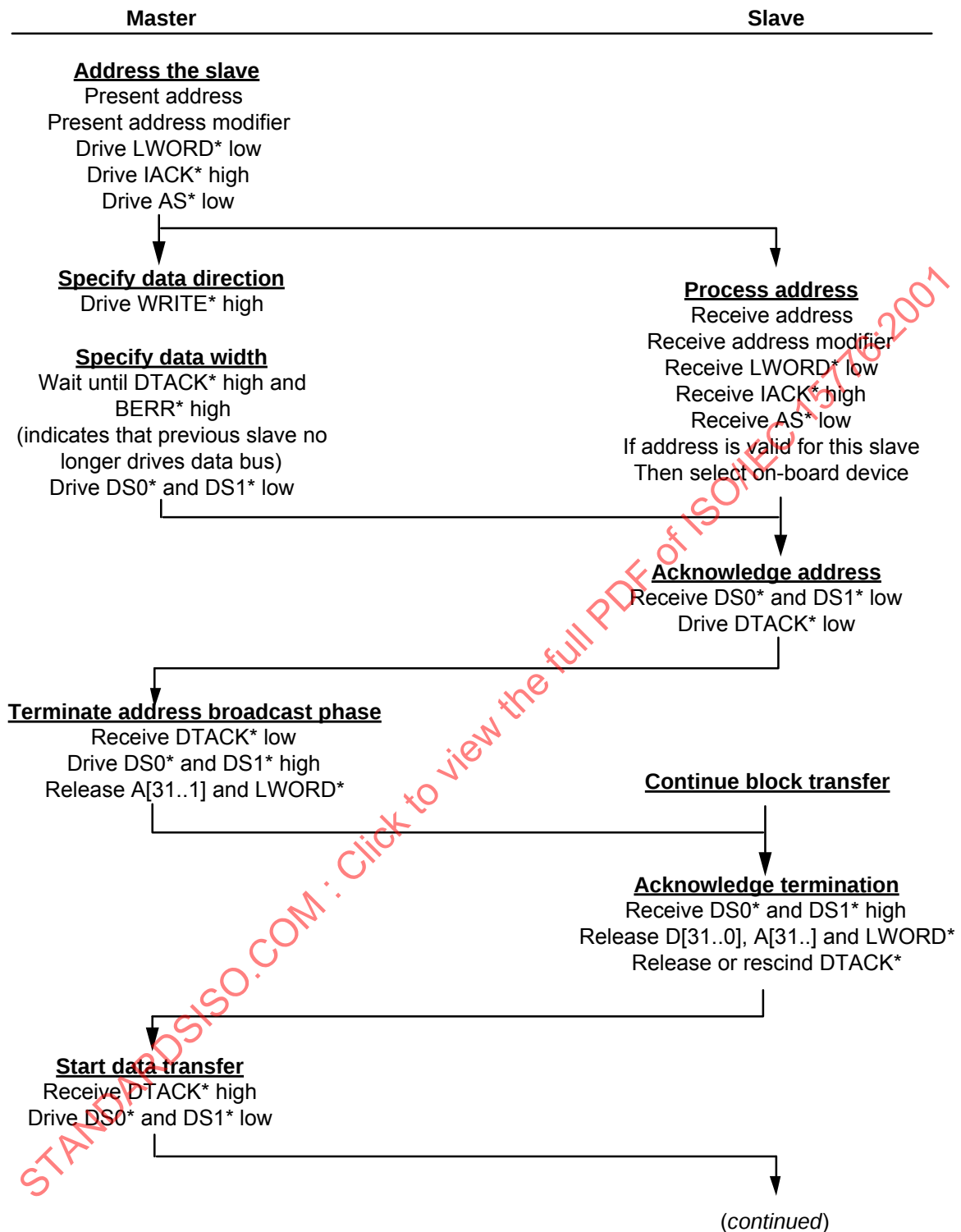
Figure 15 – Example of eight-byte block read cycle
