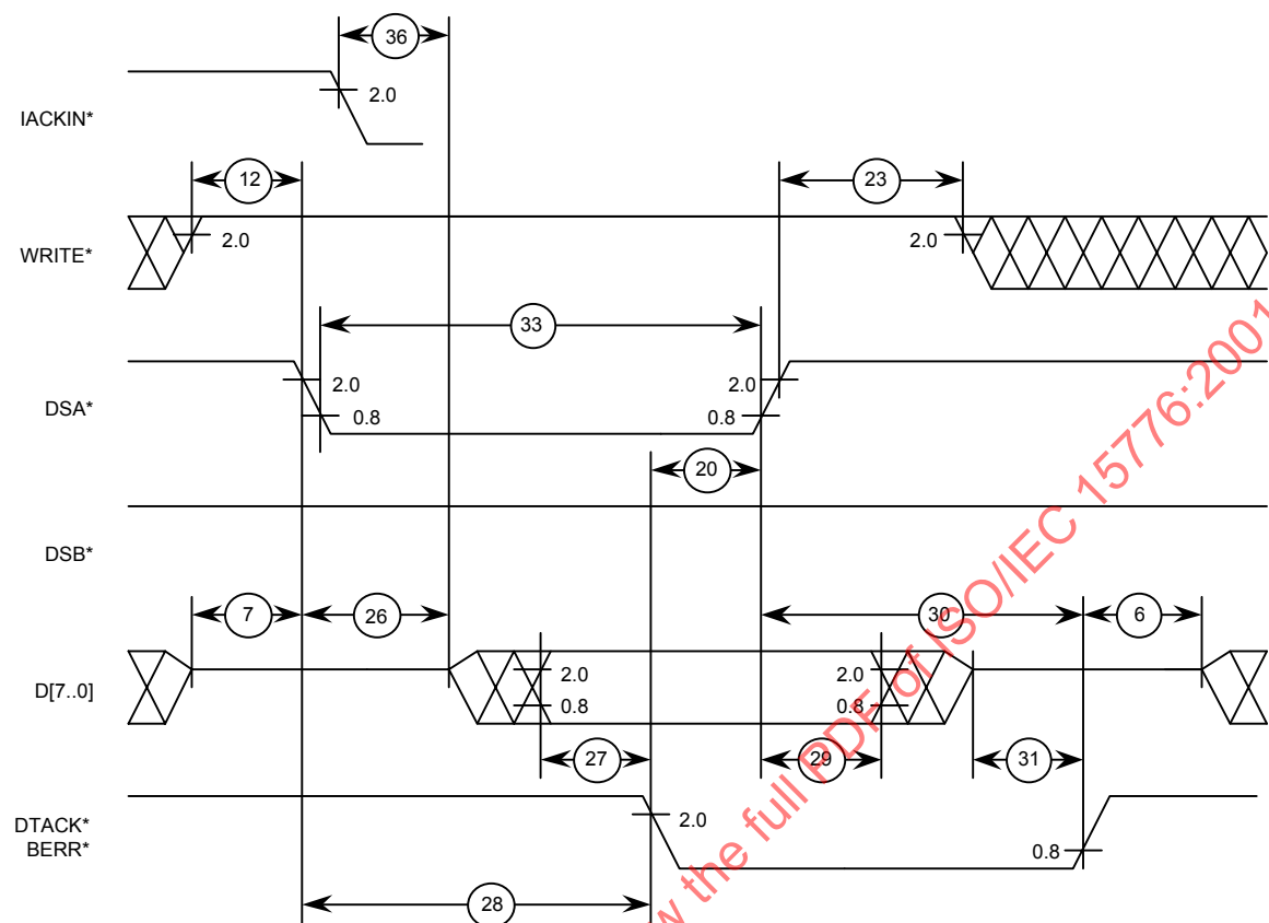
Figure 68 – Responding interrupter – Status/ID transfer timing single-byte interrupt acknowledge cycle
