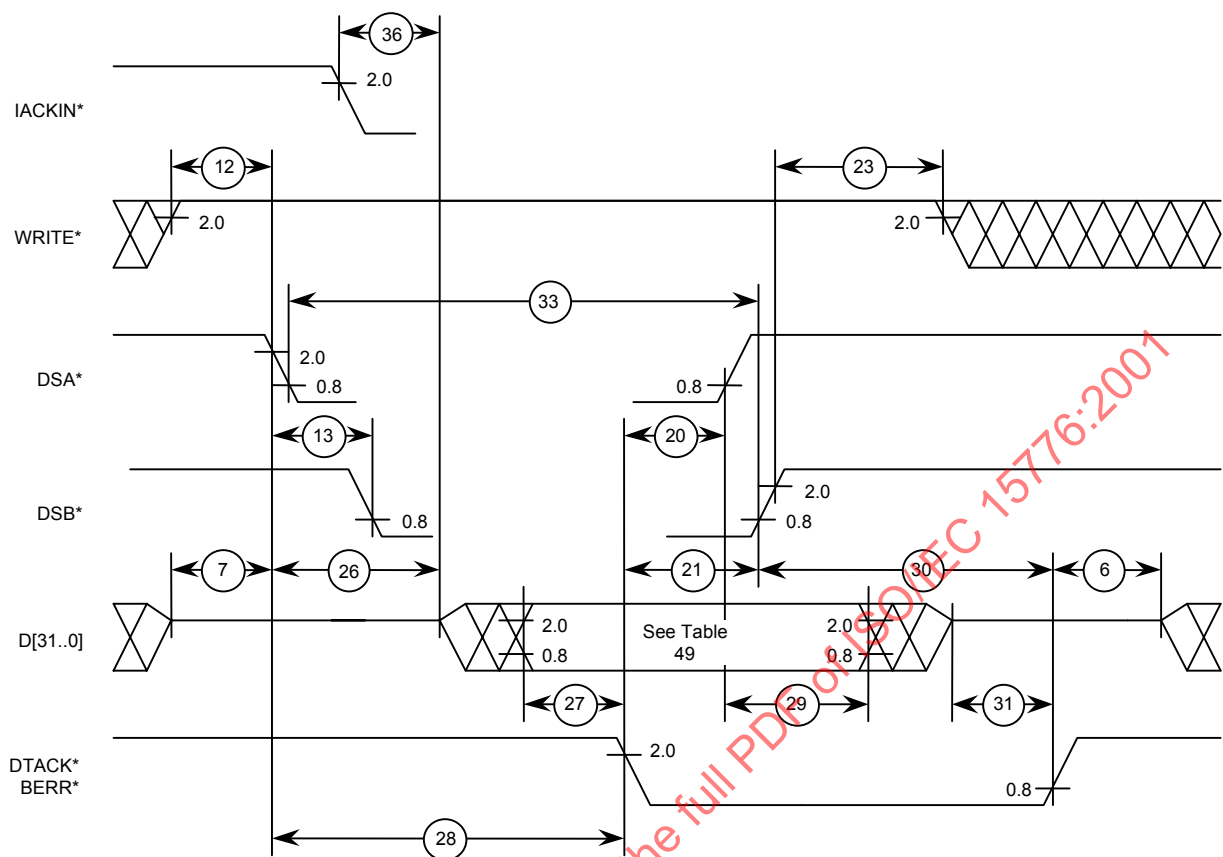
Figure 69 – Responding interrupter – Status/ID transfer timing double-byte interrupt acknowledge cycle quad-byte interrupt acknowledge cycle
