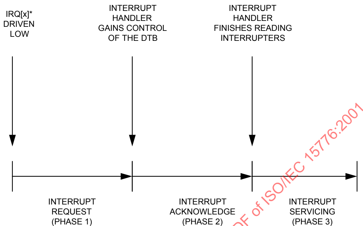
Figure 57 – The three phases of an interrupt sequence
