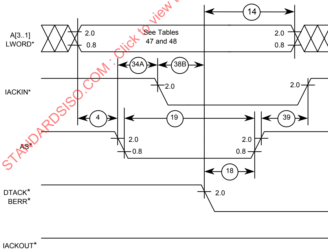
Figure 65 – Responding interrupter – Interrupter selection timing single-byte, double-byte, and quad-byte interrupt acknowledge cycles
