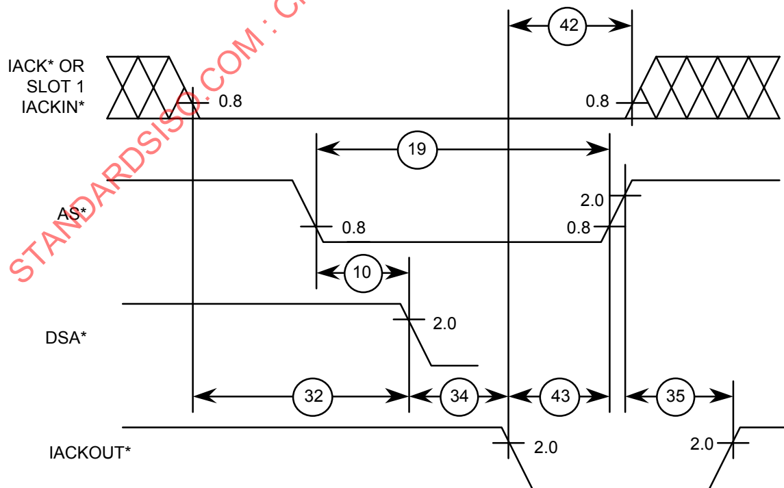
Figure 63 – IACK daisy-chain driver – Interrupter selection timing single-byte, double-byte, and quad-byte interrupt acknowledge cycles
