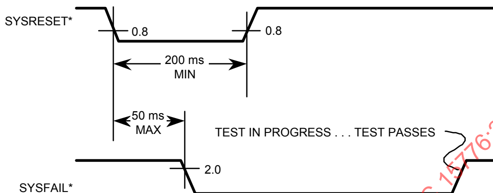
Figure 76 – SYSRESET* and SYSFAIL* timing diagram
