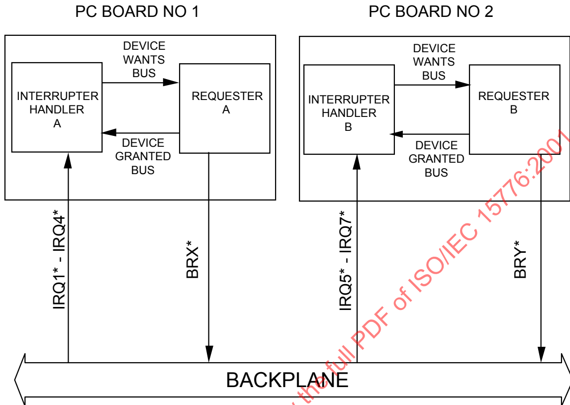
Figure 59 – Two interrupt handlers, each monitoring several interrupt request lines
