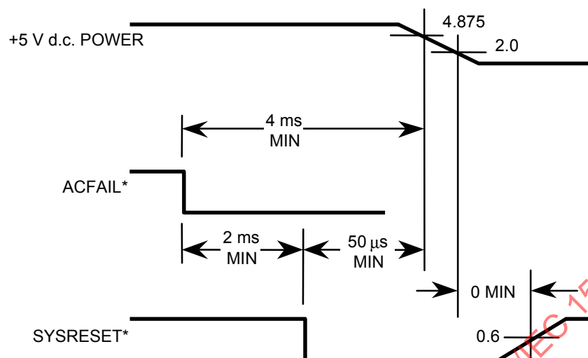
Figure 74 – Power monitor power failure timing
