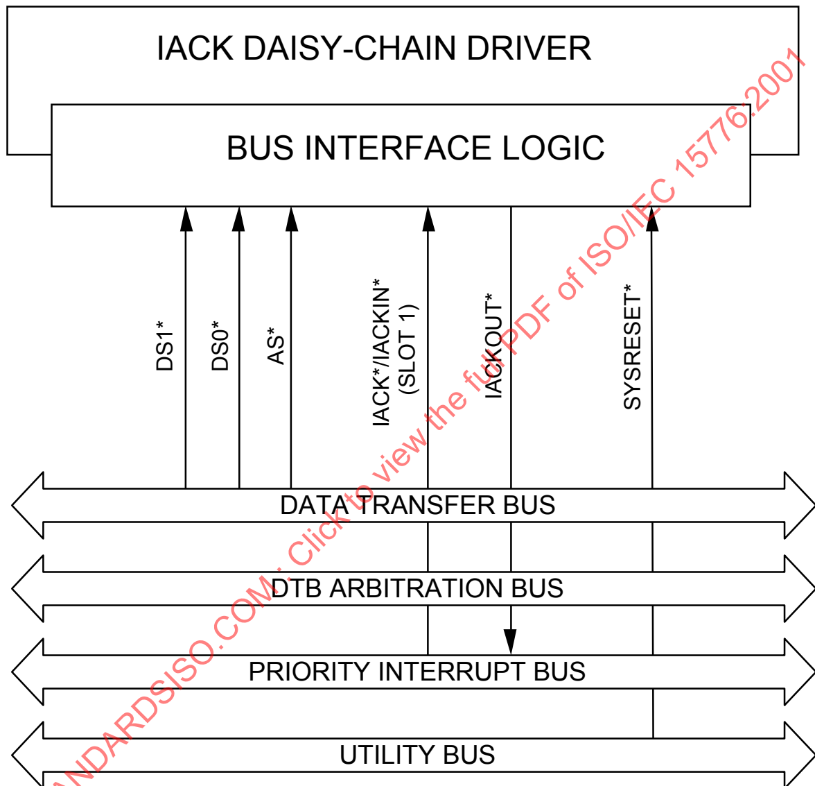
Figure 53 – Block diagram – IACK daisy-chain driver
