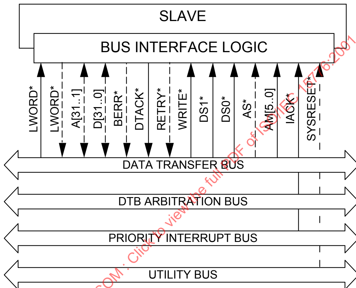
Figure 6 – Block diagram – Slave
