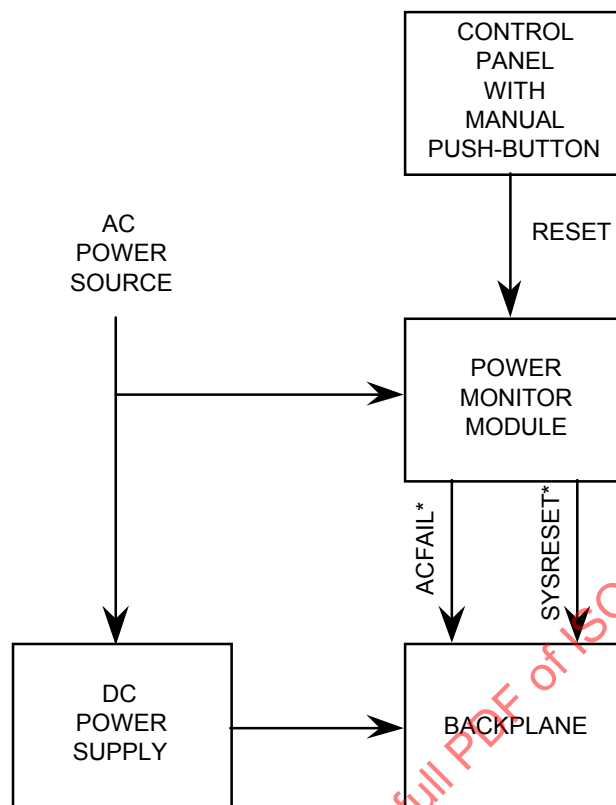
Figure 73 – Block diagram of power monitor module
