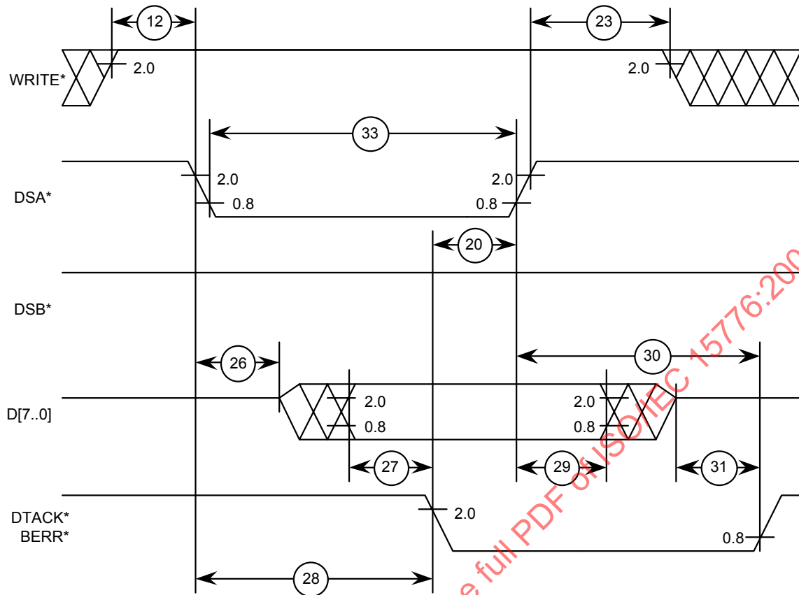
Figure 66 – Interrupt handler – Status/ID transfer timing single-byte interrupt acknowledge cycle
