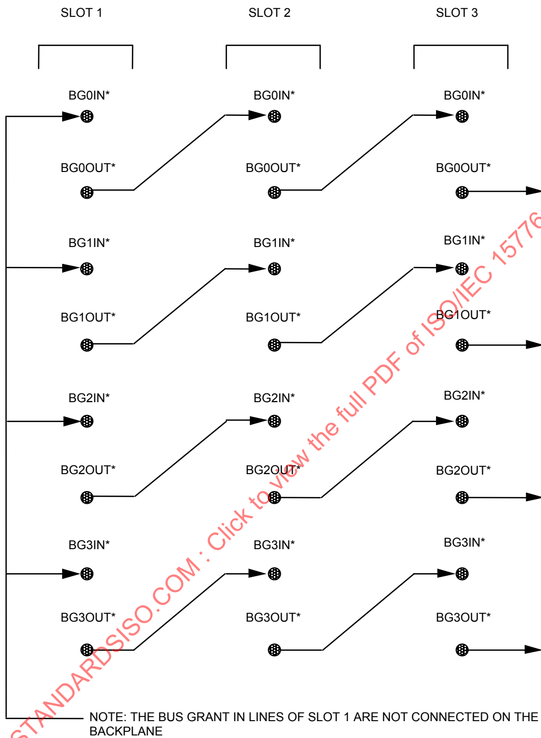
Figure 40 – Illustration of the daisy chain bus grant lines
