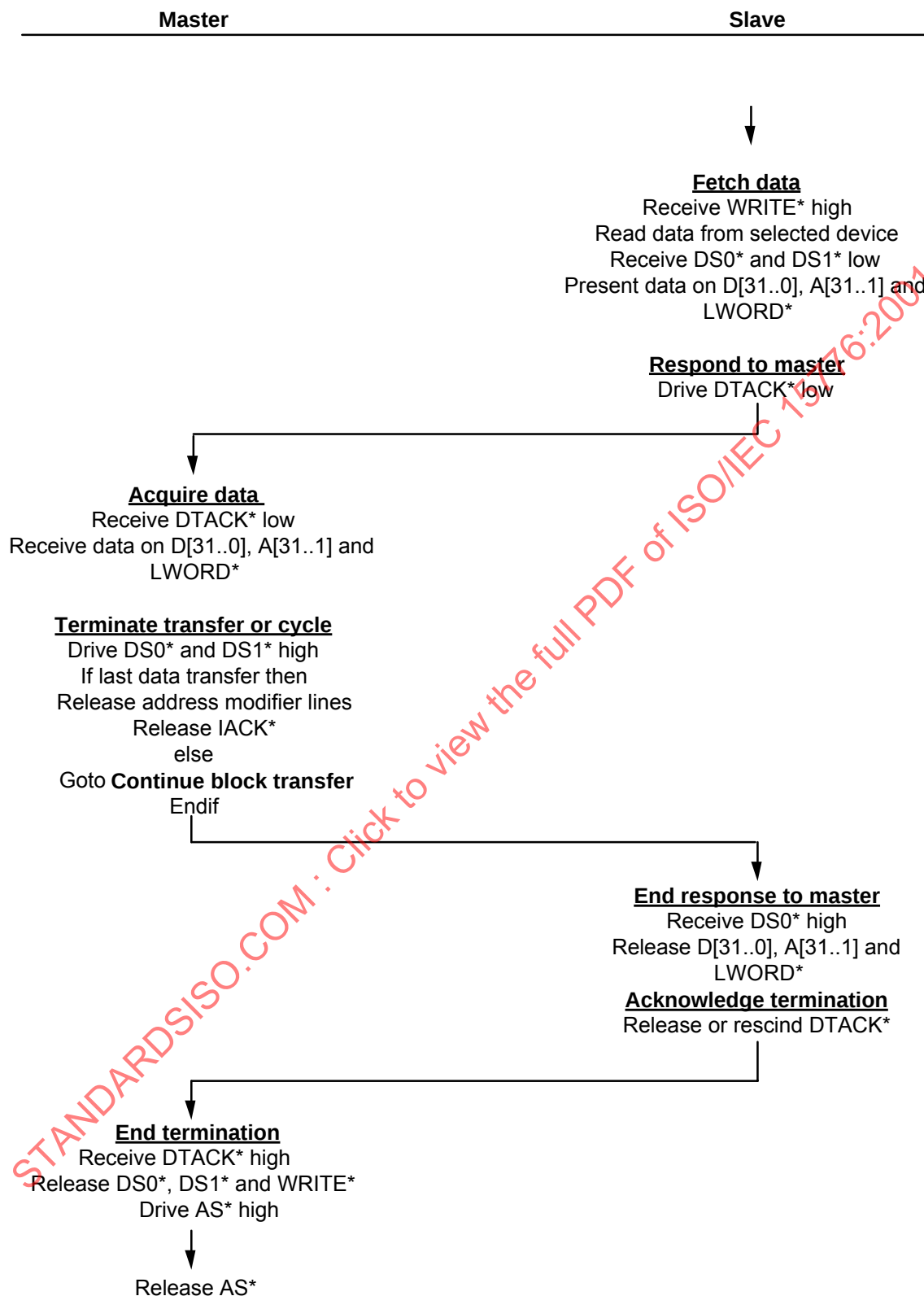
Figure 15 – Example of eight-byte block read cycle (continued)
