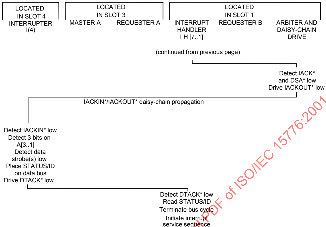
Figure 60 – Typical single handler interrupt system operation flow diagram (continued)
