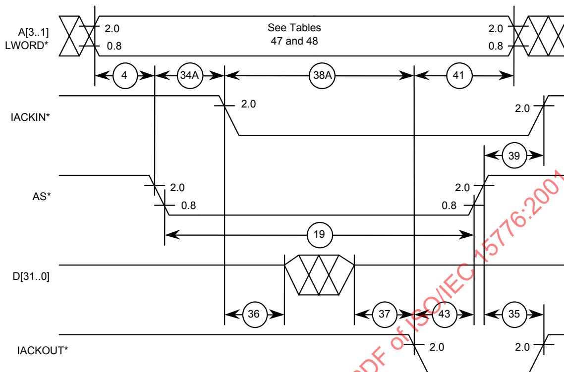
Figure 64 – Participating interrupter – Interrupter selection timing single-byte, double-byte, and quad-byte interrupt acknowledge cycles
