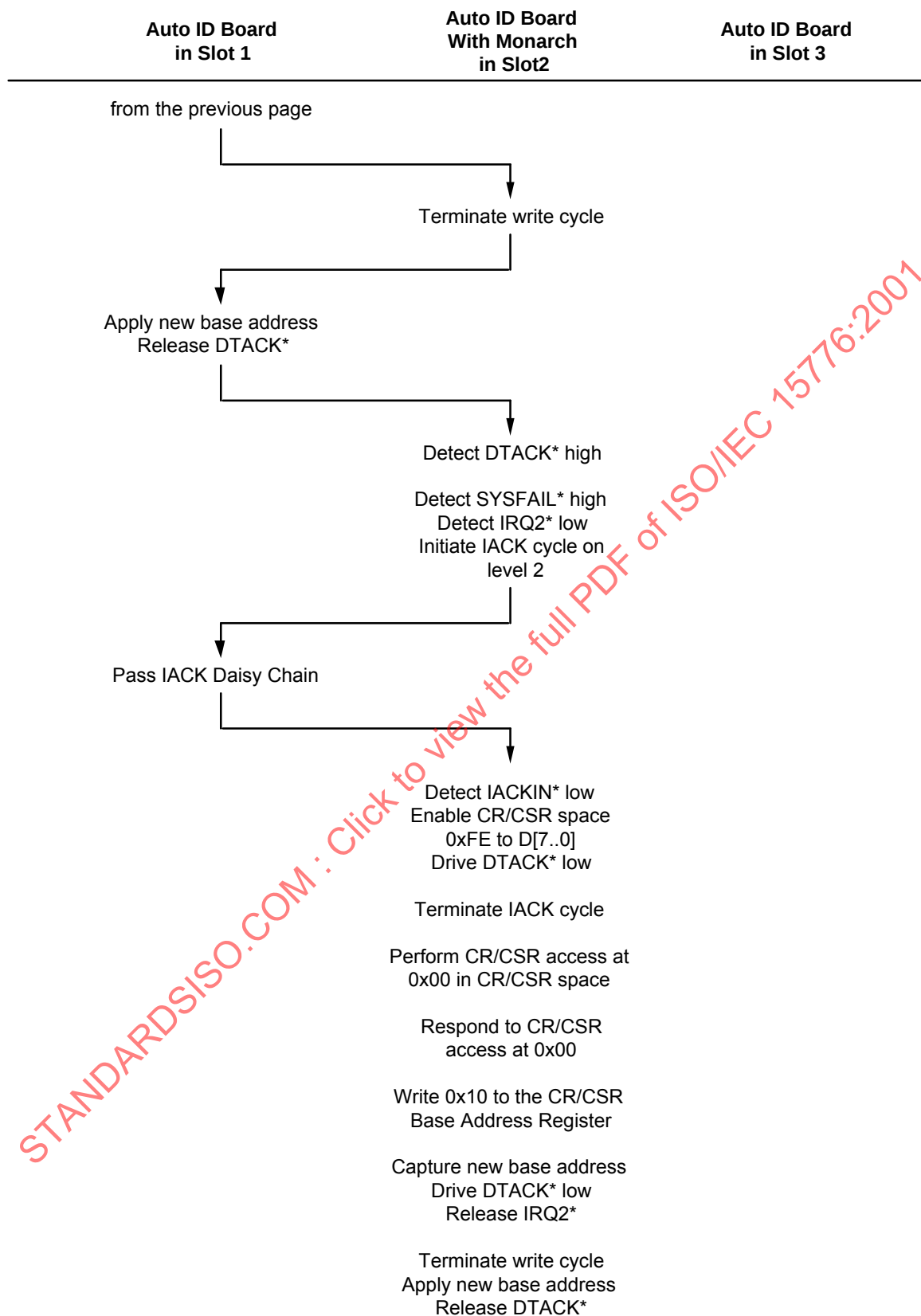
Figure 78 – CR/CSR auto ID slave initialization algorithm (continued)
