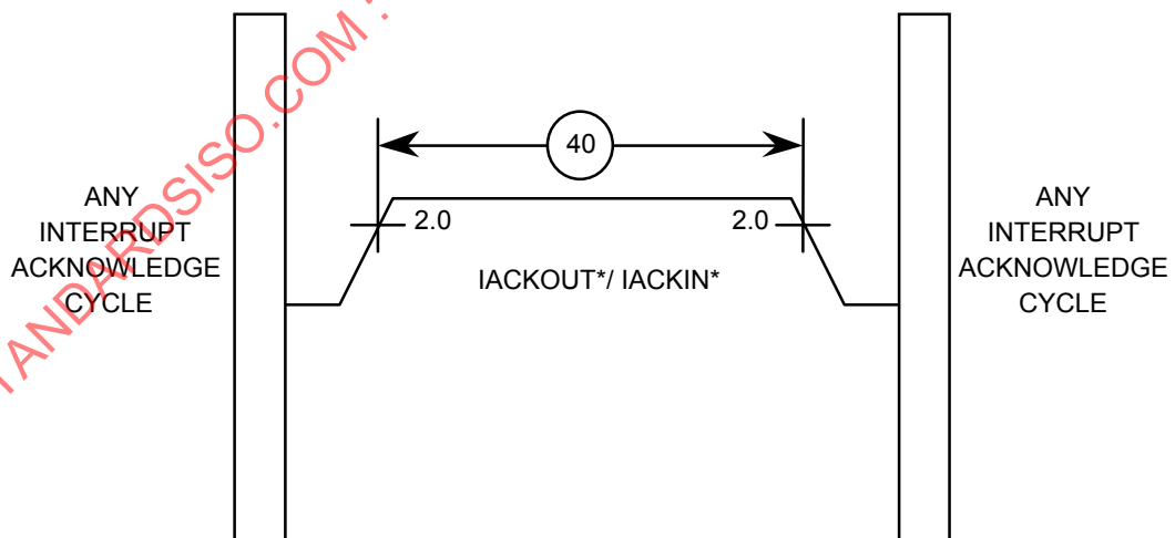
Figure 70 – IACK daisy-chain driver, responding interrupter, and participating interrupter IACK daisy-chain inter-cycle timing
