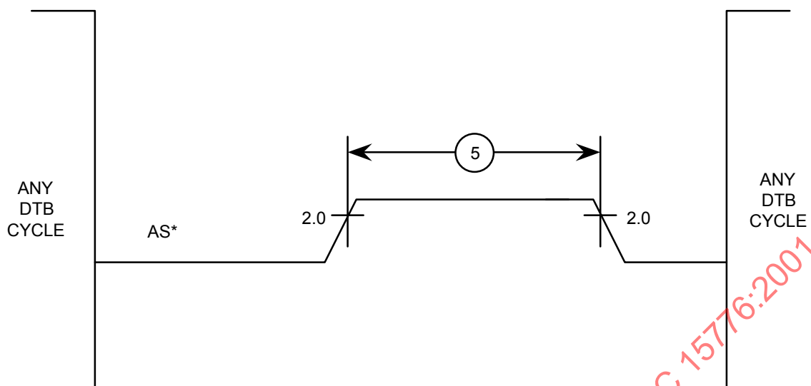
Figure 30 – Address strobe inter-cycle timing
