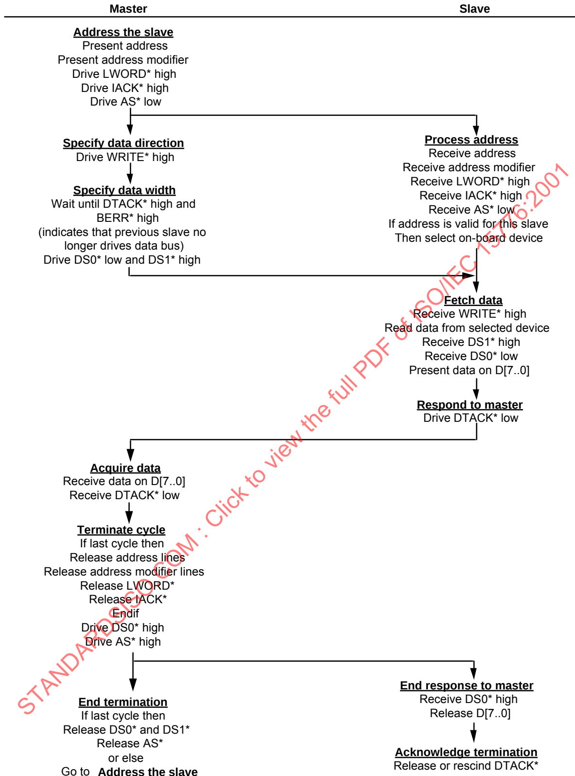
Figure 12 – Example of non-multiplexed address single-byte read cycle
