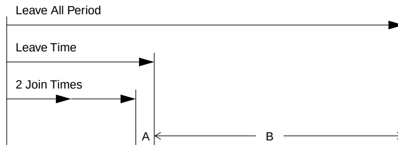
Figure 12-7—GARP timing relationships
