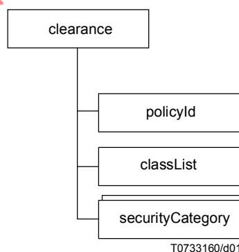
Figure 1 – Clearance Attributes Structure
