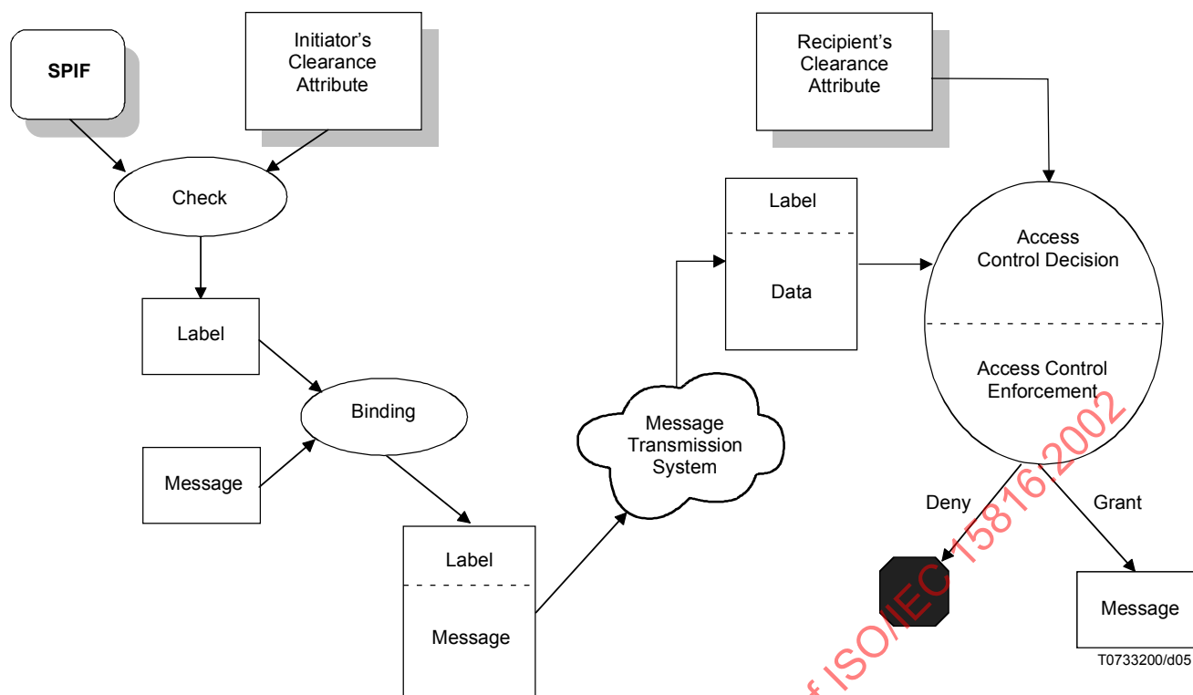
Figure 5 – Messaging Scenario Access Control
