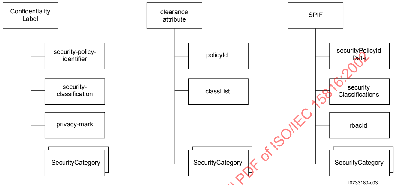
Figure 3 – Equivalent Object Class Comparison
