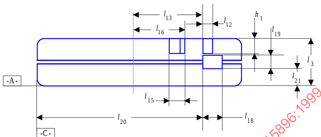
Figure 9 - Right side
