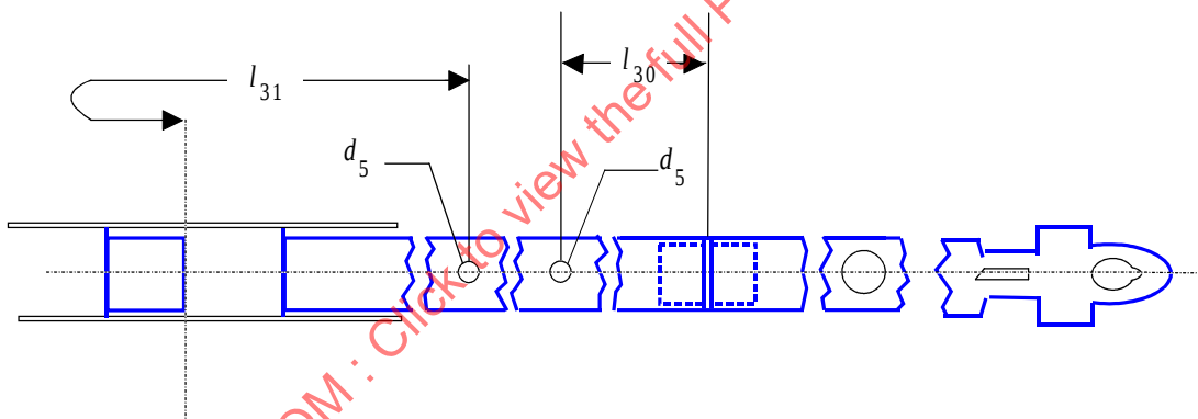
Figure 14 - Leader/tape connection
