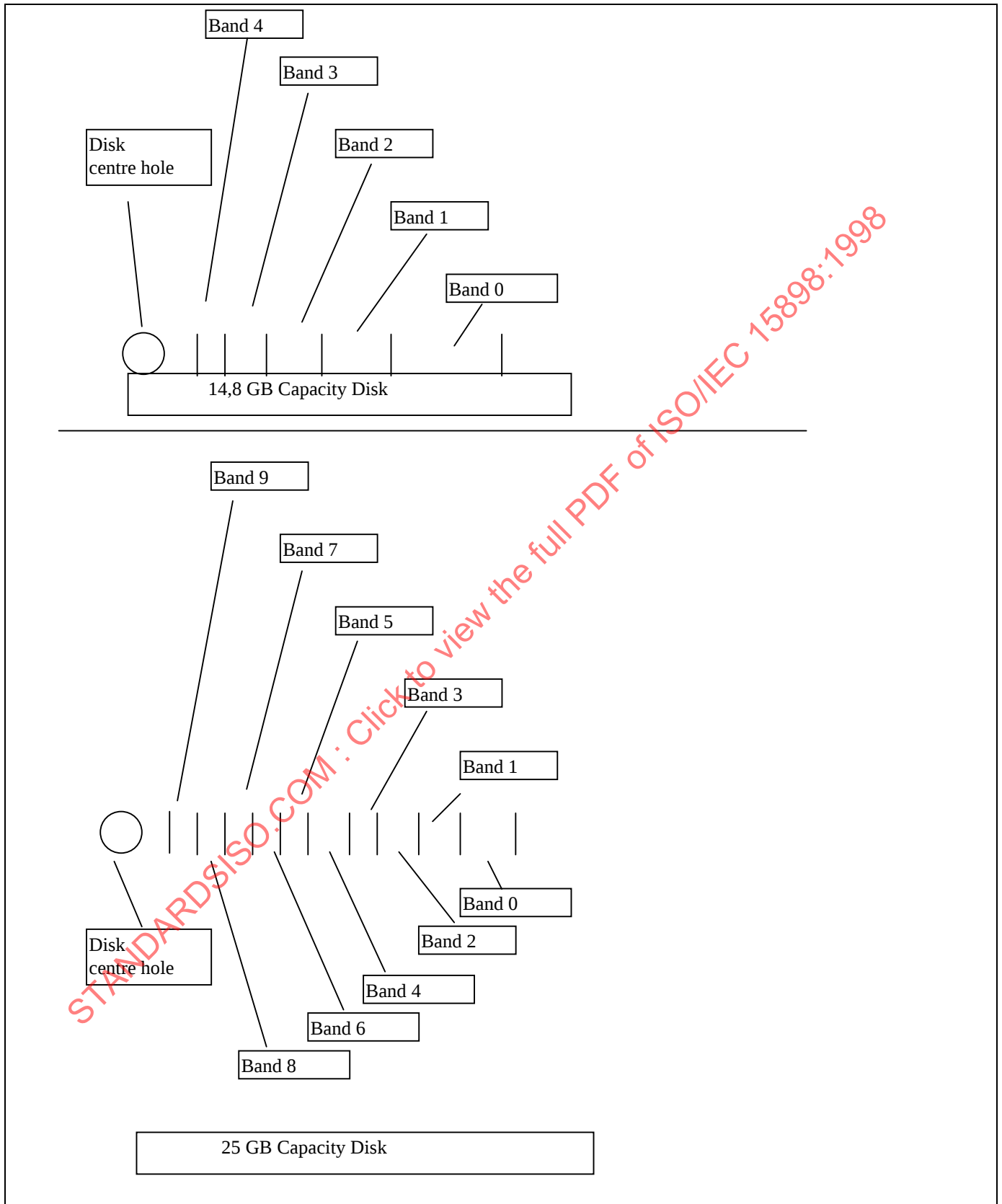
Figure 27 - Band organization
