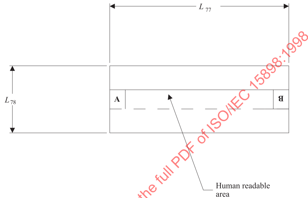
Figure 23 - Main elements of the optical disk
