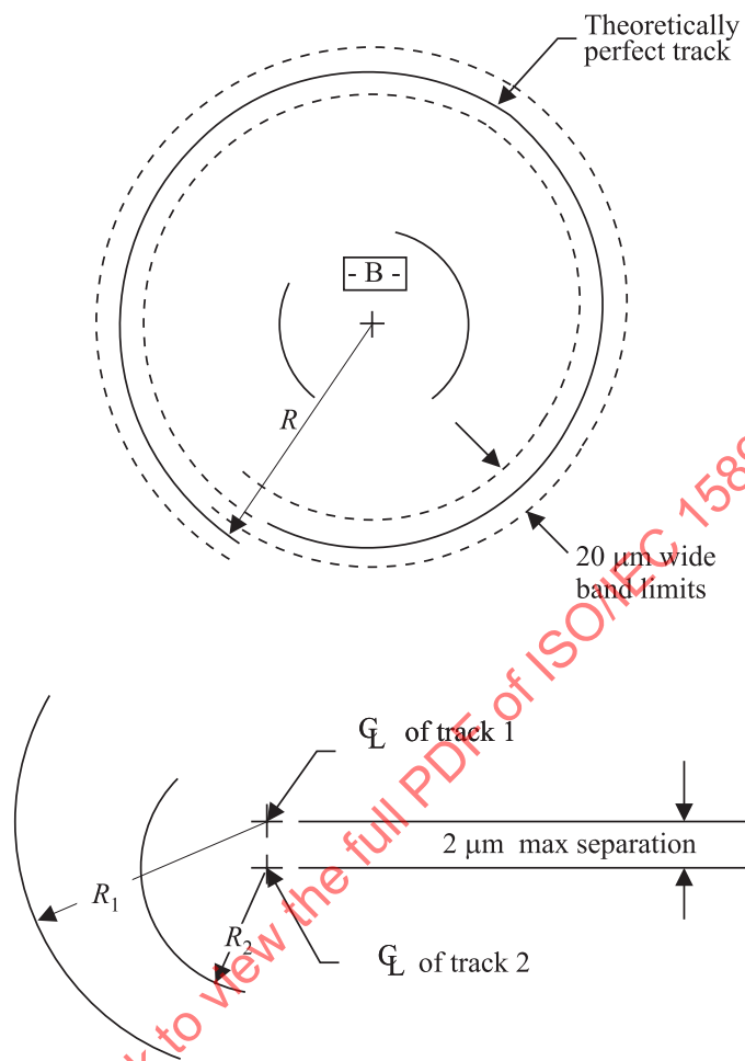
Figure 28 - Track concentricity
