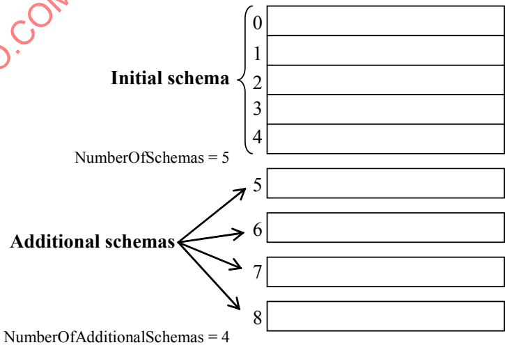
Figure AMD1-2 - Addressing the initial schema and the additional schemas
